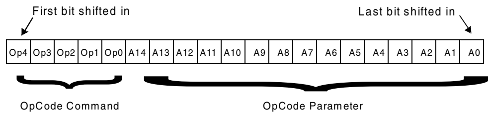
Figure 5 OpCode Format
