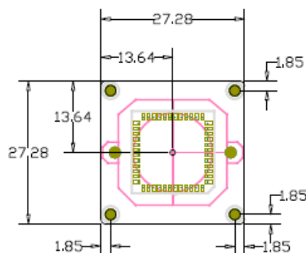
Sensor board
