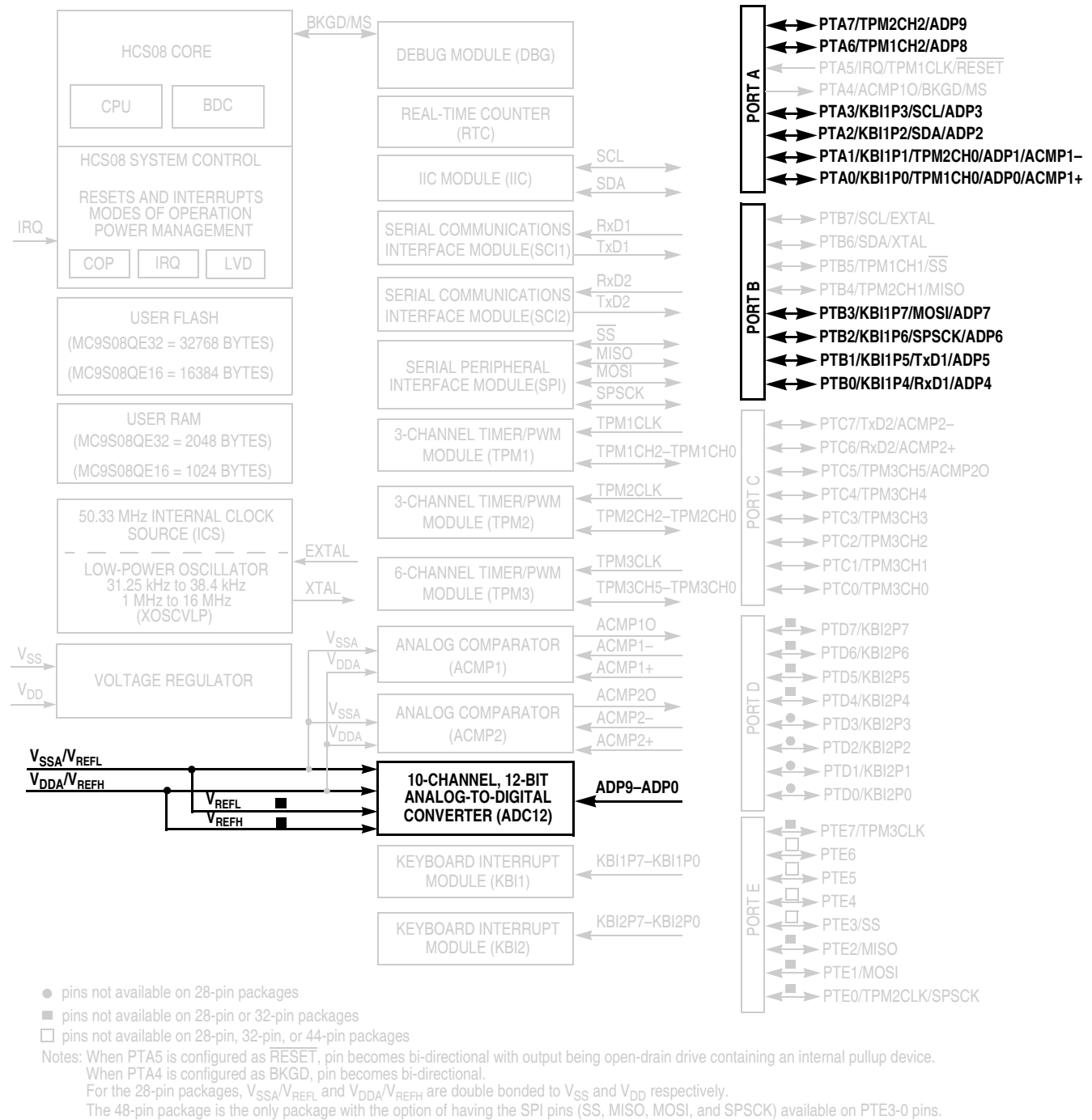
Figure 10-1. MC9S08QE32 Series Block Diagram Highlighting ADC Module and Pins
