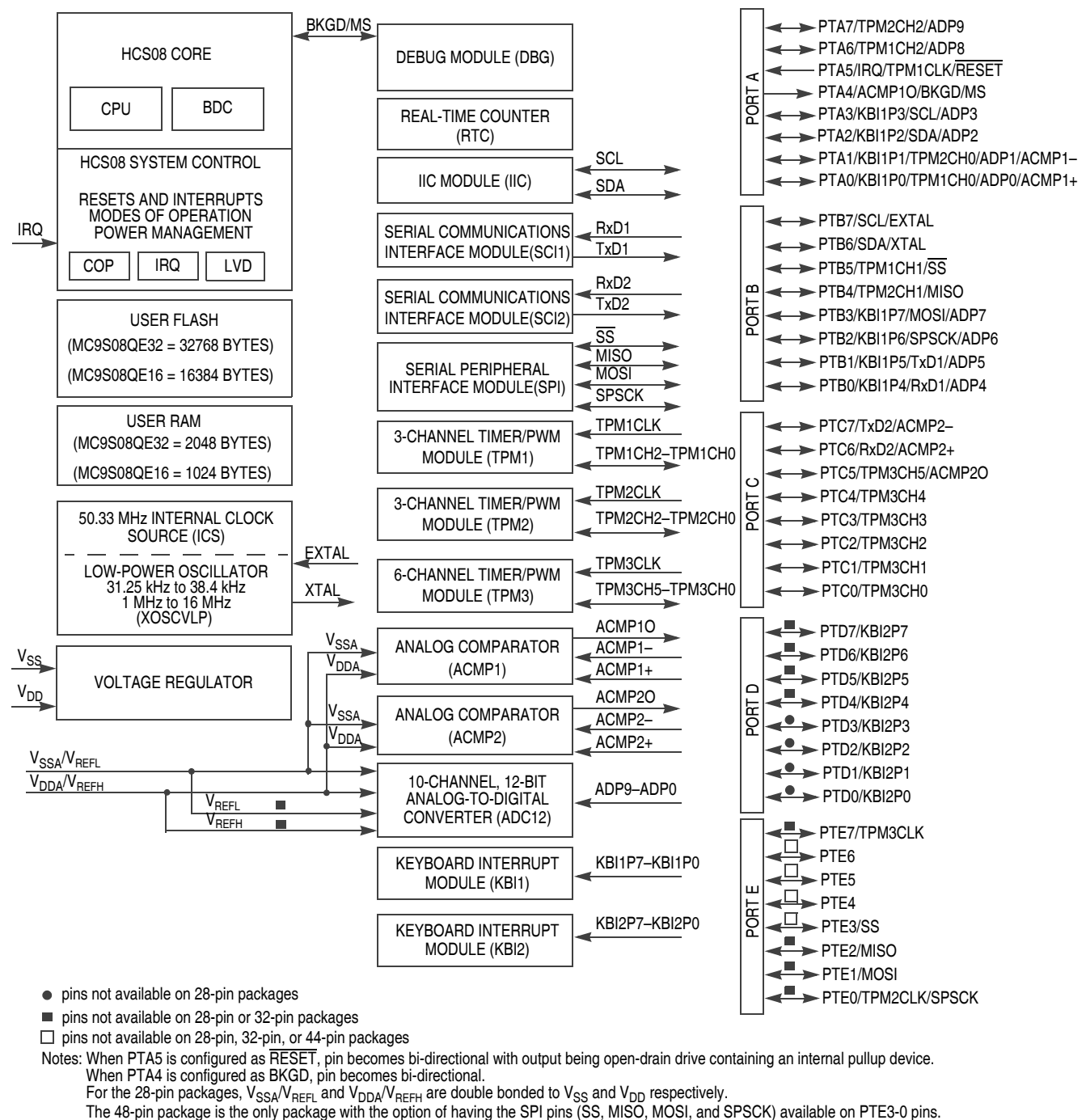
Figure 1-1. MC9S08QE32 Series Block Diagram
