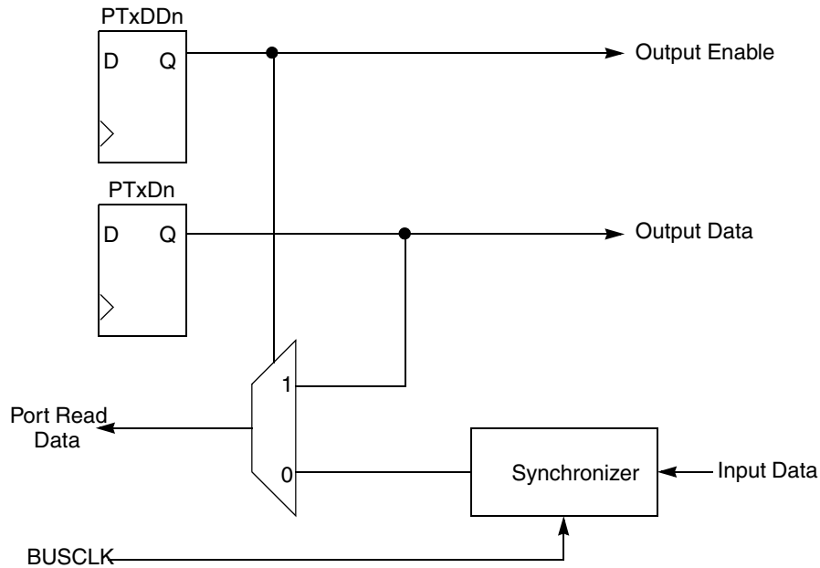
Figure 6-1. Parallel I/O Block Diagram
