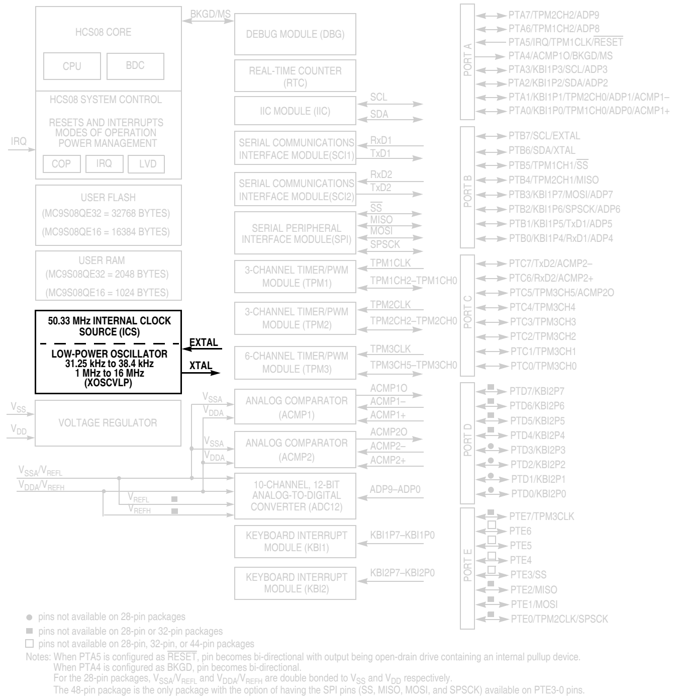
Figure 11-1. MC9S08QE32 Series Block Diagram Highlighting ICS Module and Pins
