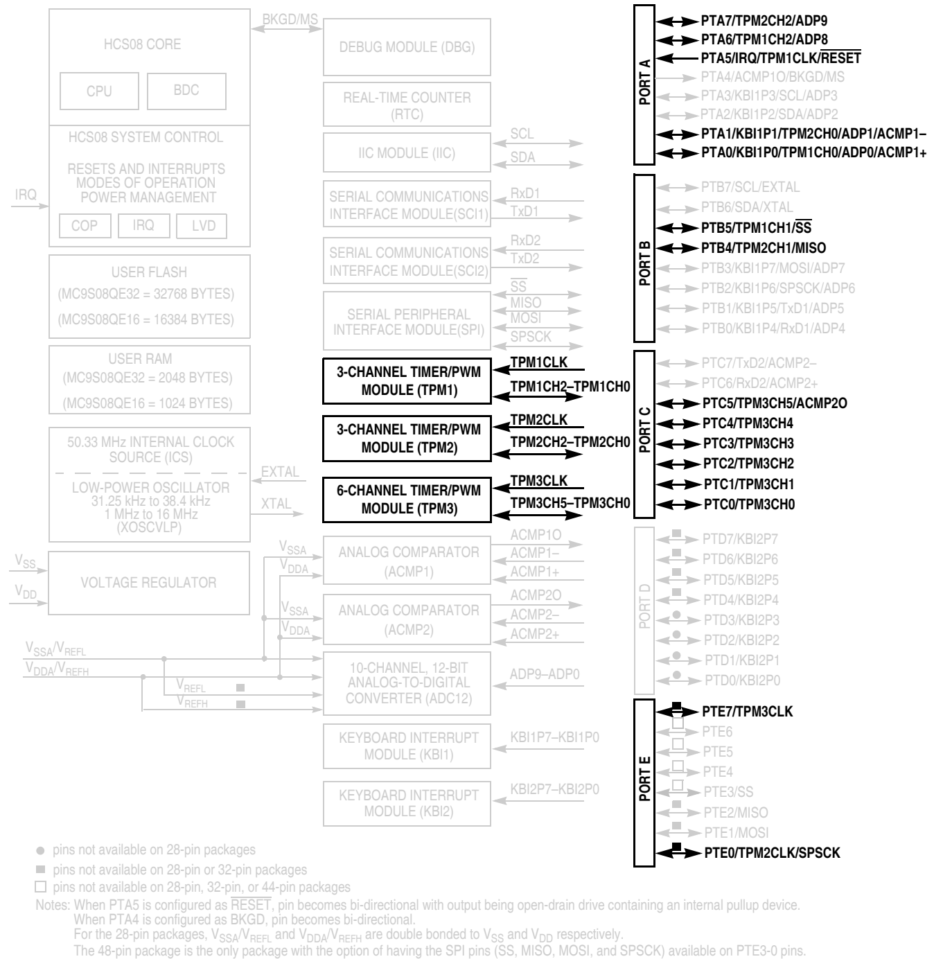
Figure 16-1. MC9S08QE32 Series Block Diagram Highlighting TPM Modules and Pins
