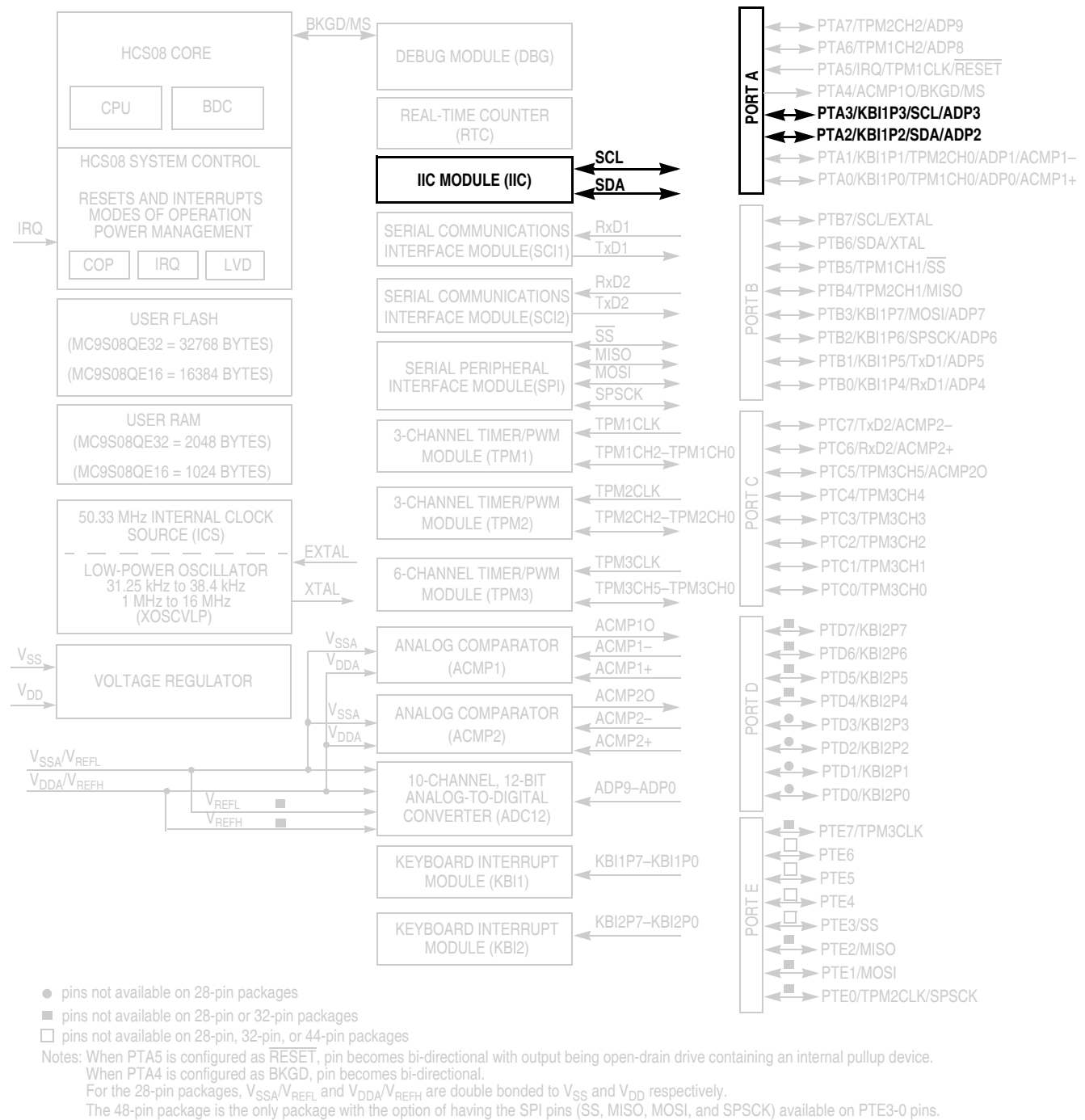
Figure 12-1. MC9S08QE32 Series Block Diagram Highlighting IIC Module and Pins
