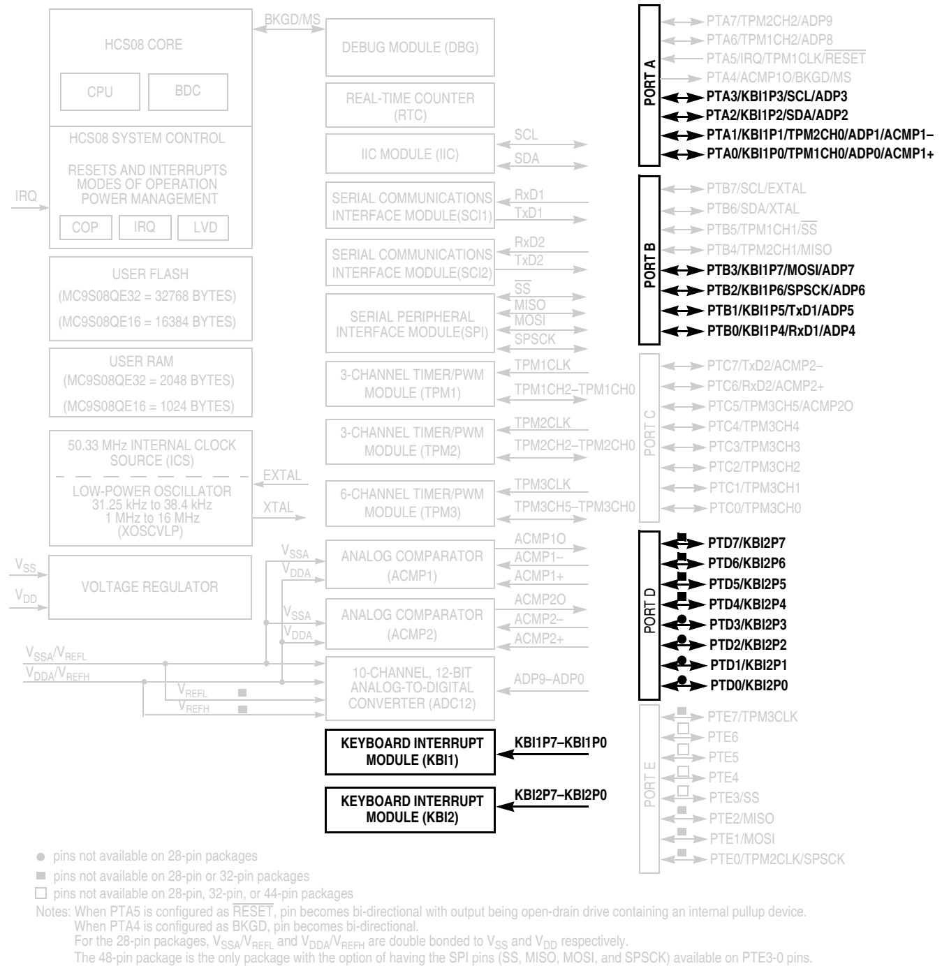
Figure 7-1. MC9S08QE32 Series Block Diagram Highlighting KBI Modules and Pins
