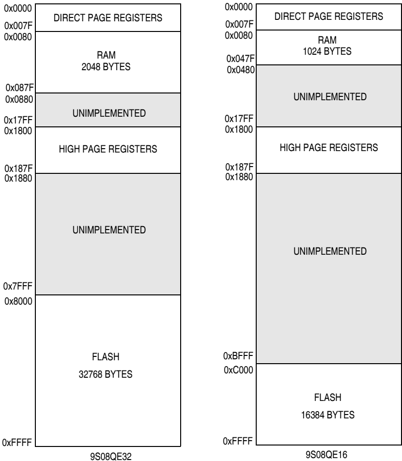
Figure 4-1. MC9S08QE32 Series Memory Maps
