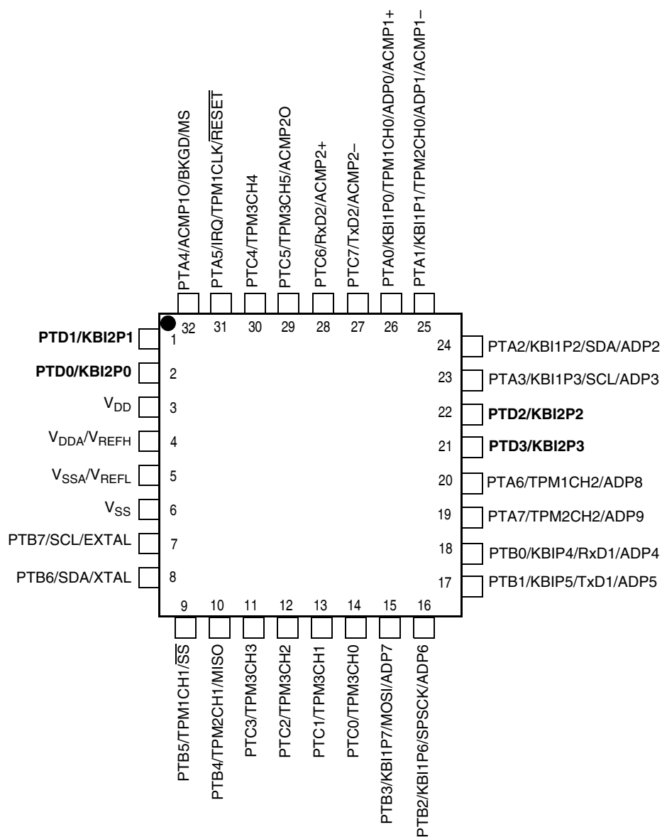
Figure 2-3. 32-Pin LQFP
