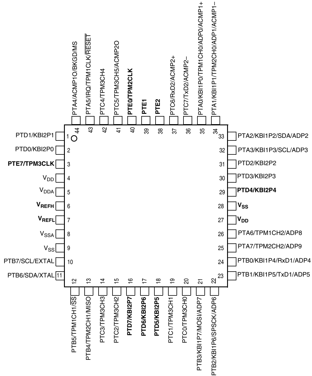
Figure 2-2. 44-Pin LQFP
