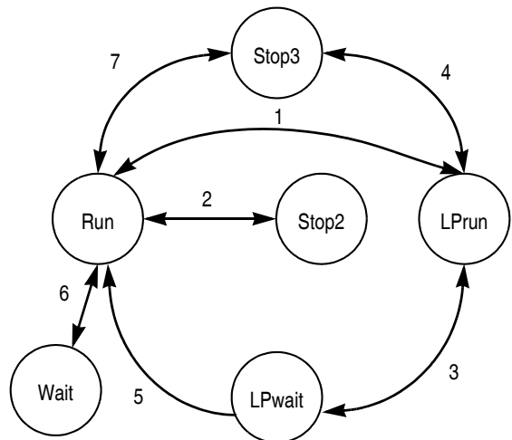
Figure 3-1. Allowable Power Mode Transitions for the MC9S08QE32 Series
