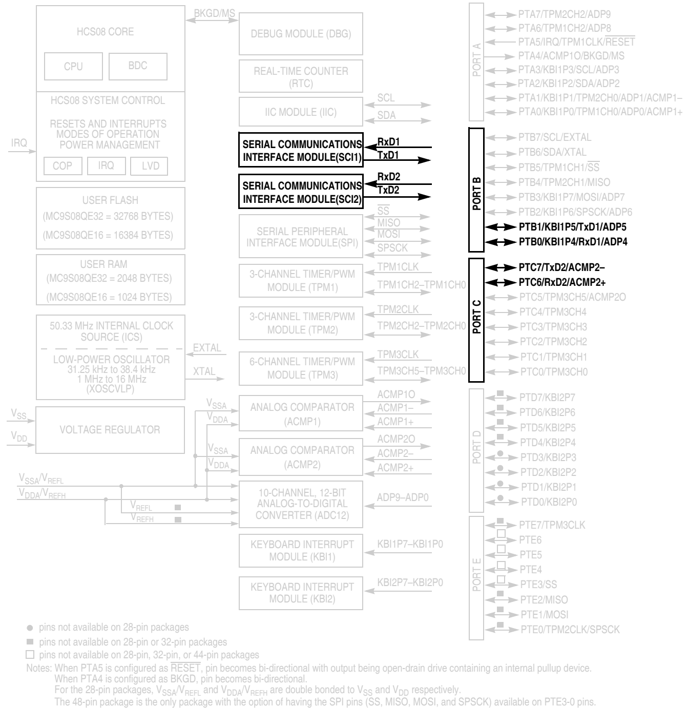
Figure 14-1. MC9S08QE32 Series Block Diagram Highlighting SCI Modules and Pins
