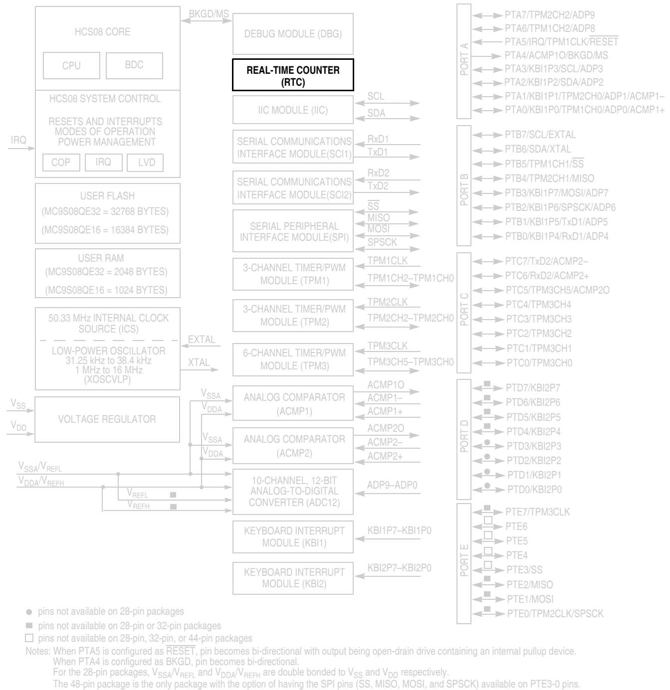
Figure 13-1. MC9S08QE32 Series Block Diagram Highlighting RTC Module
