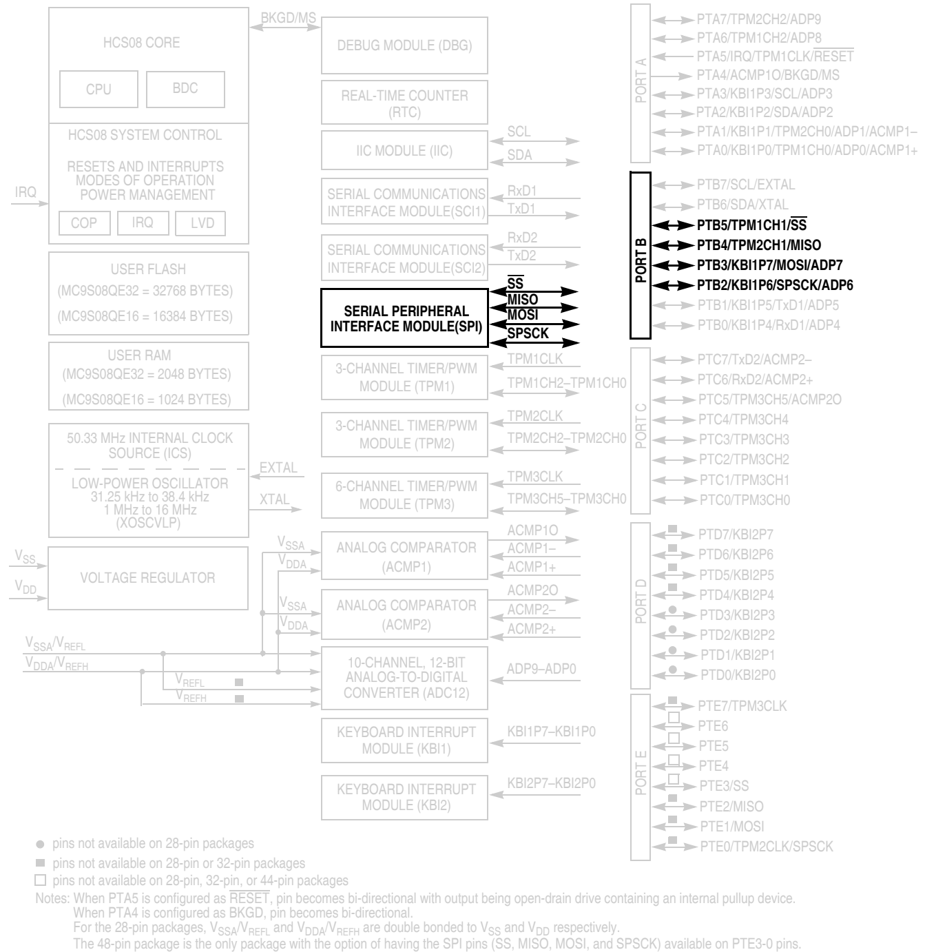
Figure 15-1. MC9S08QE32 Block Diagram Highlighting SPI Module and Pins
