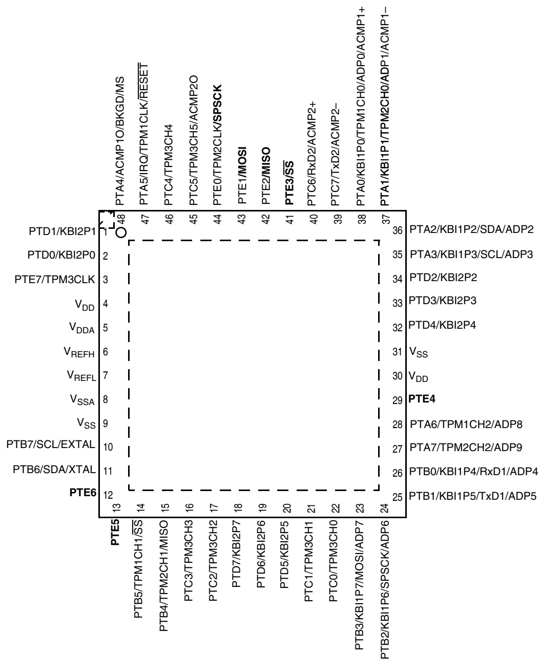
Figure 2-1. 48-Pin QFN
