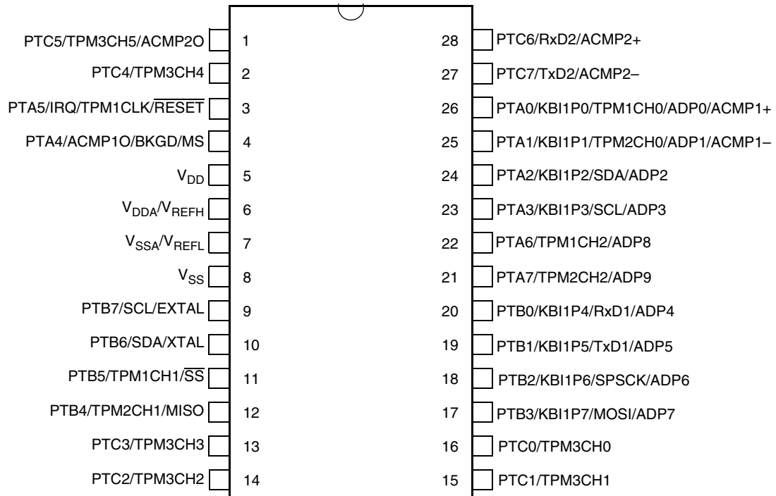
Figure 2-4. 28-Pin SOIC
