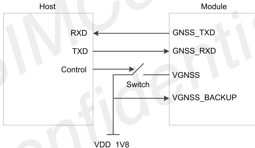
Figure 36: GNSS Circuit Diagram (NMEA to host UART)
