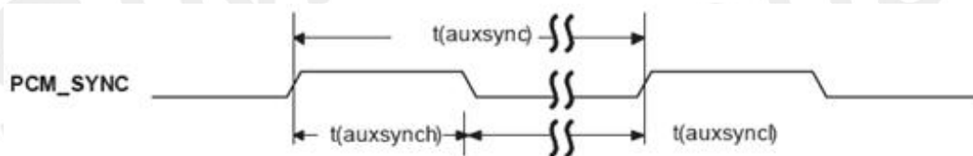
Figure 28: PCM_SYNC Timing
