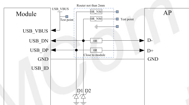
Figure 19: USB Reference Circuit
