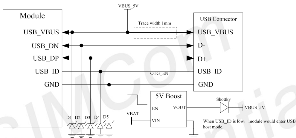
Figure 22: USB_OTG Diagram
