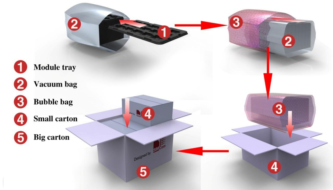
Figure 45: Packaging Diagram
