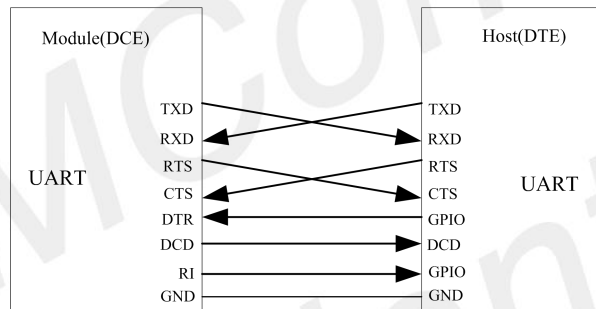
Figure 13: UART Full Modem
