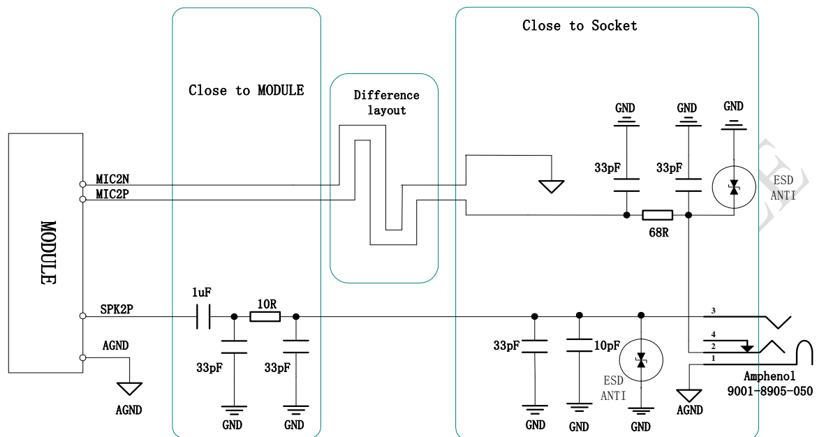
Figure 25: Earphone interface configuration
