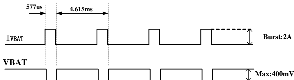
Figure 5: VBAT voltage drop during transmit burst
