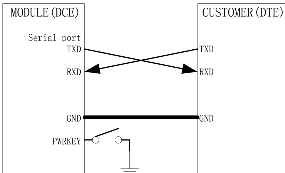
Figure 13: Connection of software upgrade
