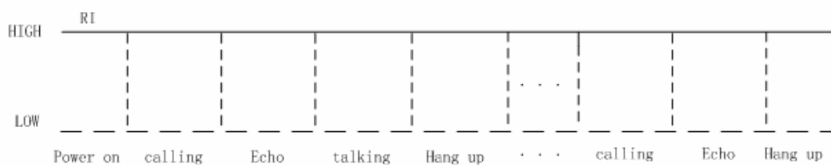
Figure 32: SIM340C Services as caller
