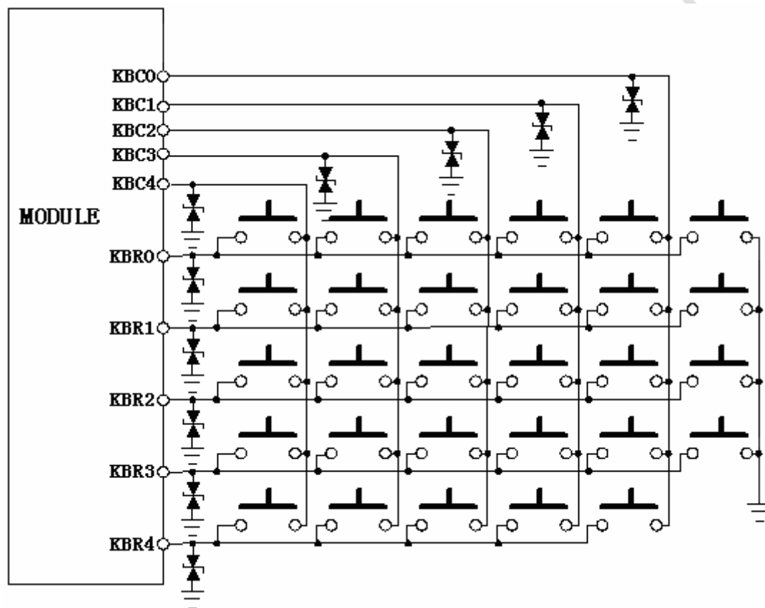
Figure 16: Reference circuit of the keypad interface
