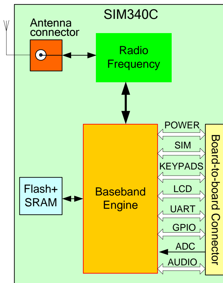
Figure 2: SIM340C functional diagram
