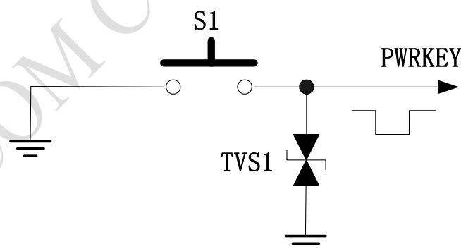
Figure 7: Turn on SIM340C using button
