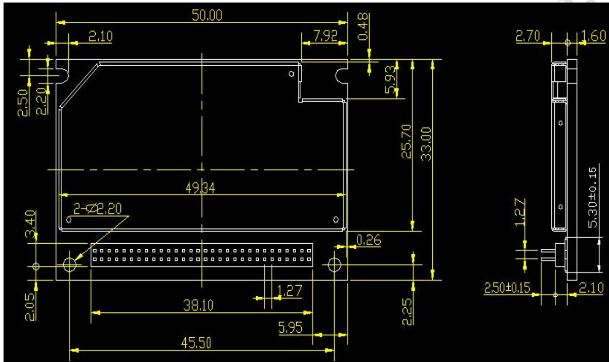
Figure 17: Mechanical dimensions of SIM340C (Unit: mm)
