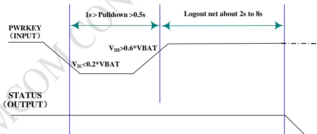
Figure 8: Timing of turn off system
