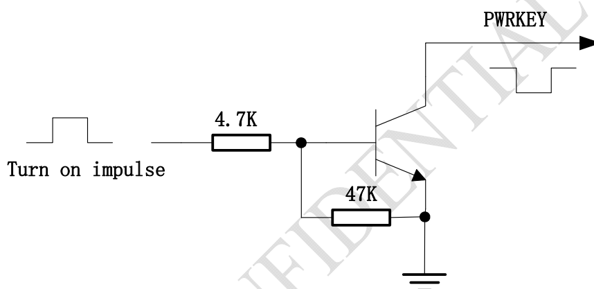
Figure 6: Turn on SIM340C using driving circuit
