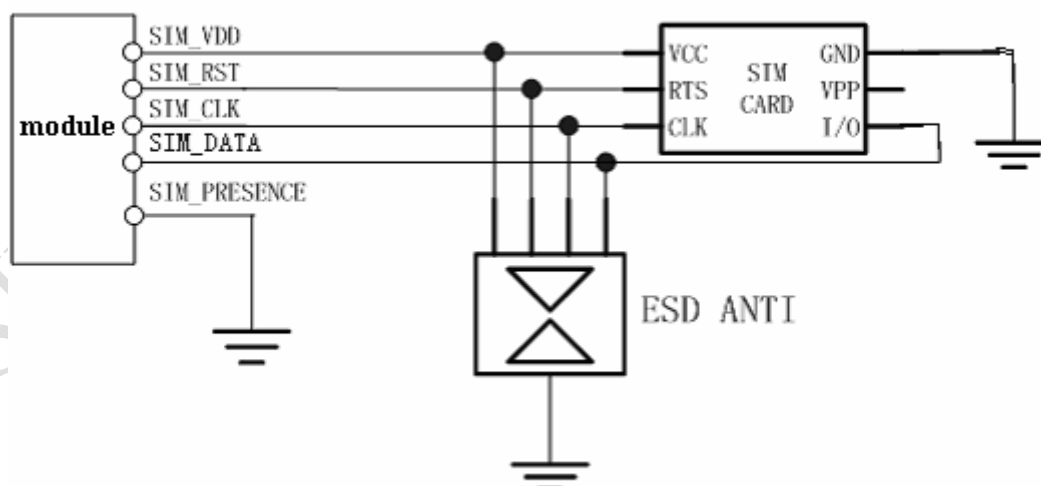
Figure 28: Reference circuit of the 6 pins SIM card holder
