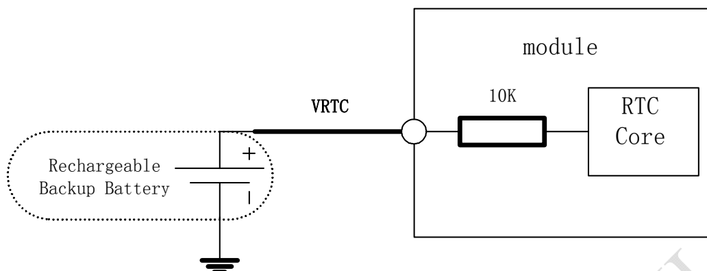
Figure13: RTC supply from rechargeable battery
