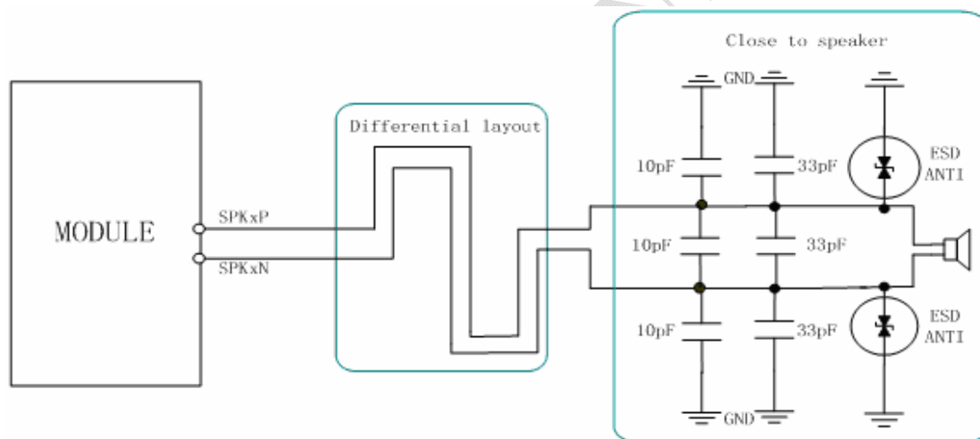
Figure 22: Speaker interface configuration
