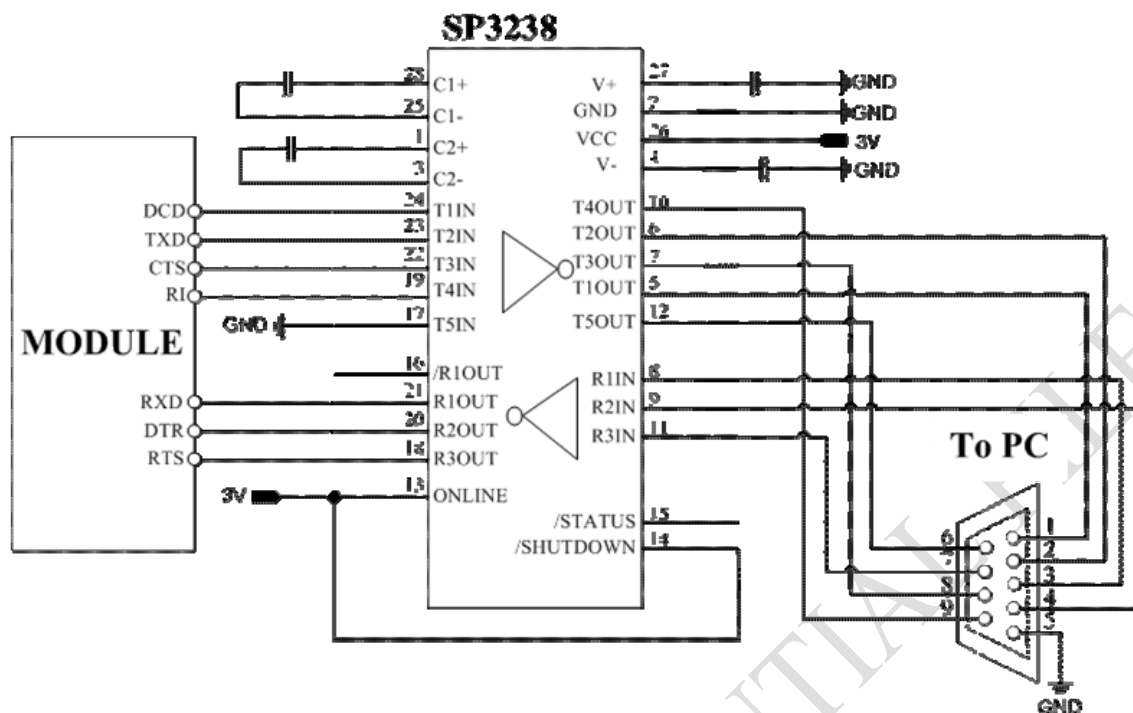
Figure 14: RS232 level converter circuit
