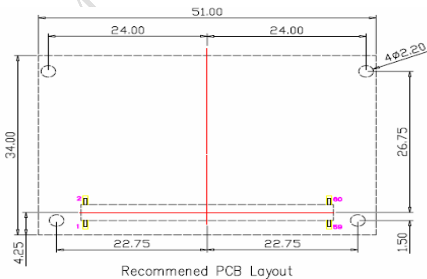
Figure 18: Recommended PCB Layout (Unit: mm)
