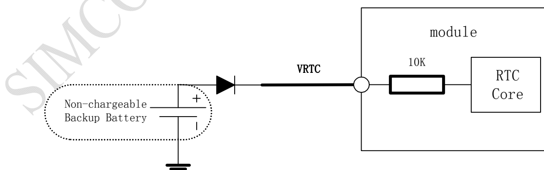
Figure12: RTC supply from non-chargeable battery
