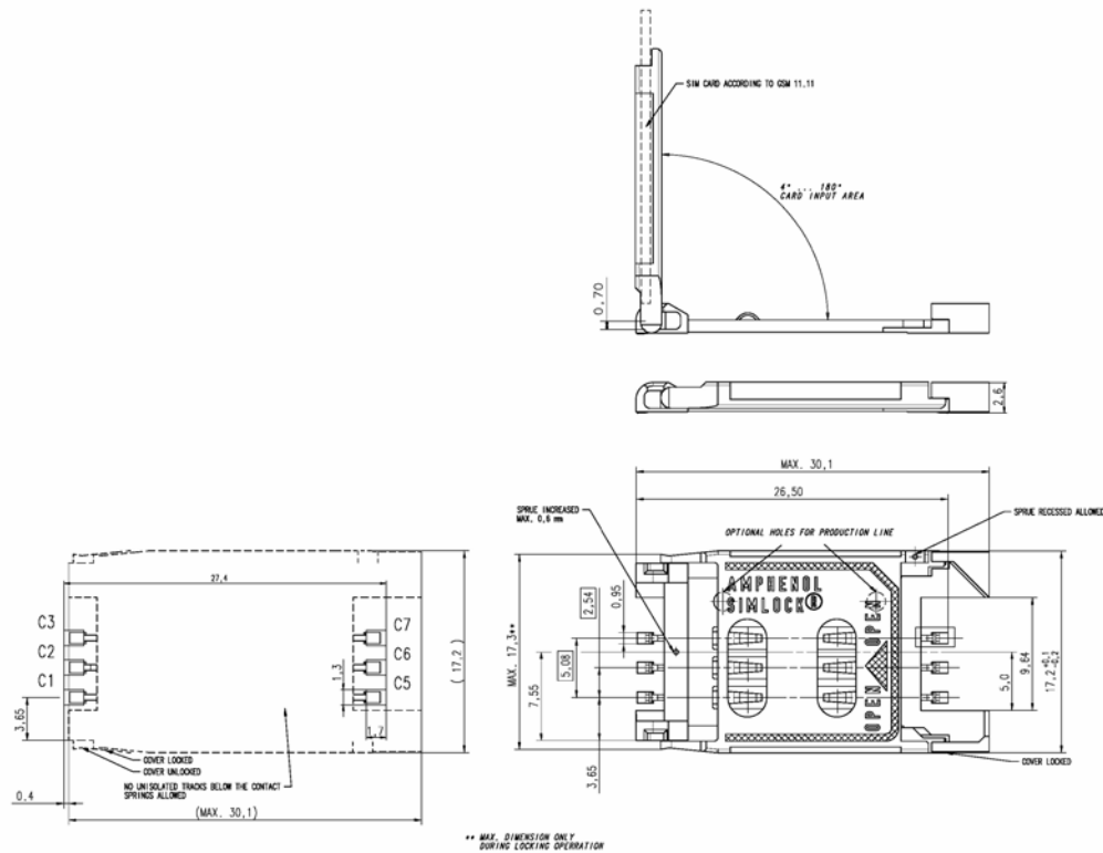
Figure 15: Amphenol C707 10M006 512 2 SIM card holder
