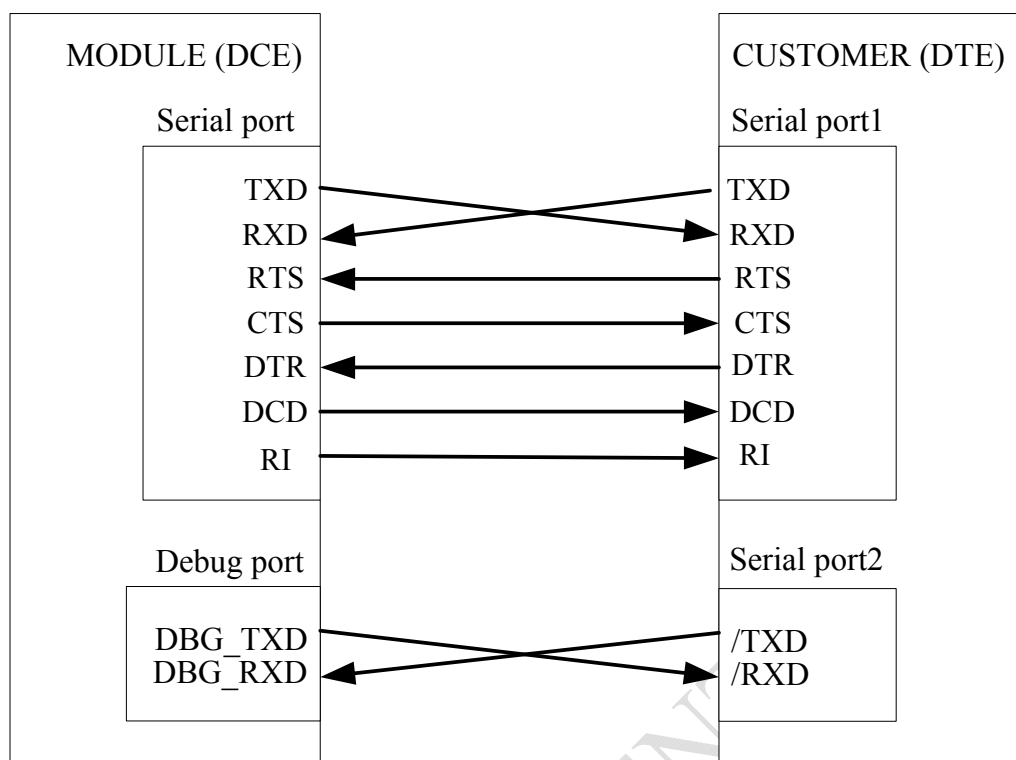
Figure 12: Connection of the serial interface
