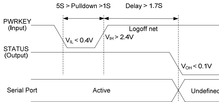
Figure 12: Timing of power down SIM900L by PWRKEY
