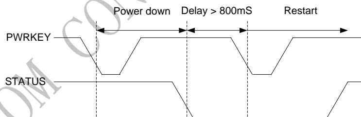
Figure 13: Timing of restart SIM900L
