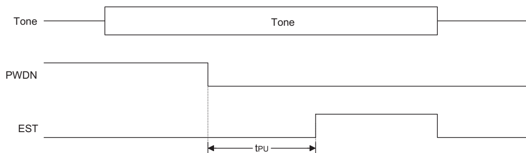
Figure 4. Power-up Timing
