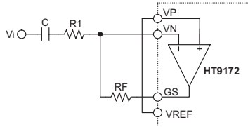
(b) Differential Input Circuit
