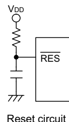
Reset circuit
