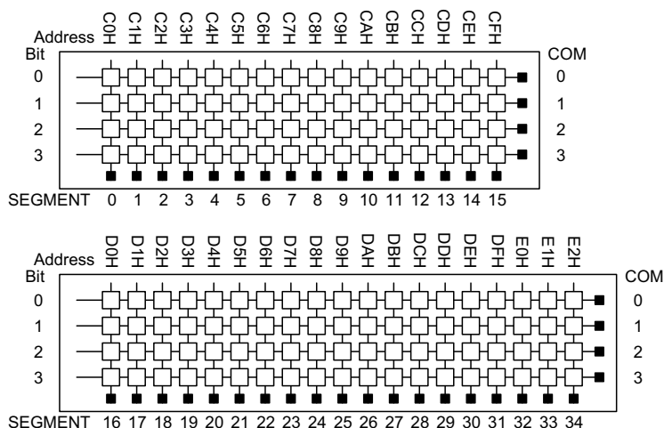
Display memory
