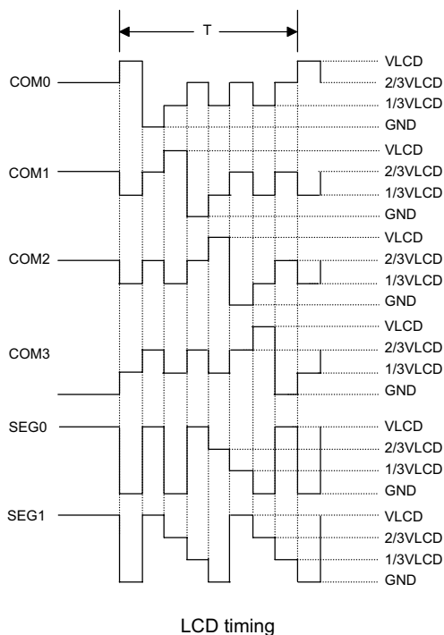
LCD timing
