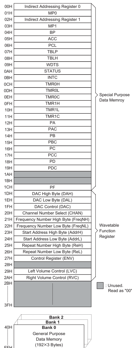
RAM Mapping
