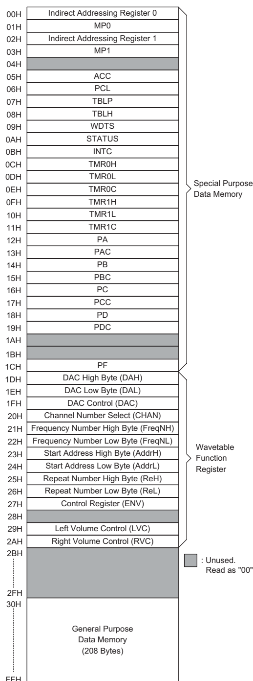
RAM Mapping
