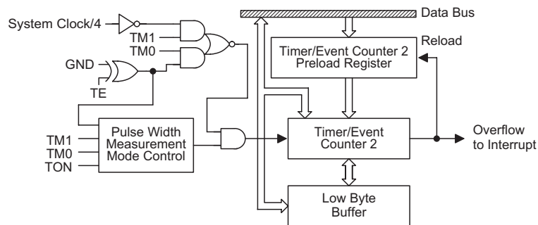
Timer Counter 2
