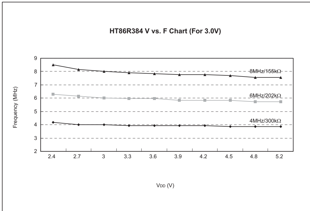
HT86R384 V vs. F Characteristics Curve
