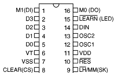
HT6P11 – 16 DIP/SOP
