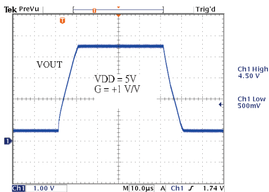
Fig 5. Large-Signal, Non-Inverting Pulse Response
