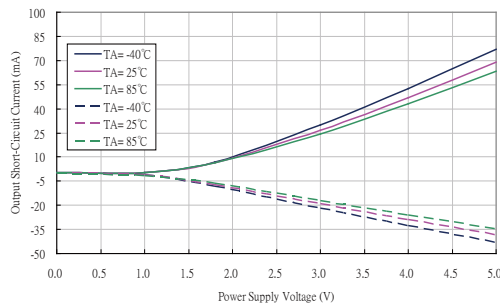
Fig 8. Output Short-Circuit Current vs. Power Supply Voltage
