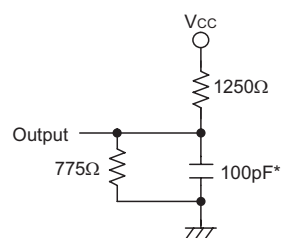
Output Load Circuit
