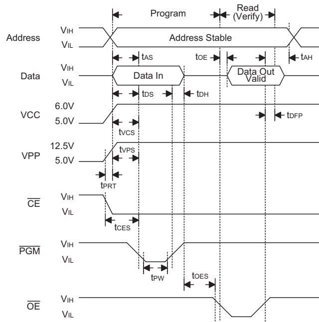
Figure 2. Programming Waveforms
