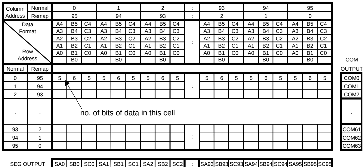
Figure 11 – 65k Color Depth Graphic Display Data RAM Structure
