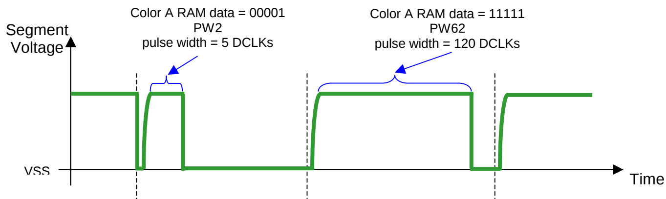
Figure 15 – illustration of relation between graphic display RAM value and gray scale control
