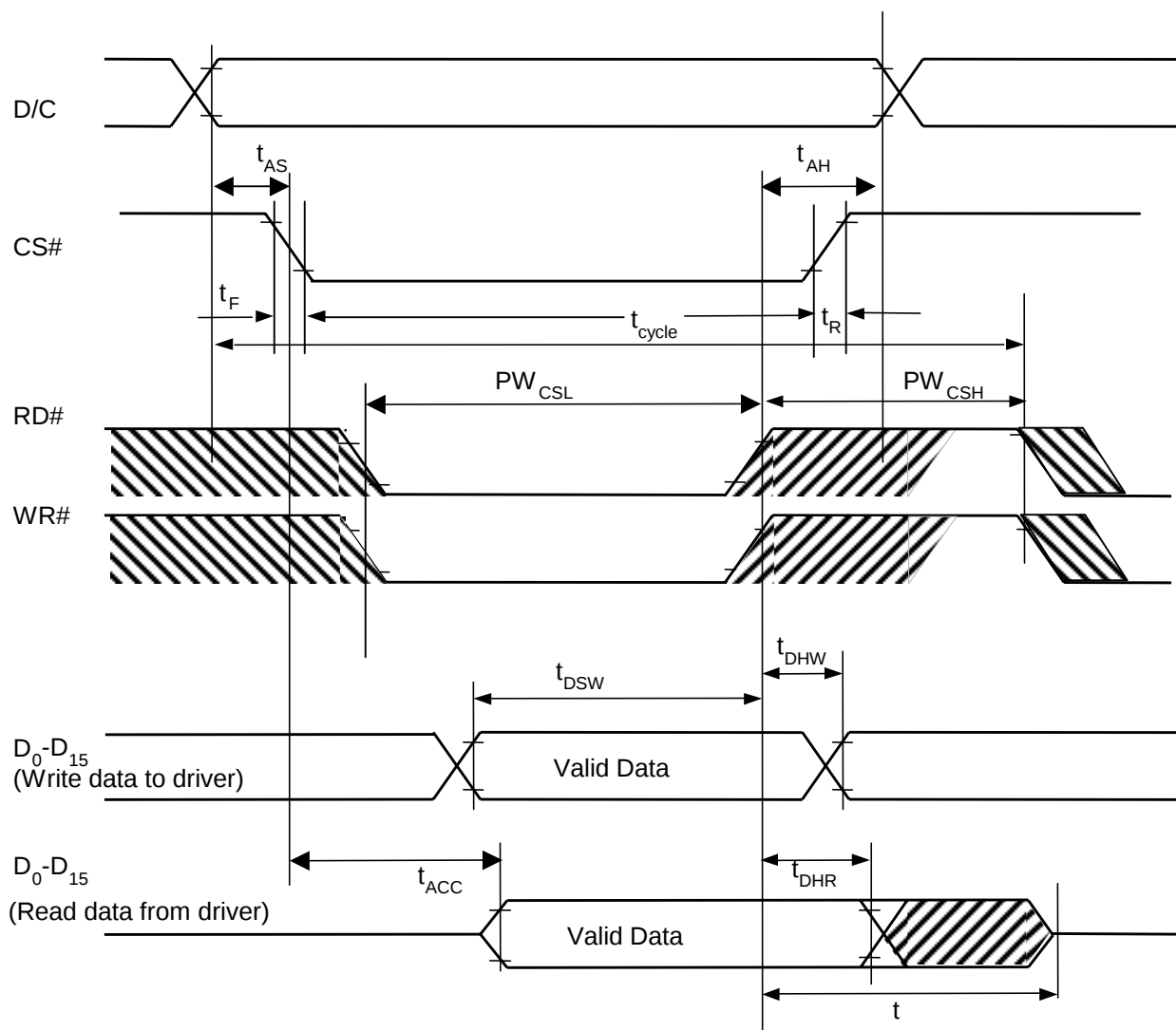
Figure 29 - 8080-series MPU parallel interface characteristics
