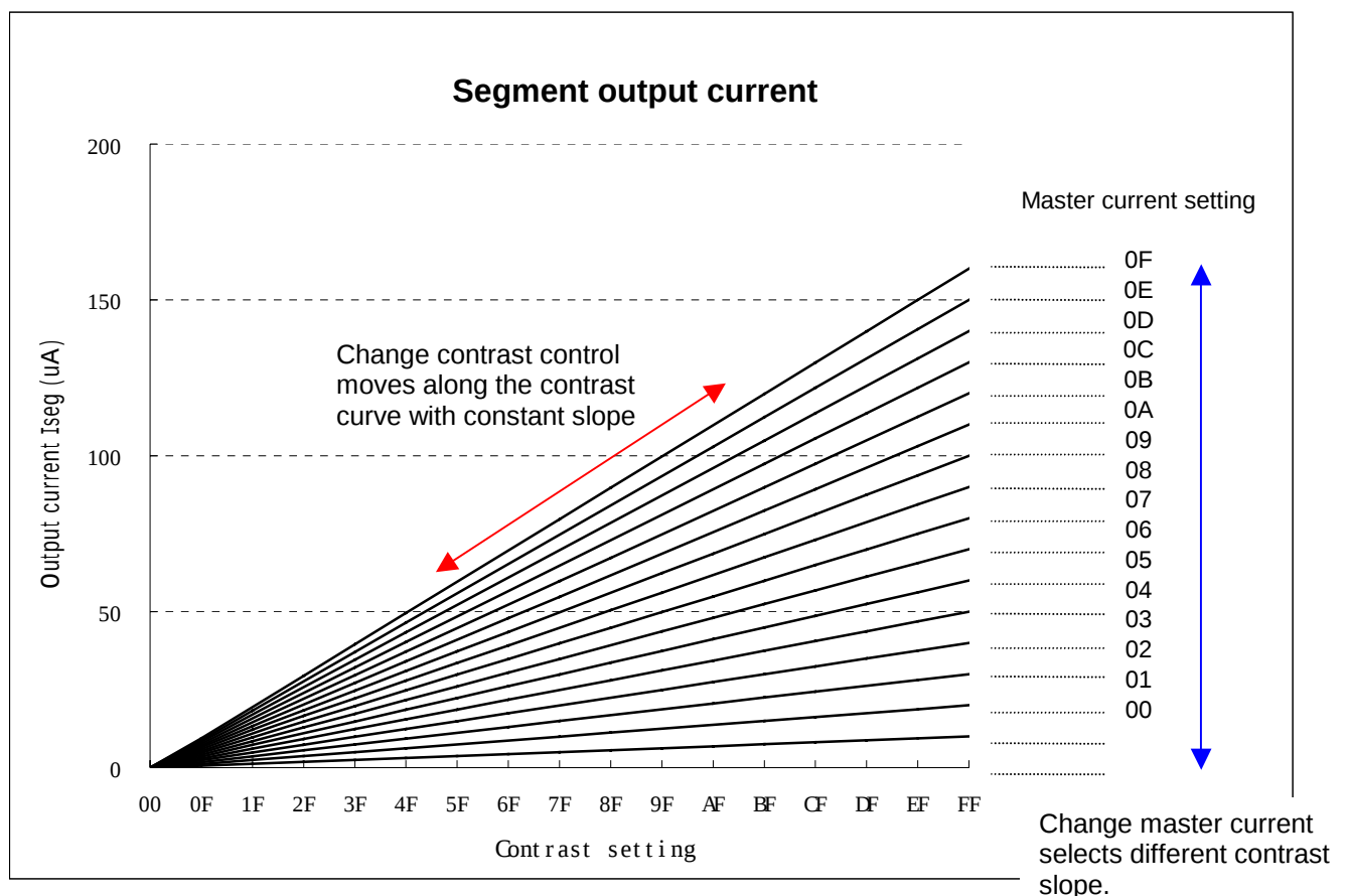
Figure 18 – Segment Output Current for Different Contrast Control and Master Current Setting
