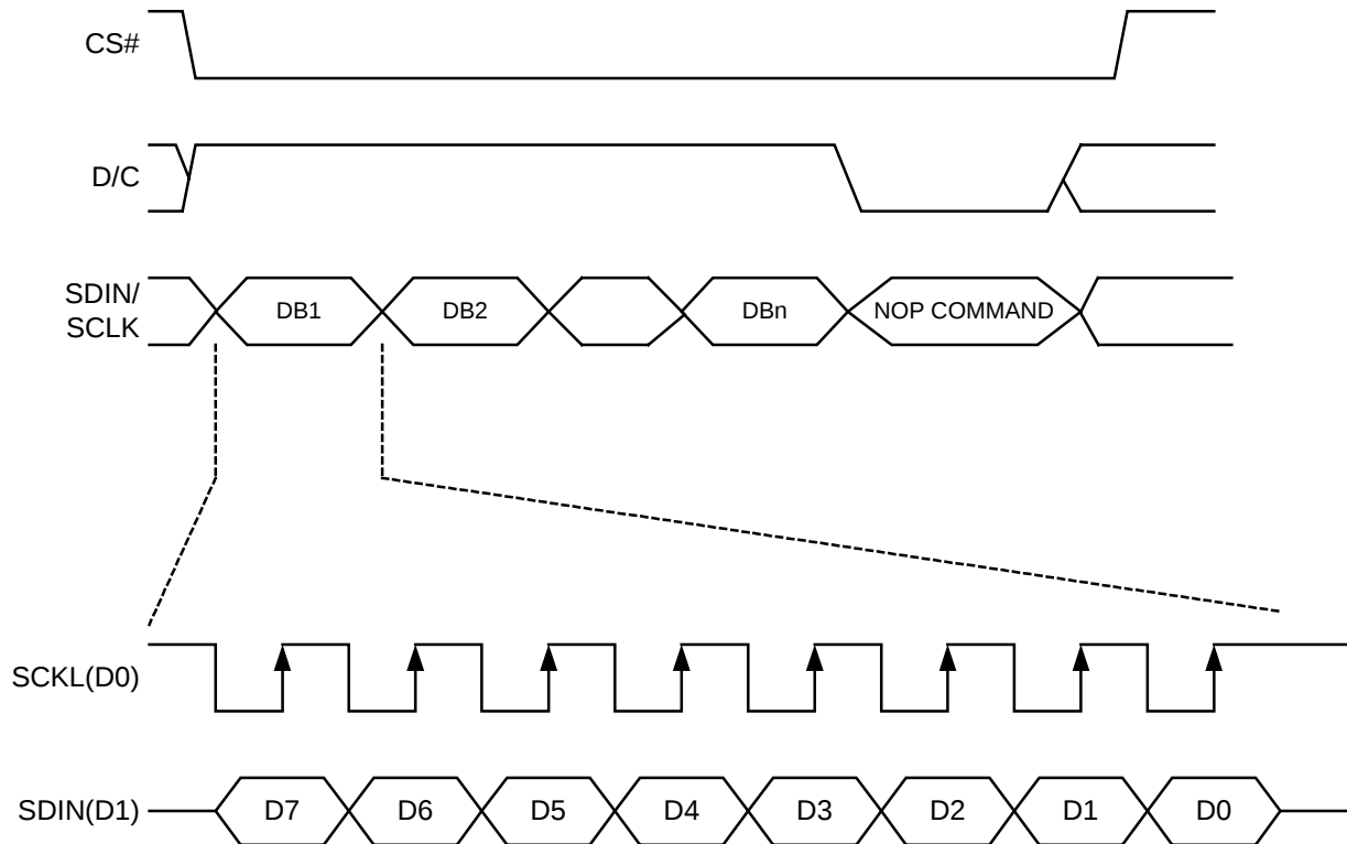
Figure 10 - Display data write procedure in SPI mode
