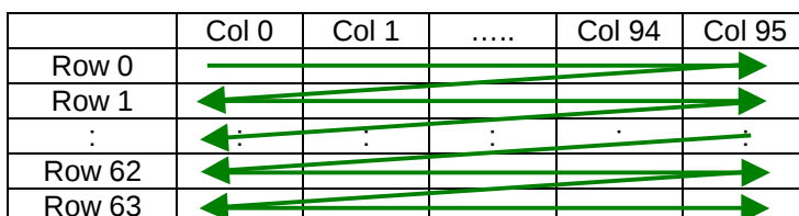
Figure 19 – Address Pointer Movement of Horizontal Address Increment Mode
