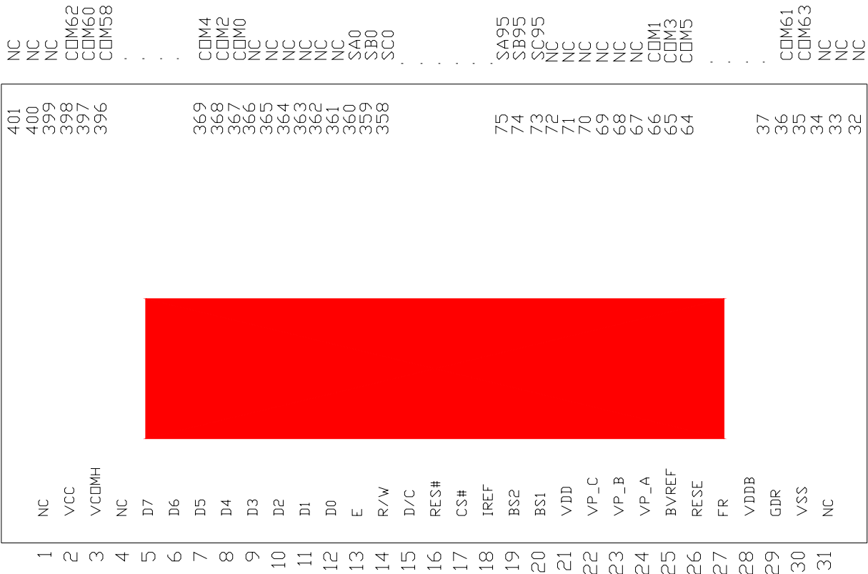
Figure 33 - SSD1332T1R1 TAB pin assignment
