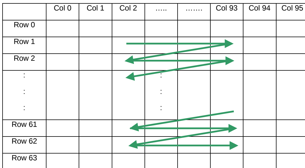
Figure 17 – Example of Column and Row Address Pointer Movement
