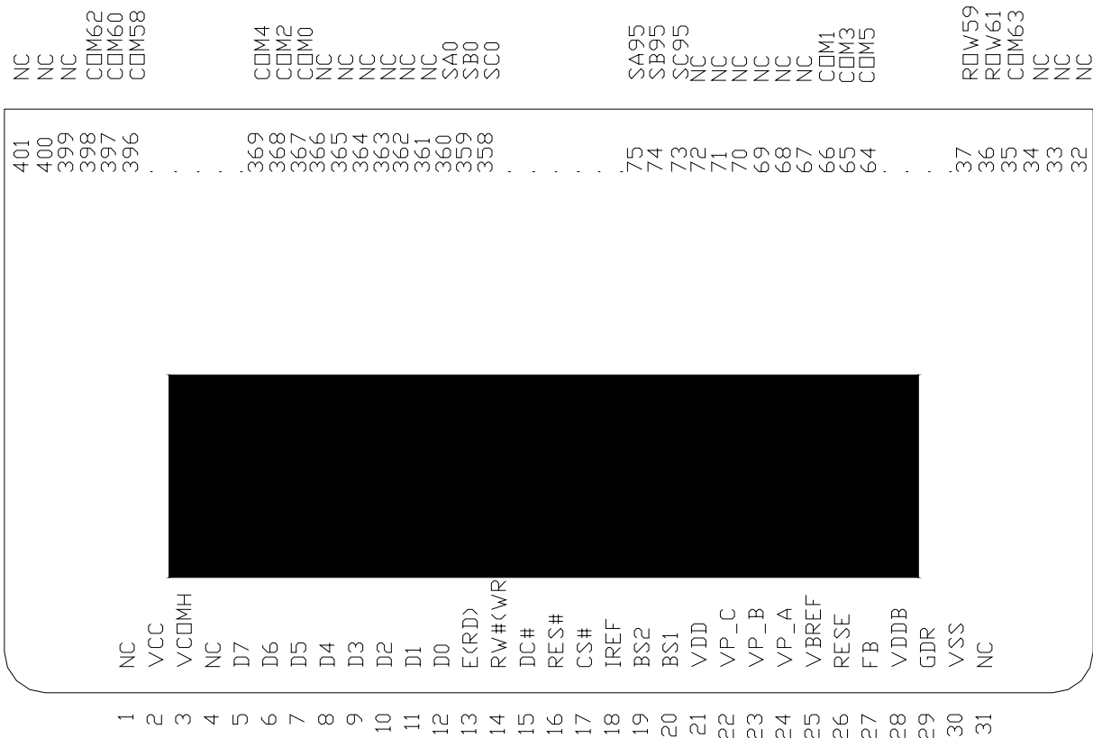
Figure 32 - SSD1332U1R1 COF pin assignment
