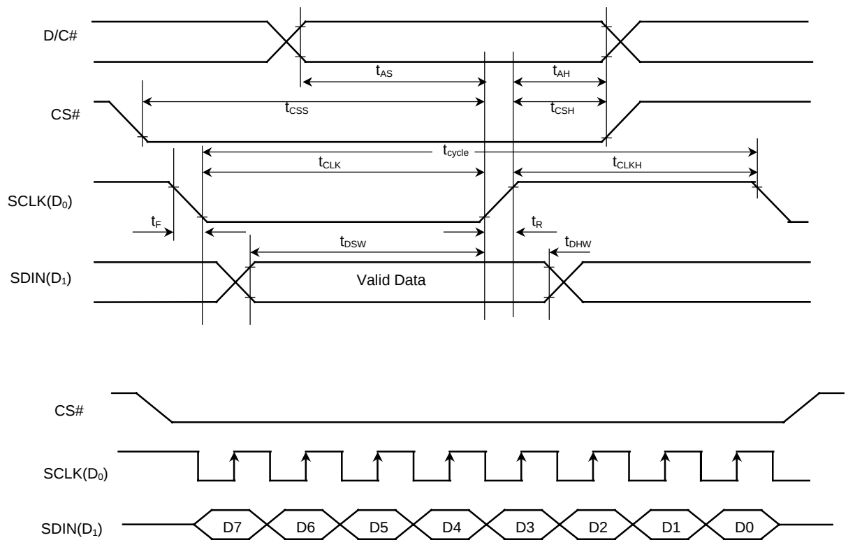
Figure 30 - Serial interface characteristics
