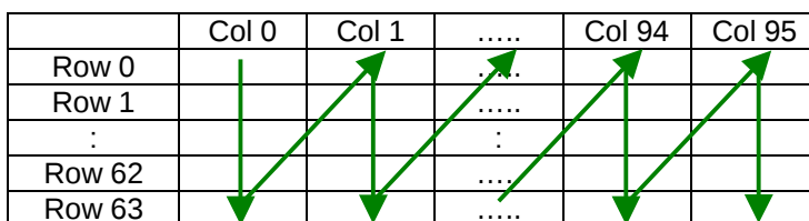
Figure 20 – Address Pointer Movement of Vertical Address Increment Mode
