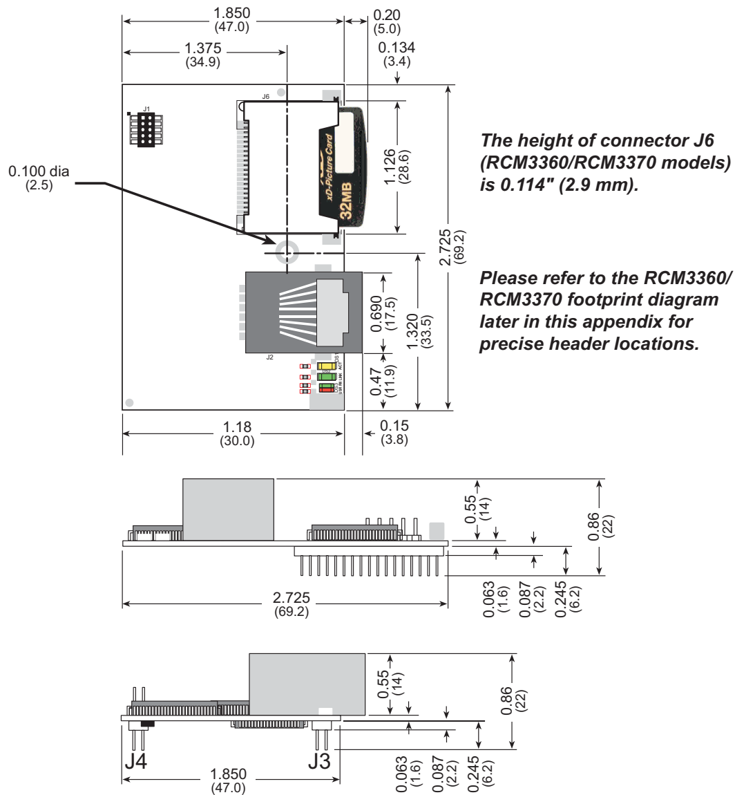
Figure A-1. RCM3360/RCM3370 Dimensions
