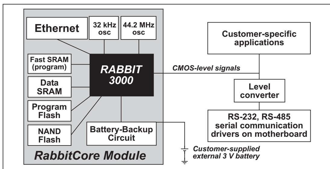
Figure 4. RCM3360/RCM3370 Subsystems
