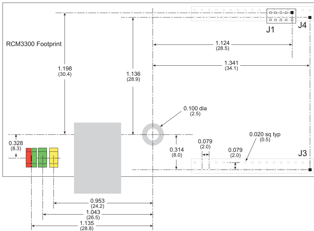
Figure A-3. User Board Footprint for RCM3360/RCM3370
