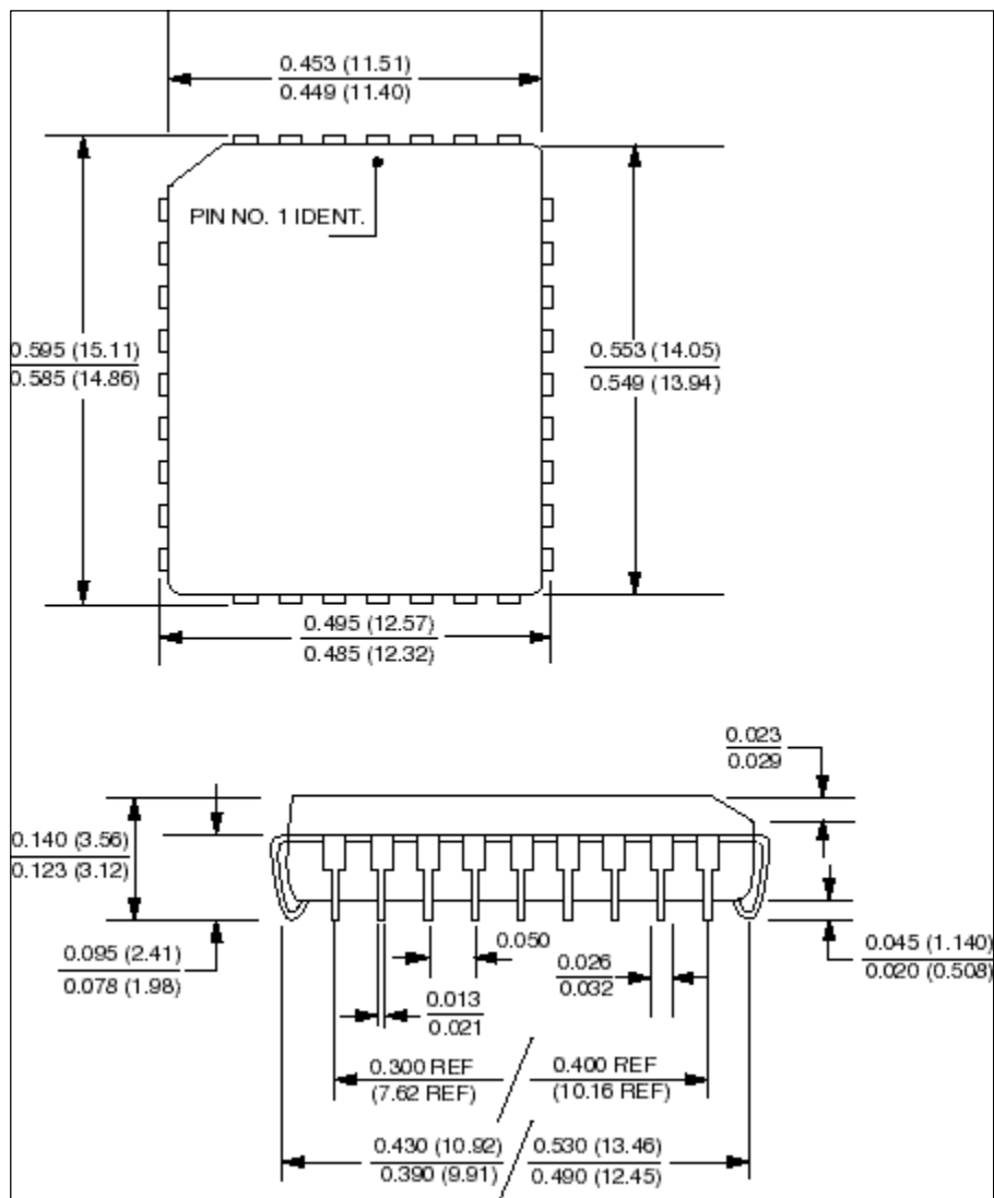
32-Pin PLCC
