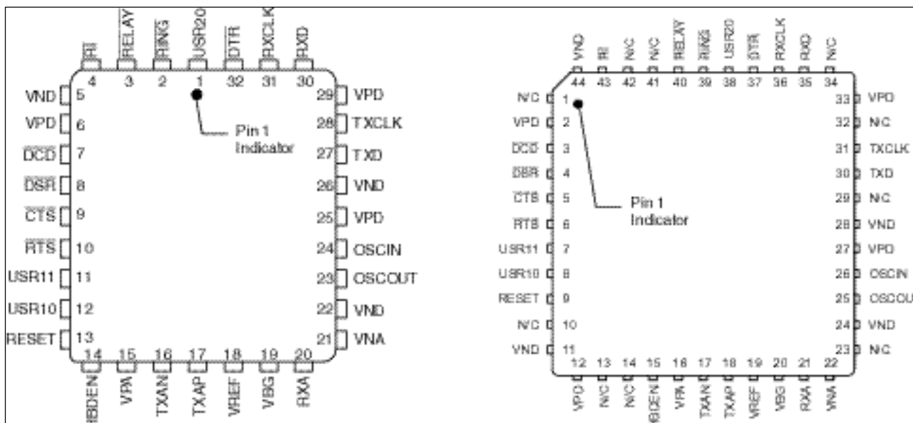
32-Lead PLCC 73M2901-32IH/5
