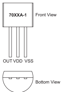
TO-92
