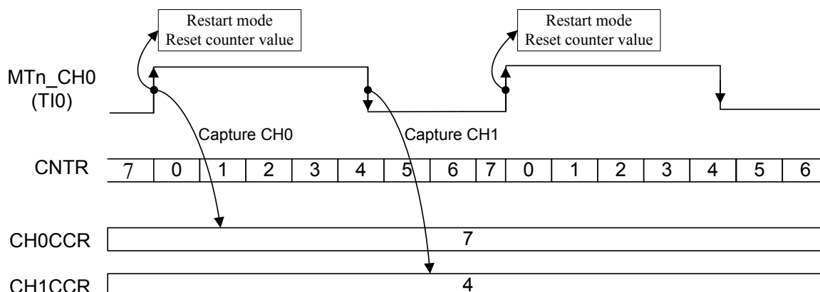
Figure 92. PWM Pulse Width Measurement Example
