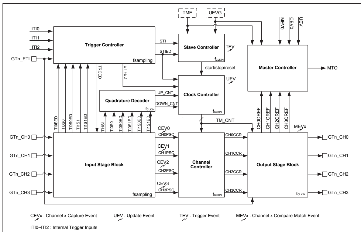
Figure 38. GPTM Block Diagram
