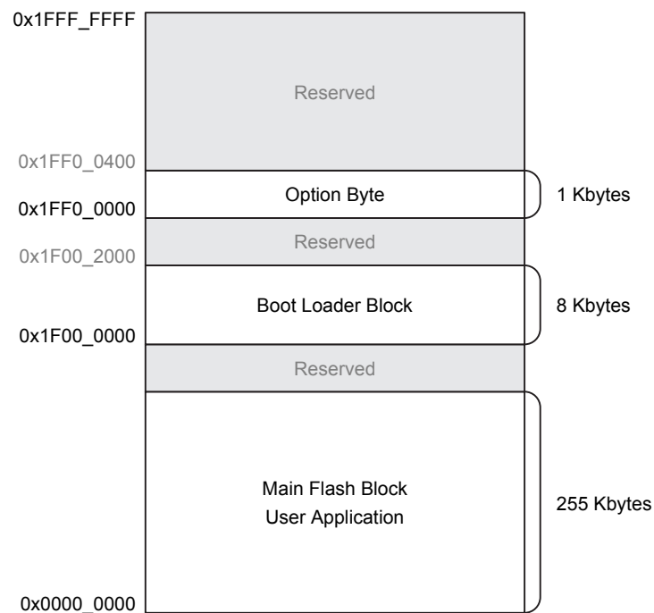
Figure 6. Flash Memory Map
