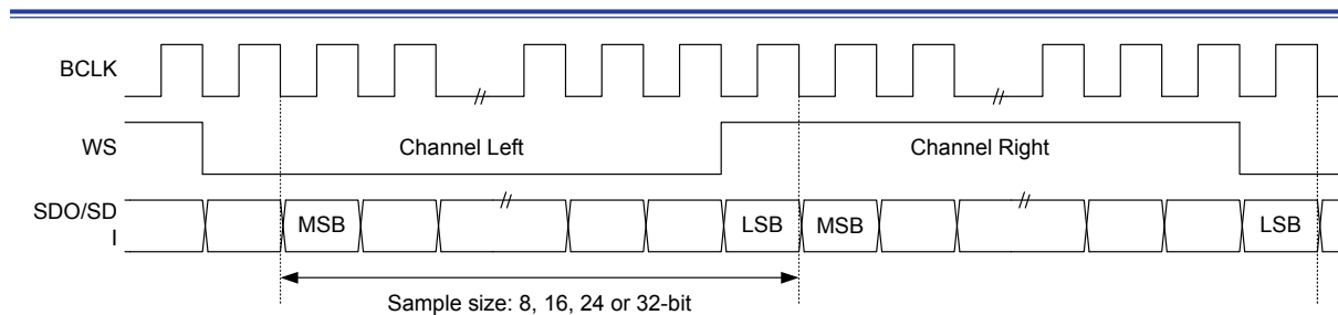
Figure 197. I 2 S-justified Stereo Mode Waveforms
