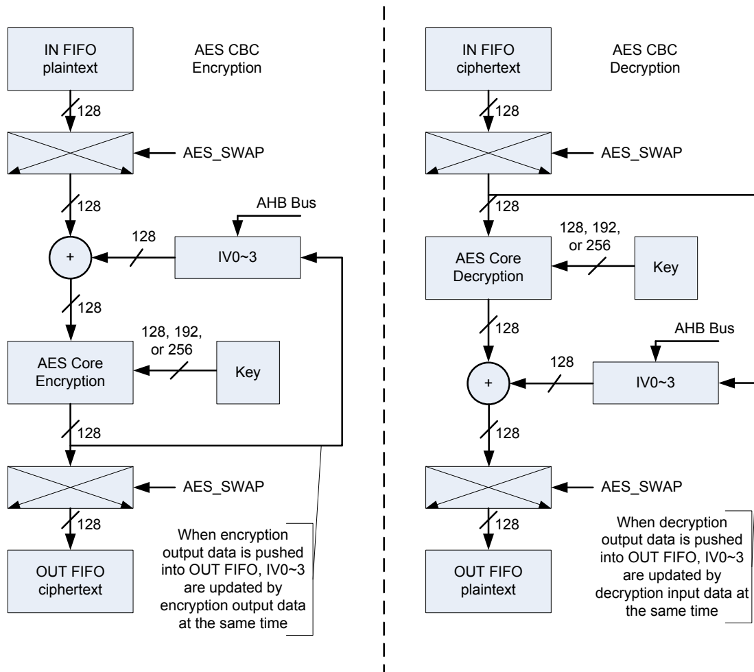
Figure 216. CBC Mode of AES
