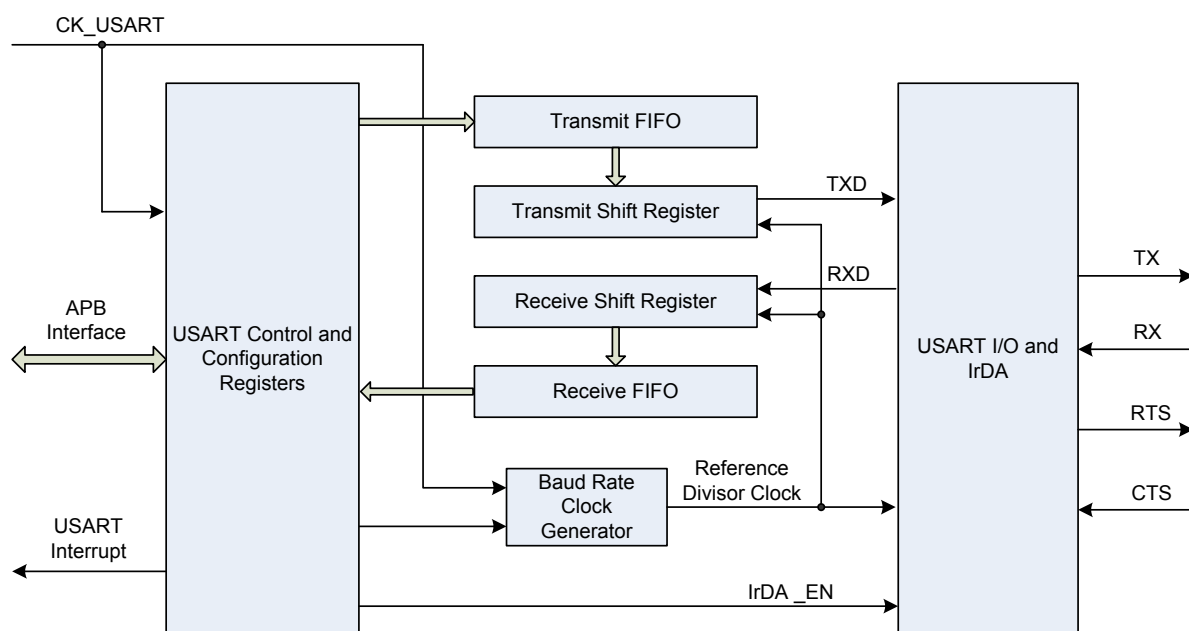
Figure 150. USART Block Diagram
