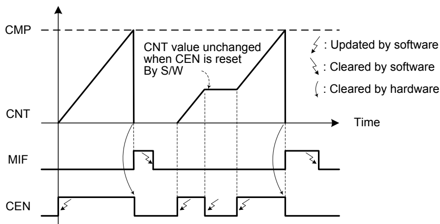
Figure 75. BFTM – One Shot Mode
