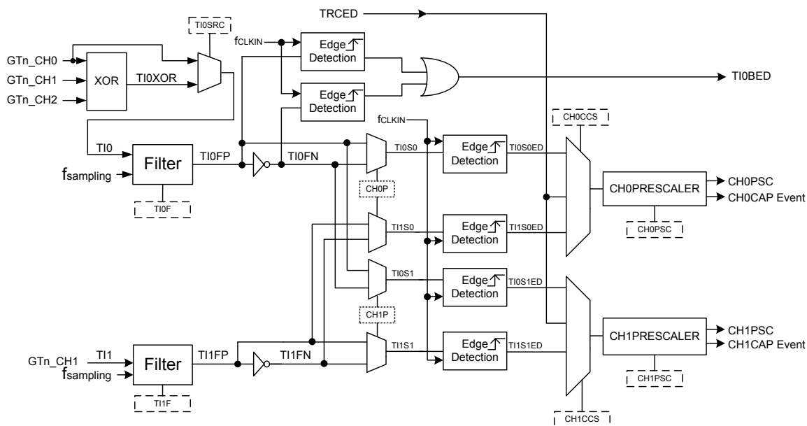
Figure 53. Channel 0 and Channel 1 Input Stage
