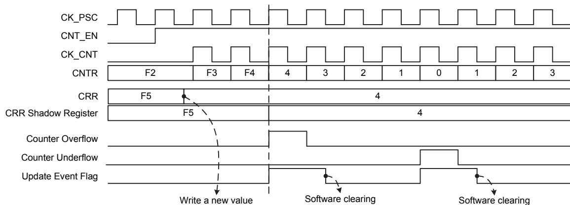
Figure 41. Center-aligned Counting Example
