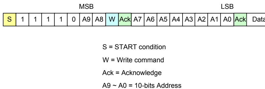
Figure 130. 10-bit Addressing Write Transmit Mode
