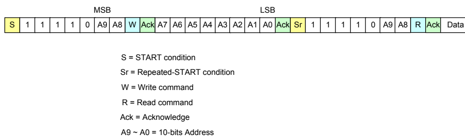
Figure 131. 10-bit Addressing Read Receive Mode
