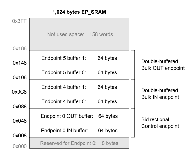
Figure 171. Endpoint Buffer Allocation Example
