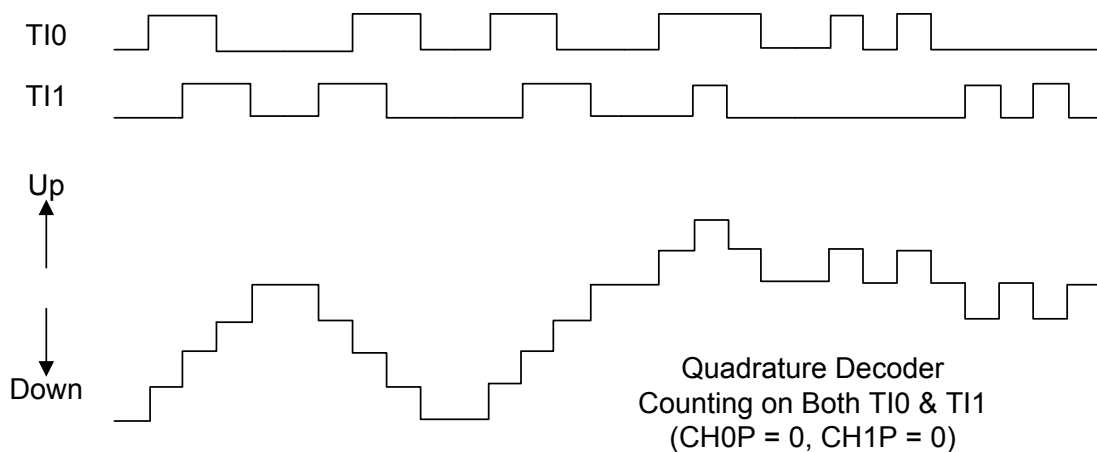
Figure 63. Both TI0 and TI1 Quadrature Decoder Counting.
