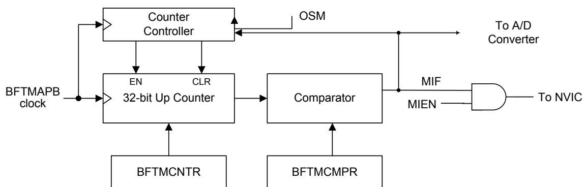
Figure 73. BFTM Block Diagram
