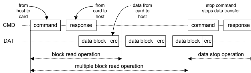
Figure 227. "Multiple" Block Read Operation
