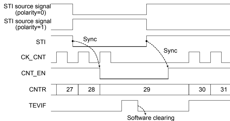
Figure 86. MCTM in Pause Mode
