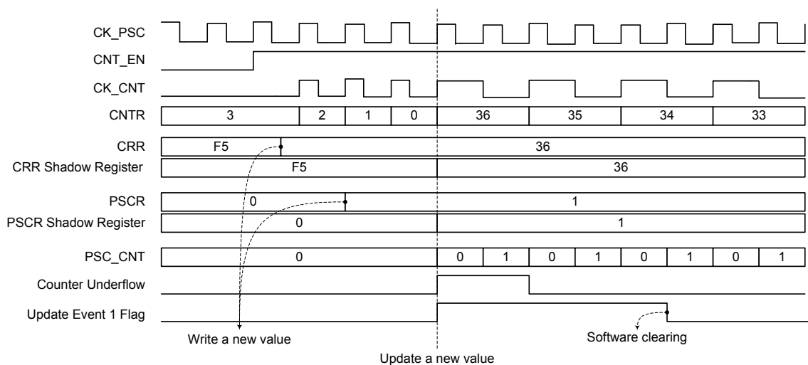
Figure 79. Down-counting Example
