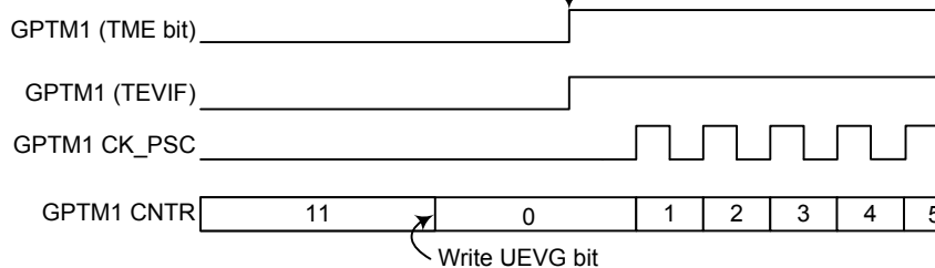
Figure 71. Trigger GPTM0 and GPTM1 with the GPTM0 CH0 Input
