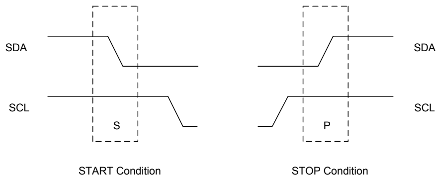
Figure 127. START and STOP Condition
