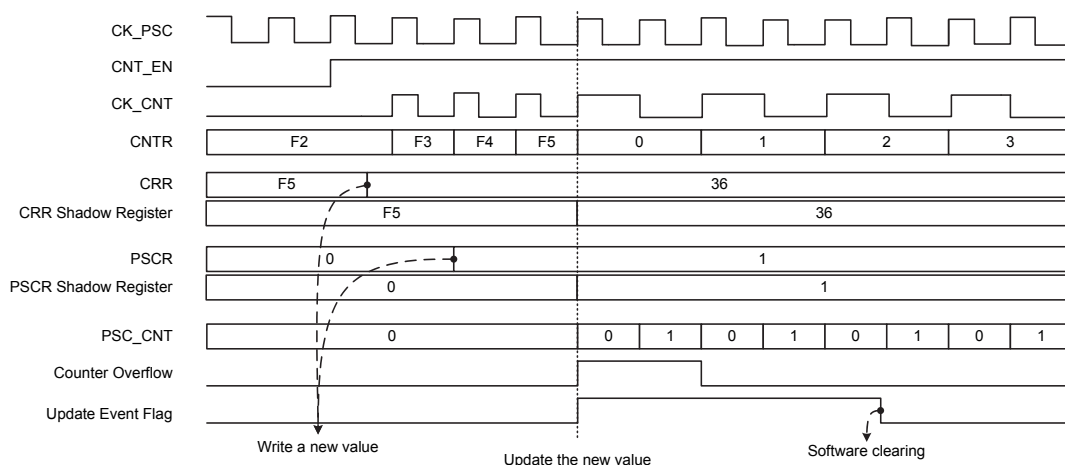
Figure 39. Up-counting Example
