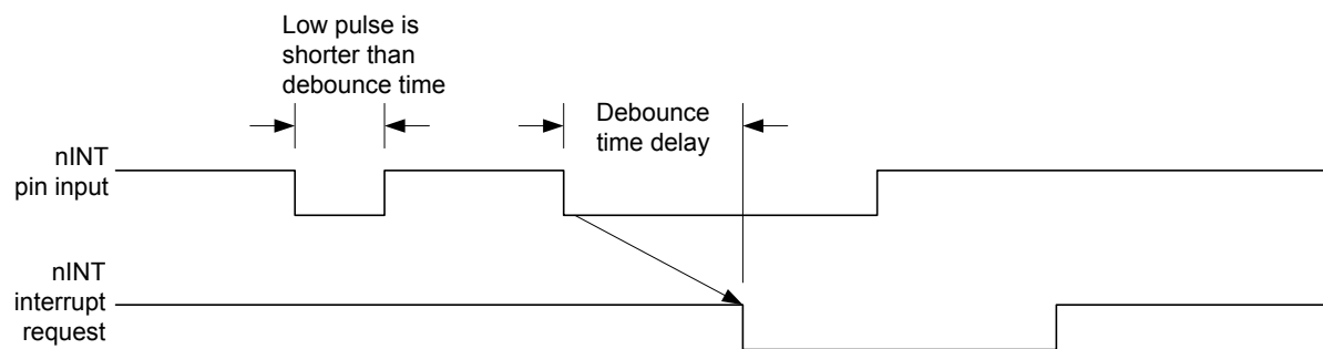
Figure 27. EXTI Interrupt Debounce Function
