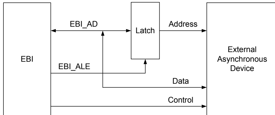
Figure 181. An EBI Address Latch Setup Diagram
