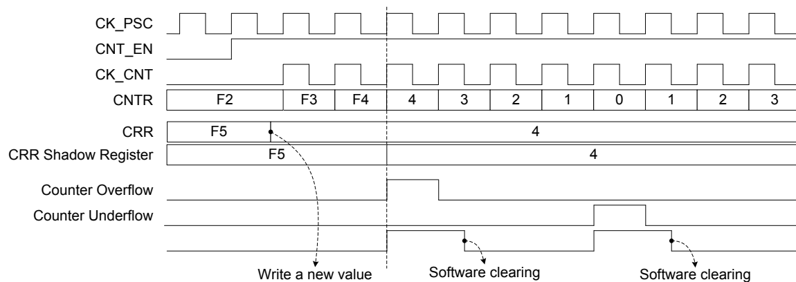
Figure 80. Center-aligned Counting Example
