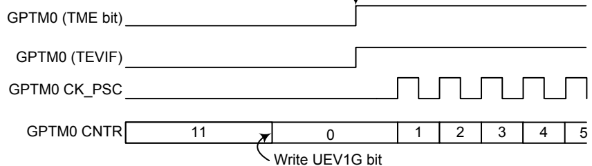
Figure 120. Trigger MCTM0 and GPTM0 with the MCTM0 CH0 Input
