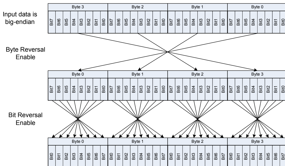
Figure 213. CRC Data Bit and Byte Reversal Example
