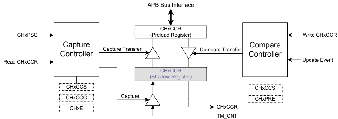
Figure 50. Capture/Compare Block Diagram
