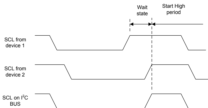
Figure 133. Clock Synchronization during Arbitration
