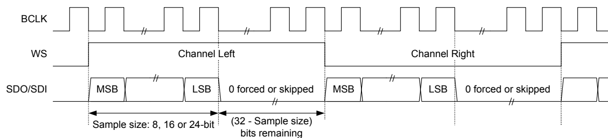
Figure 200. Left-justified Stereo Mode Waveforms (32-bit Channel Enabled)
