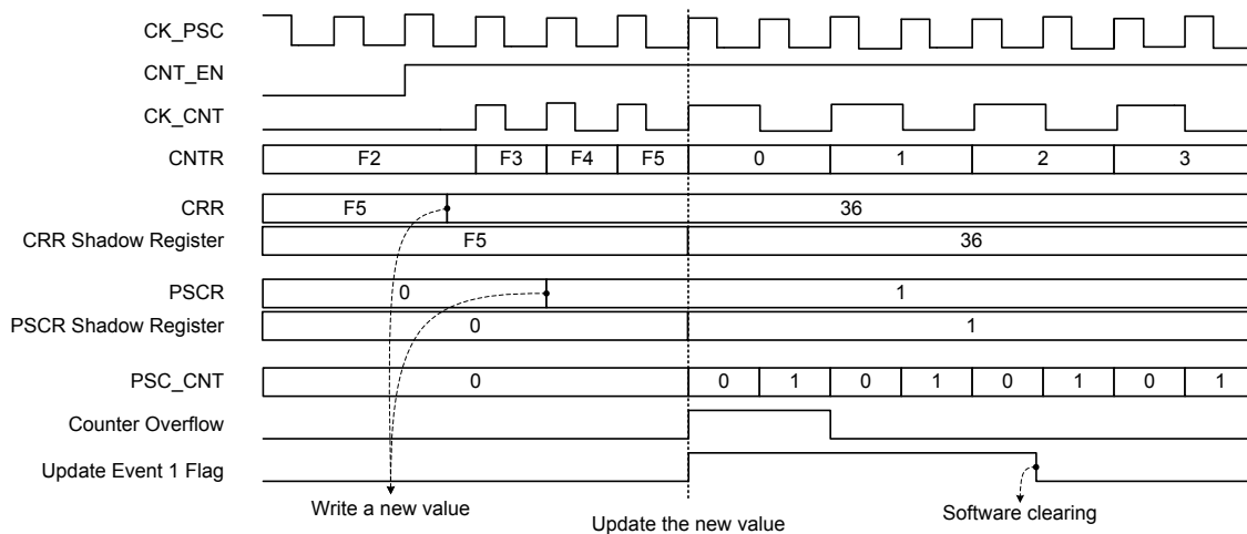
Figure 78. Up-counting Example
