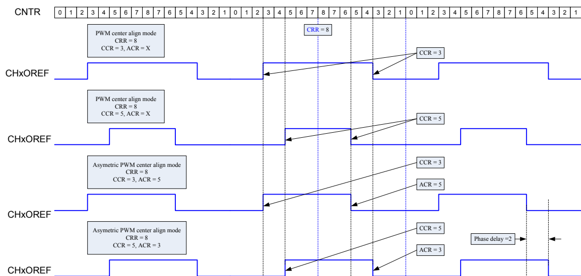
Figure 117. Asymmetric PWM Mode versus Center-aligned Counting mode
