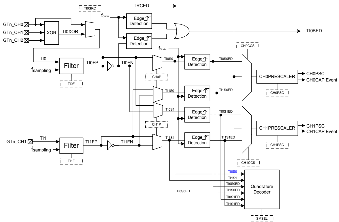
Figure 62. Input Stage and Quadrature Decoder Block Diagram
