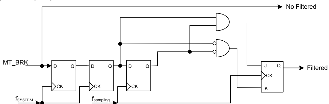
Figure 103. MT_BRK Pin Digital Filter Diagram with N = 2
