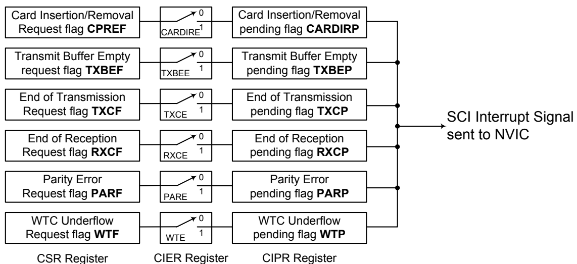
Figure 169. SCI Interrupt Structure
