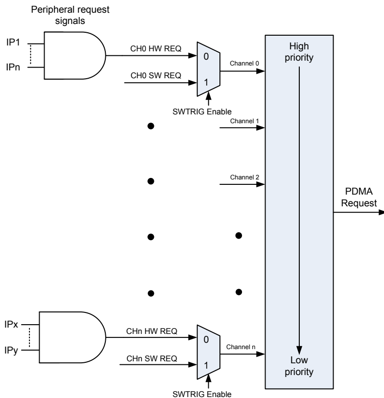
Figure 174. PDMA Request Mapping Architecture
