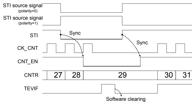
Figure 46. GPTM in Pause Mode
