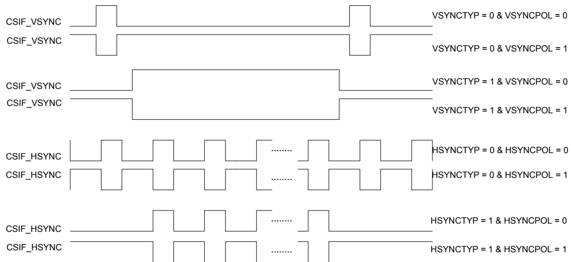
Figure 236. VSYNC & HSYNC Timing
