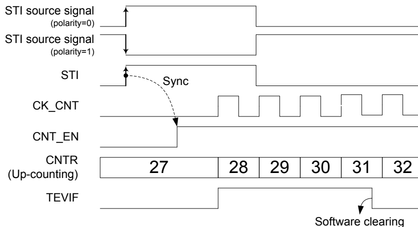
Figure 47. GPTM in Trigger Mode
