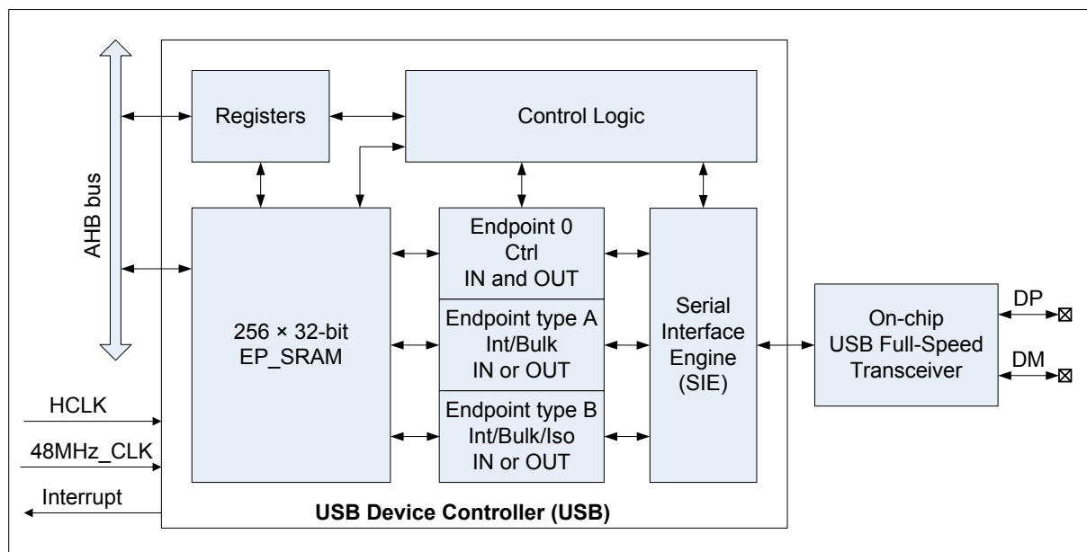
Figure 170. USB Block Diagram
