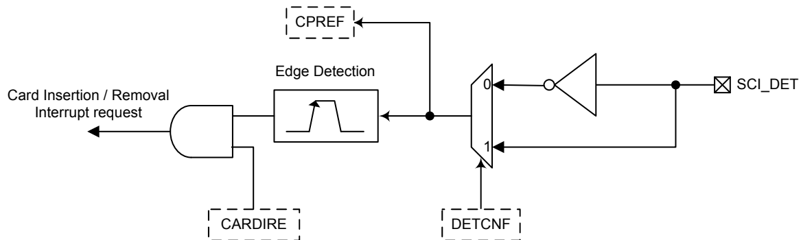
Figure 168. SCI Card Detection Diagram
