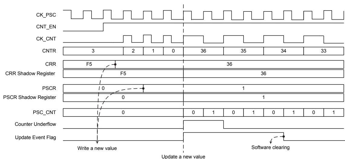
Figure 40. Down-counting Example
