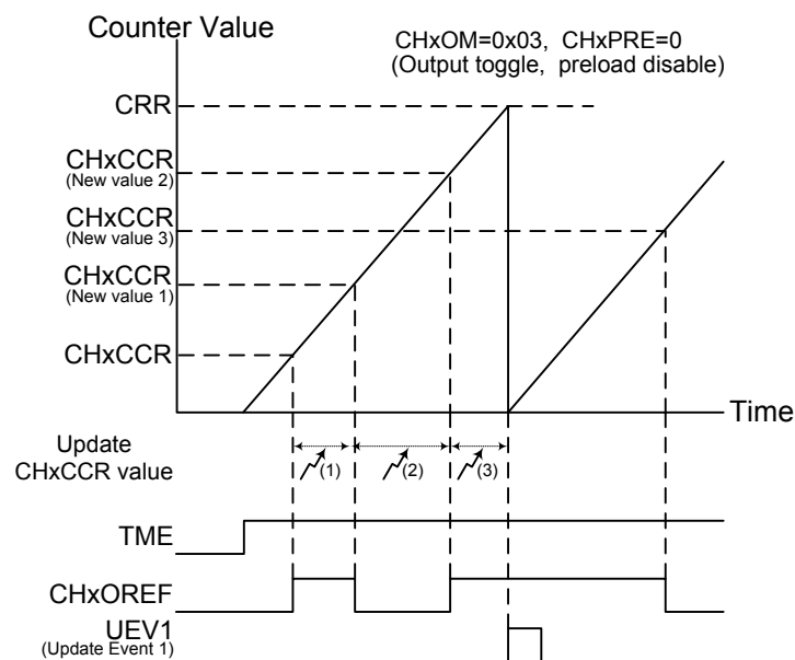
Figure 96. Toggle Mode Channel Output Reference Signal – CHxPRE = 0
