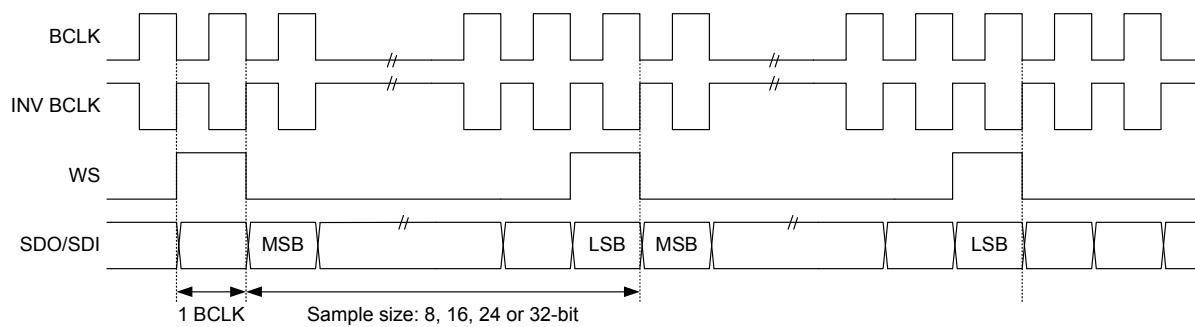
Figure 205. Left-justified Mono Mode Waveforms
