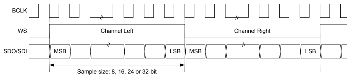
Figure 199. Left-justified Stereo Mode Waveforms
