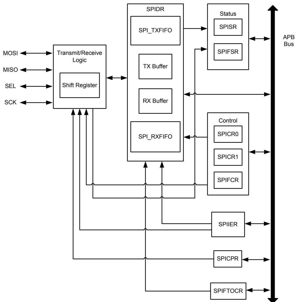
Figure 140. SPI Block Diagram
