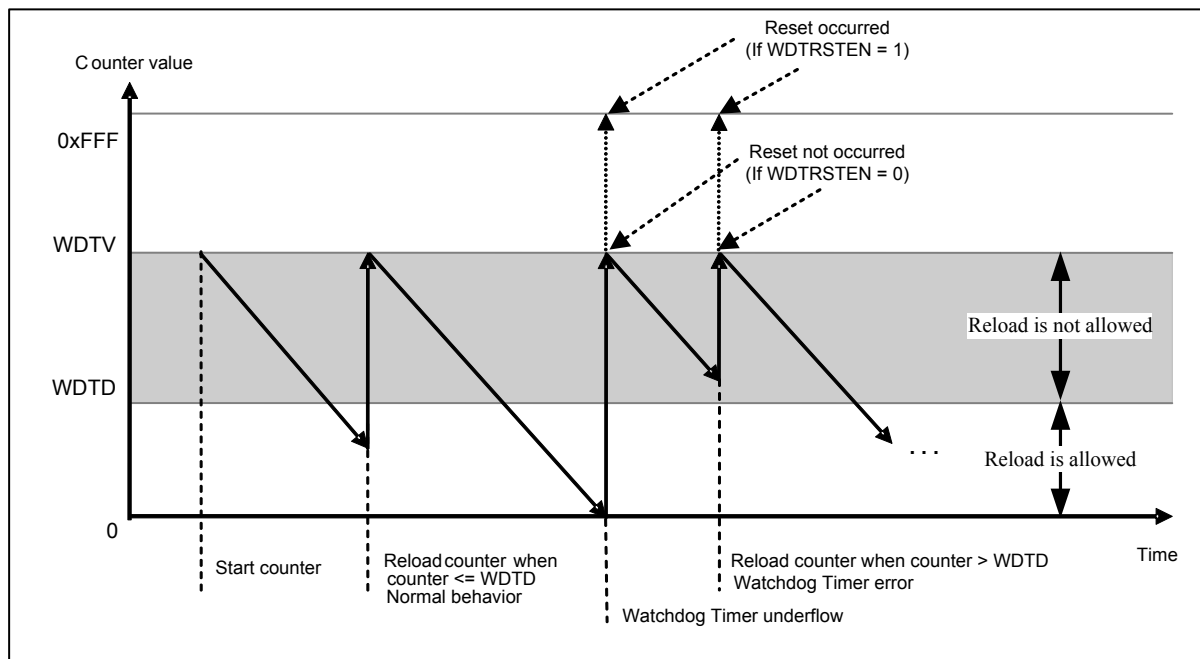
Figure 125. Watchdog Timer Behavior
