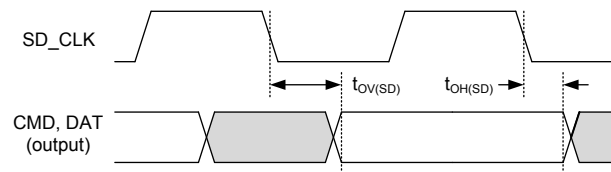
Figure 223. Normal Speed Timing
