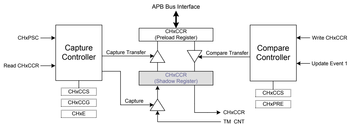
Figure 90. Capture/Compare Block Diagram
