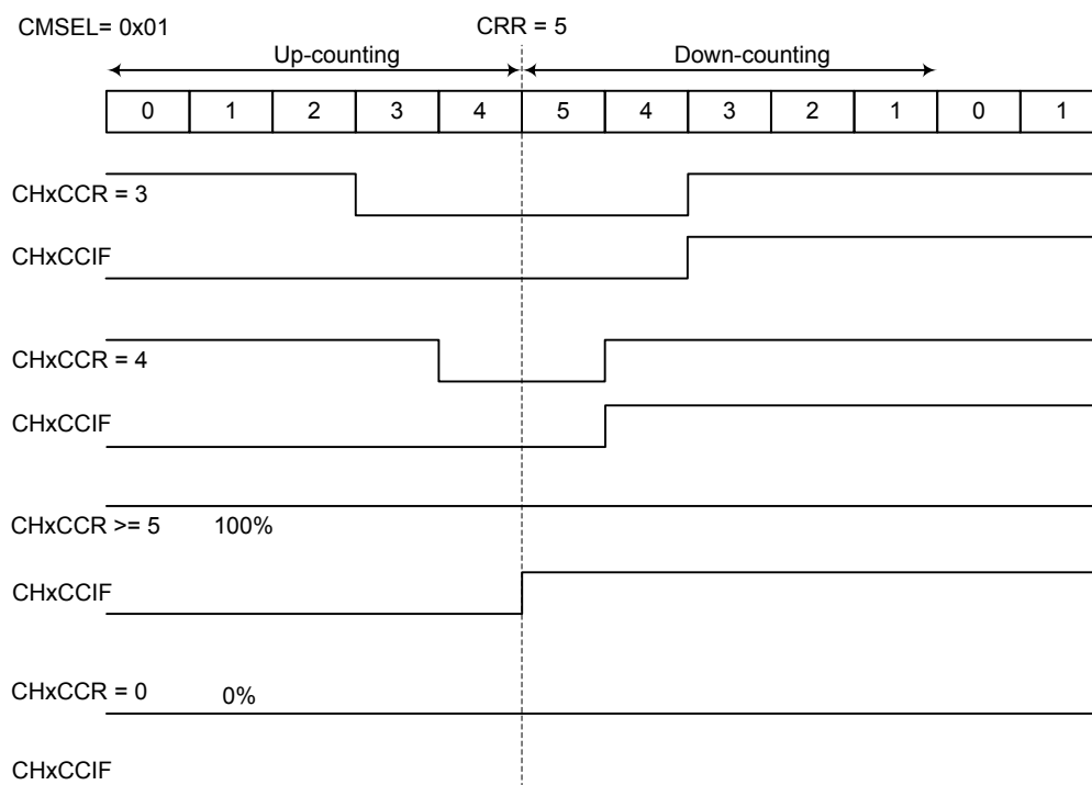
Figure 100. PWM Mode 1 Channel Output Reference Signal and Counter in Centre-aligned Counting Mode
