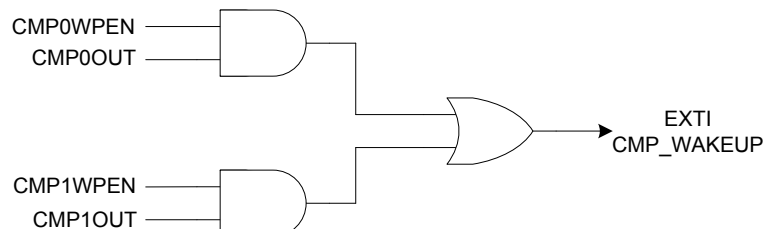
Figure 37. Wakeup Signals of Comparators
