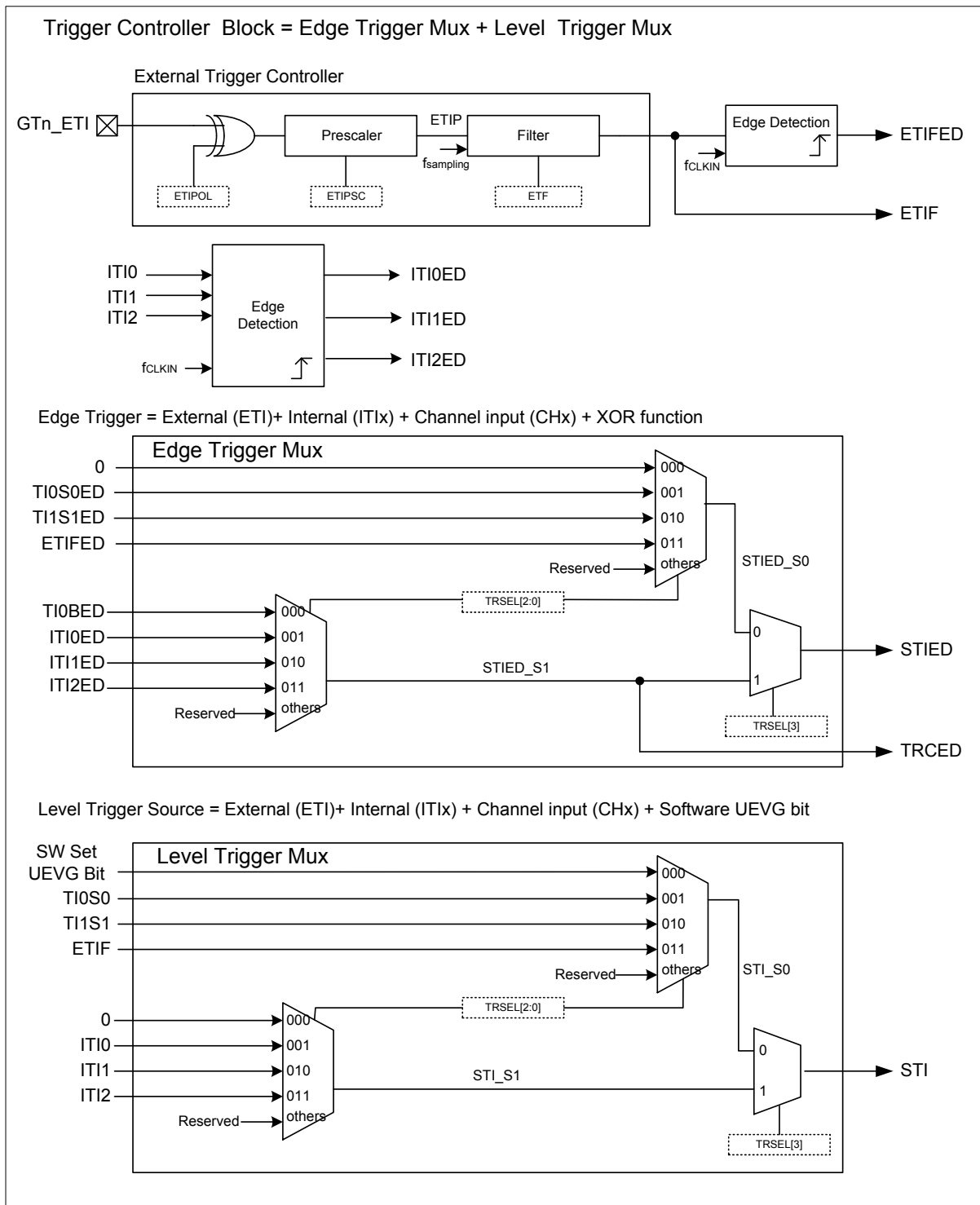
Figure 43. Trigger Control Block
