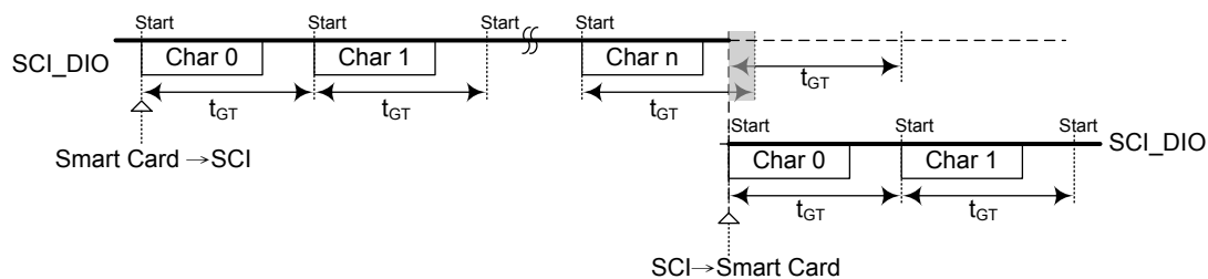
Figure 166. Guard Time Duration
