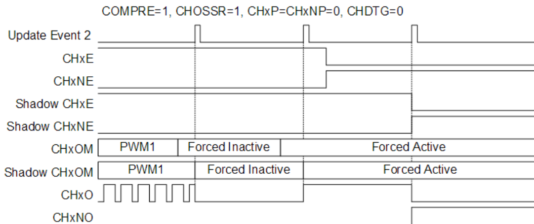
Figure 109. CHxE, CHxNE and CHxOM Updated by Update Event 2
