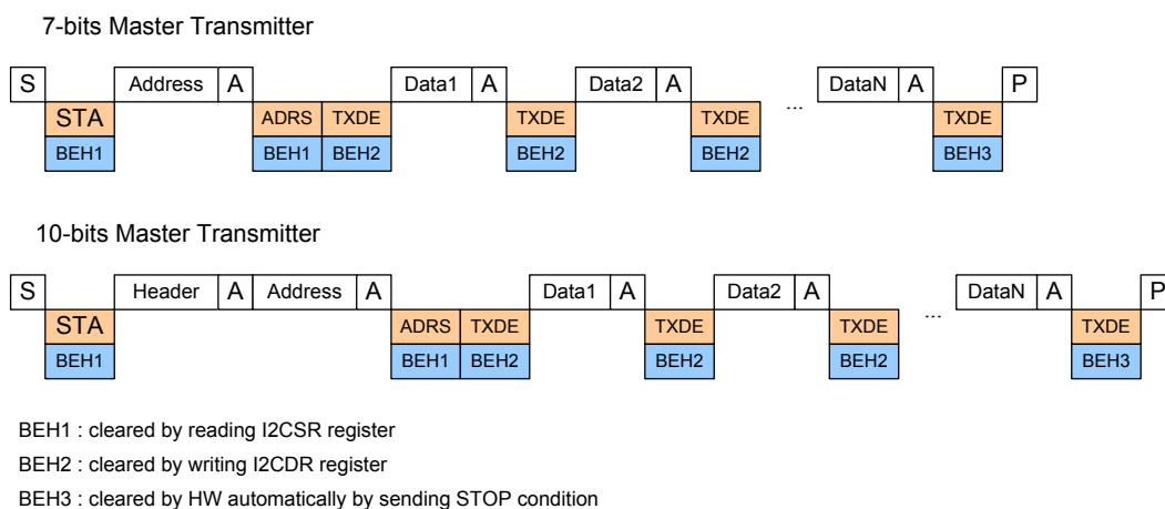
Figure 135. Master Transmitter Timing Diagram
