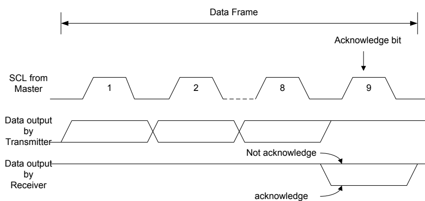
Figure 132. I 2 C Bus Acknowledge
