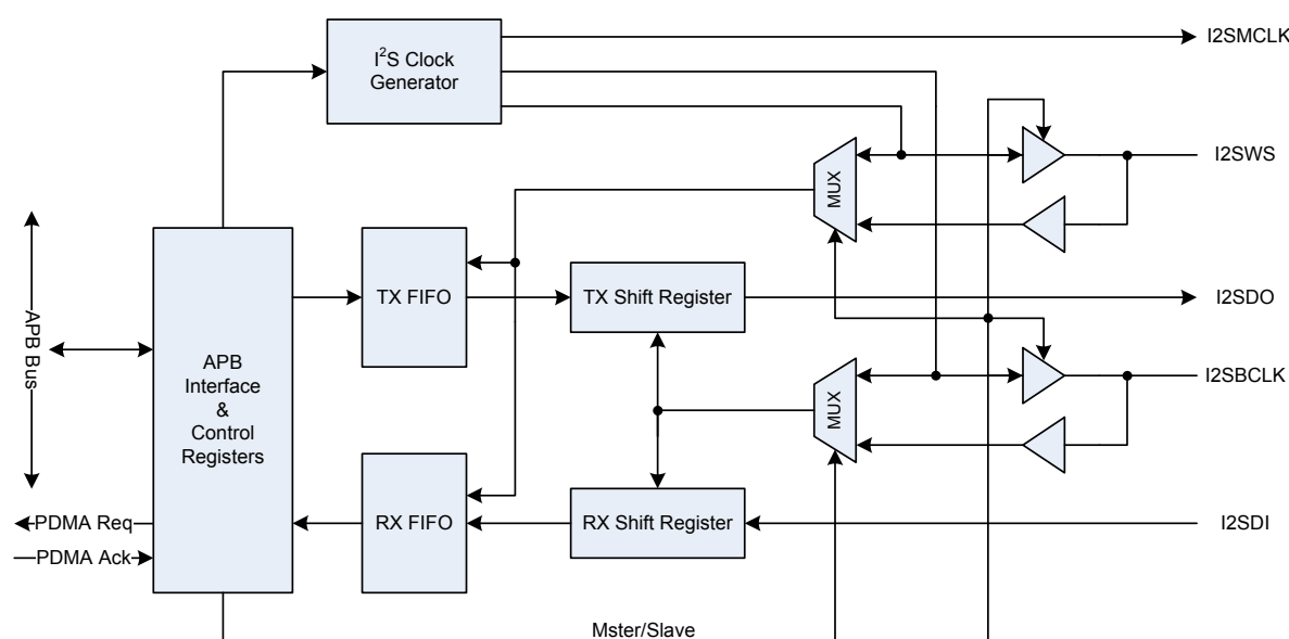
Figure 194. I 2 S Block Diagram
