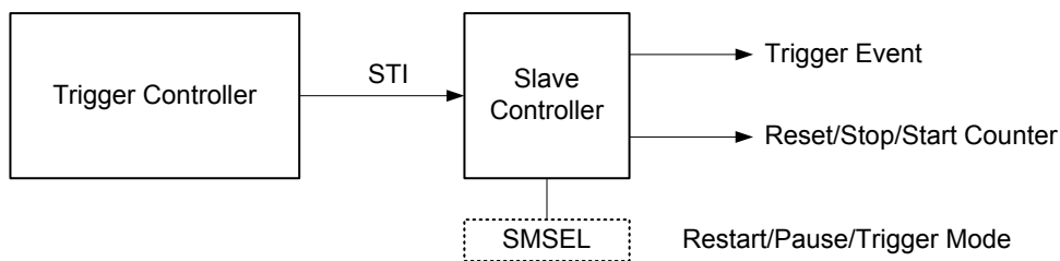
Figure 84. Slave Controller Diagram
