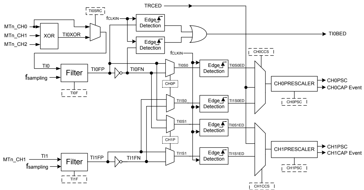
Figure 93. Channel 0 and Channel 1 Input Stages
