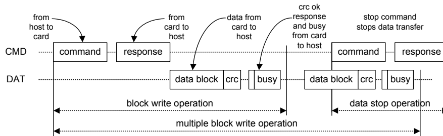
Figure 228. "Multiple" Block Write Operation
