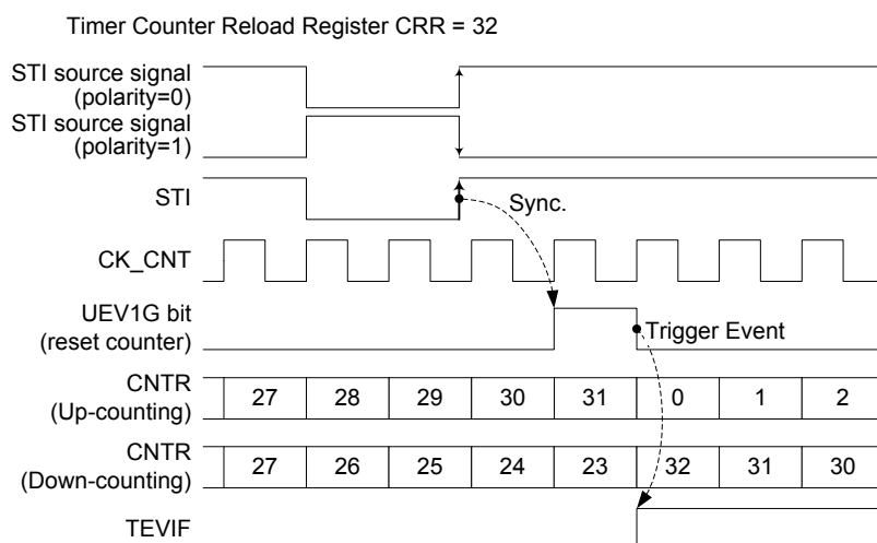
Figure 85. MCTM in Restart Mode
