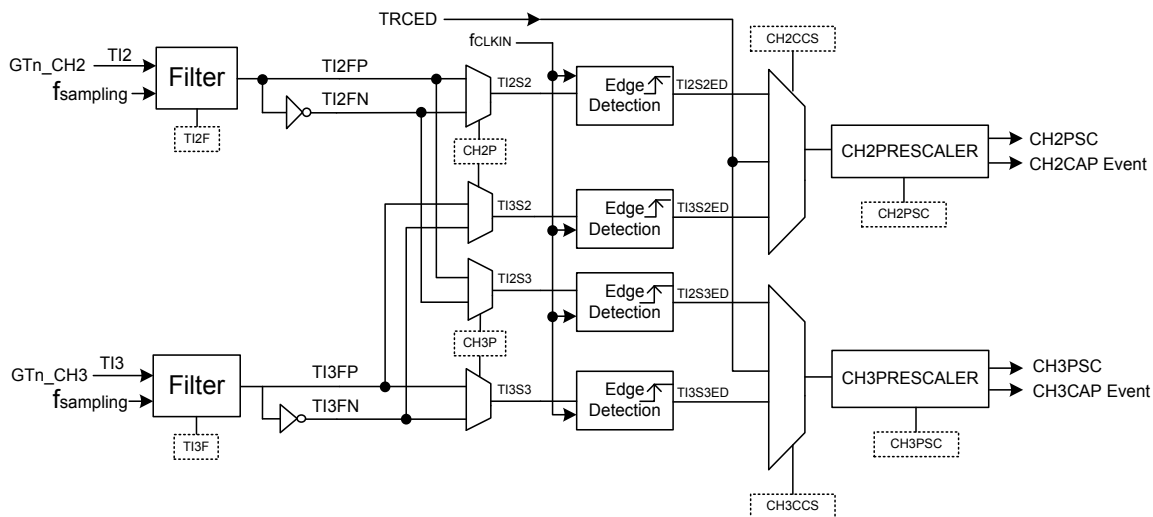
Figure 54. Channel 2 and Channel 3 Input Stage
