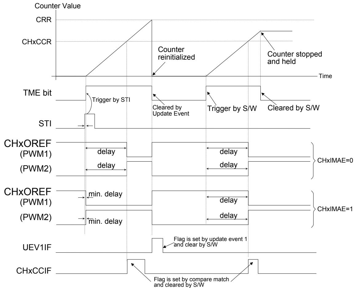
Figure 115. Single Pulse Mode
