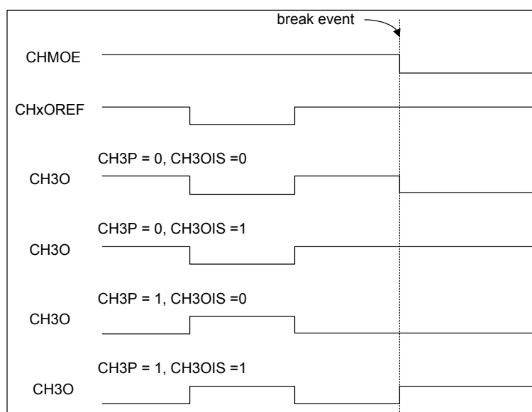
Figure 104. Channel 3 Output with a Break Event Occurrence
