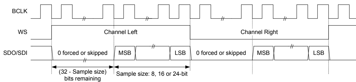
Figure 202. Right-justified Stereo Mode Waveforms (32-bit Channel Enabled)
