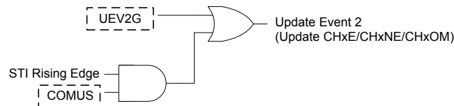
Figure 110. Update Event 2 Setup Diagram
