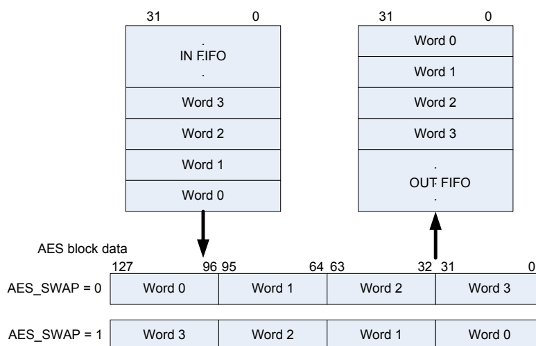
Figure 220. AES Word Swap Function
