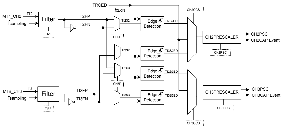
Figure 94. Channel 2 and Channel 3 Input Stages
