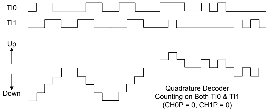
Figure 112. Both TI0 and TI1 Quadrature Decoder Counting
