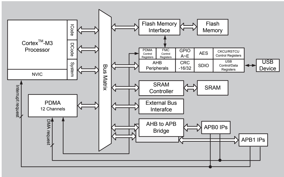
Figure 3. Bus Architecture
