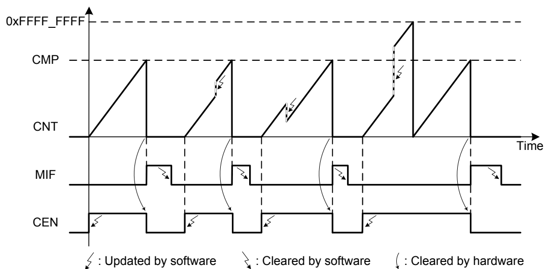
Figure 76. BFTM – One Shot Mode Counter Updating
