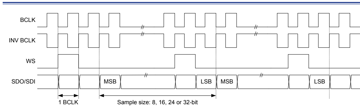
Figure 203. I 2 S-justified Mono Mode Waveforms
