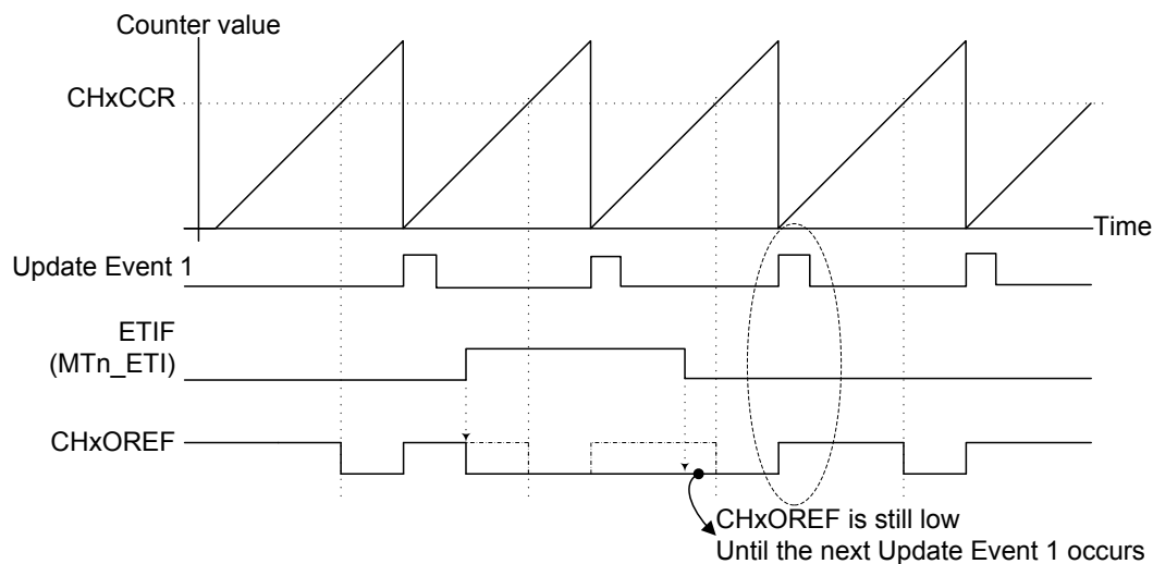
Figure 114. Clearing CHxOREF by ETIF
