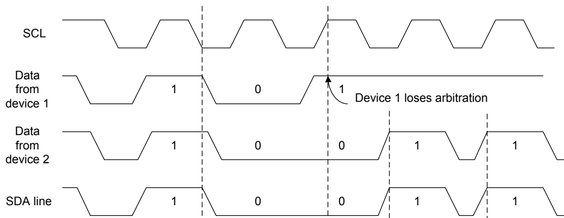
Figure 134. Two Master Arbitration Procedure
