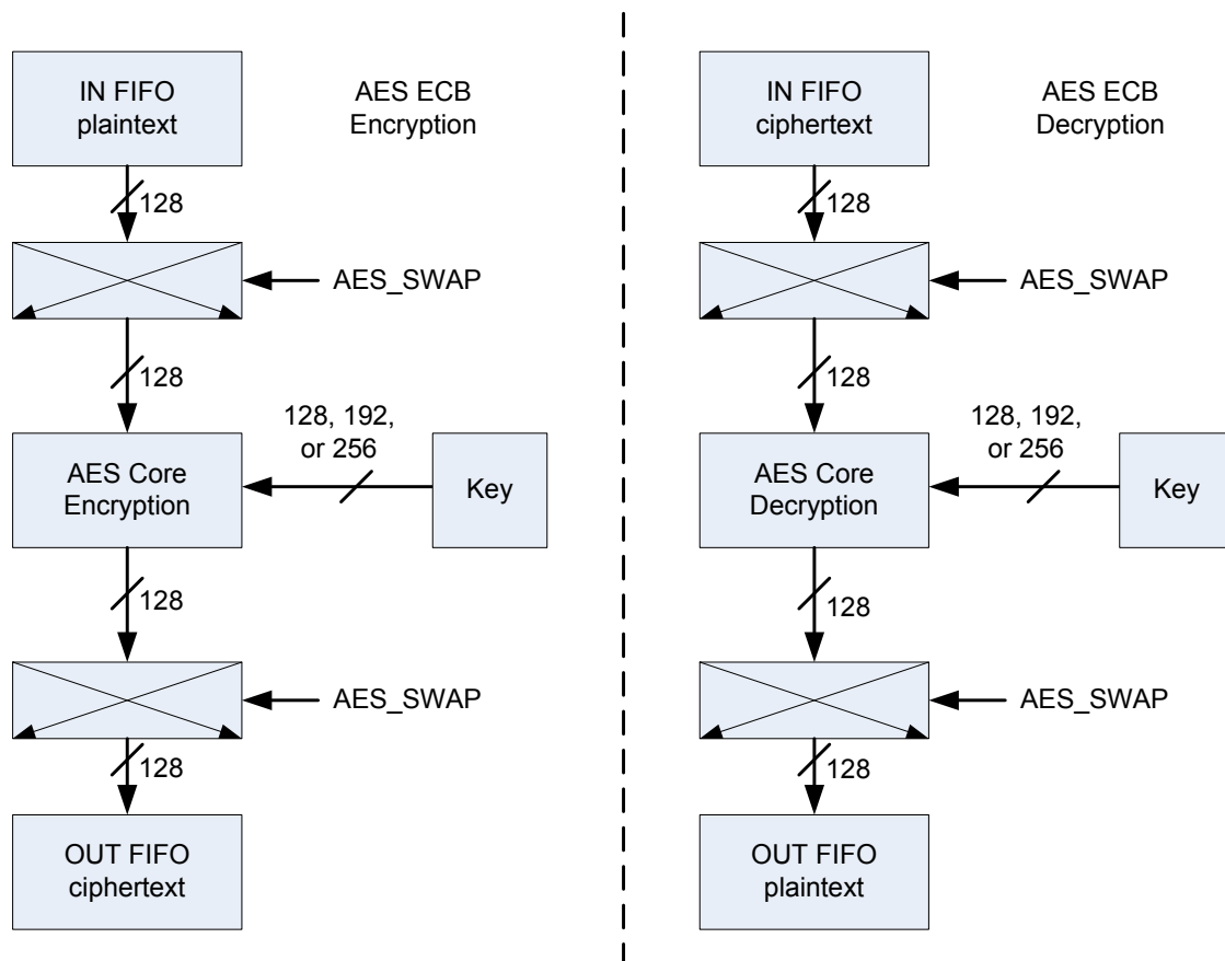
Figure 215. ECB Mode of AES
