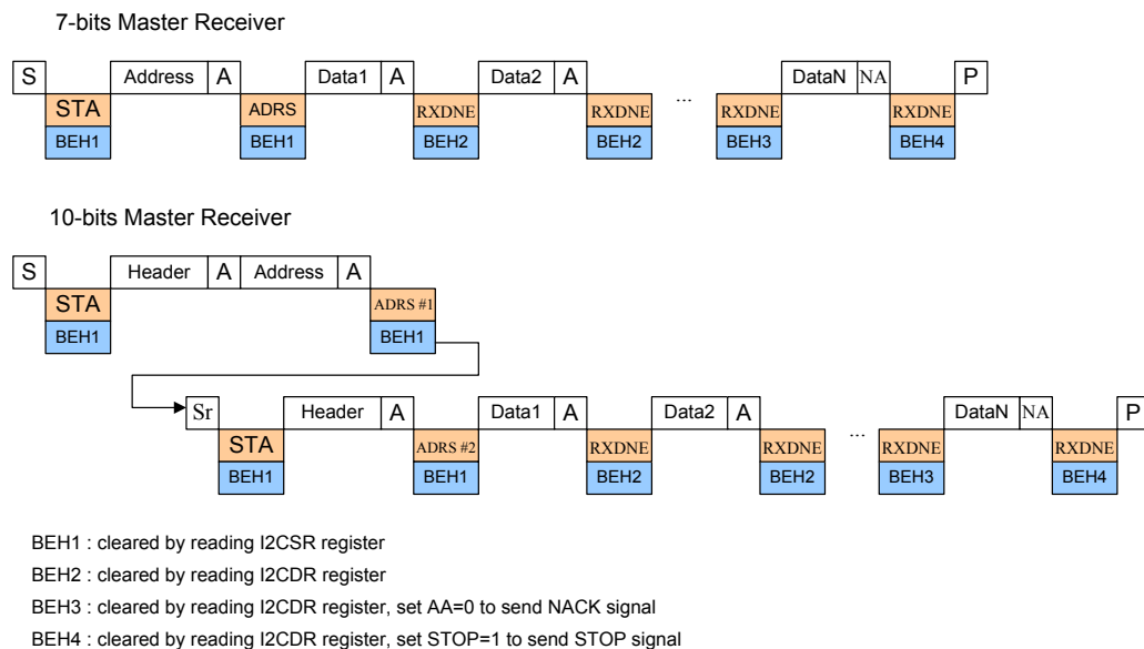
Figure 136. Master Receiver Timing Diagram
