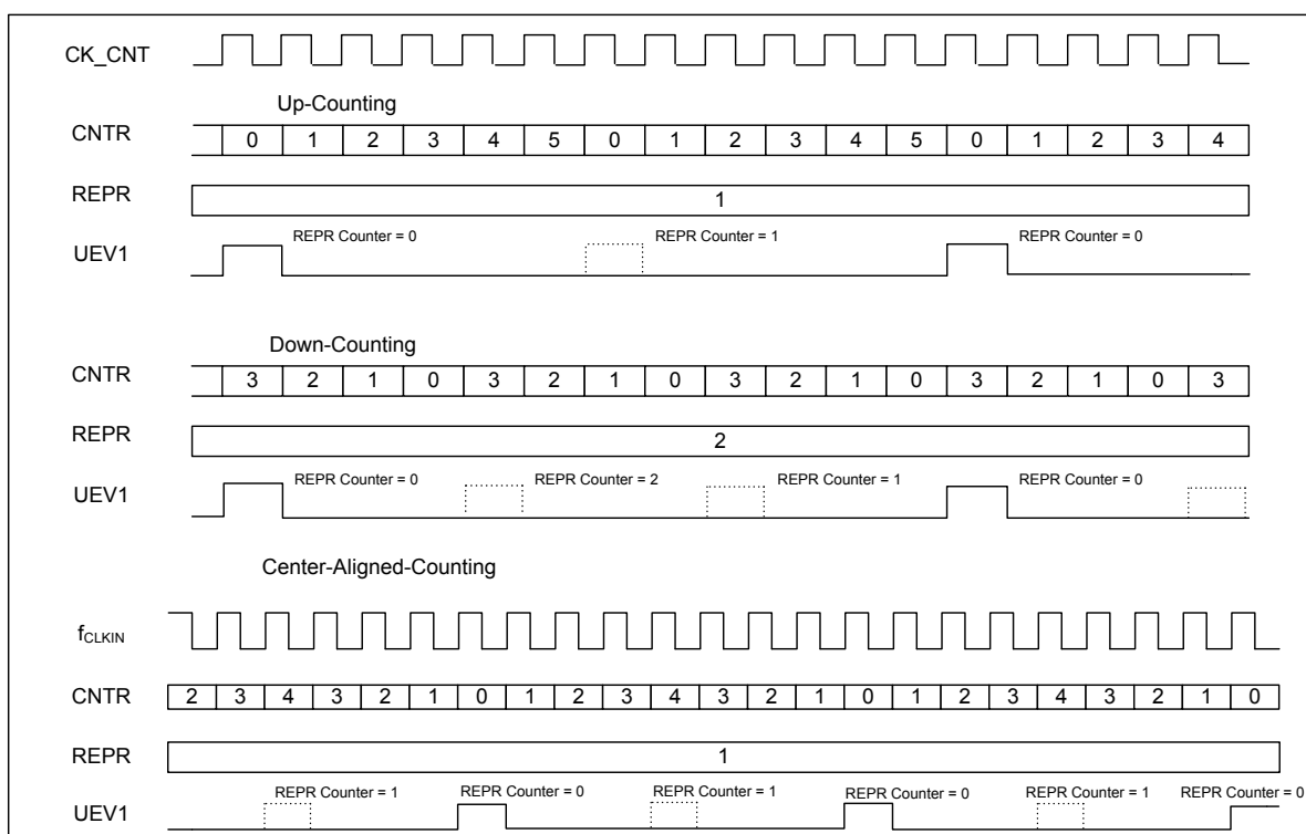
Figure 81. Update Event Dependent Repetition Mechanism Example
