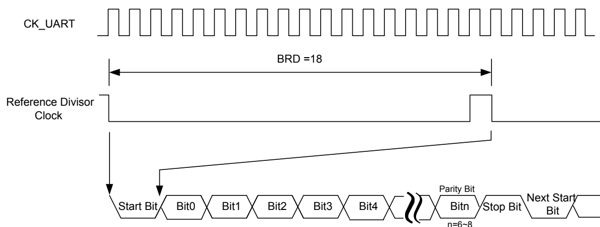
Figure 163. UART Clock CK_UART and Data Frame Timing
