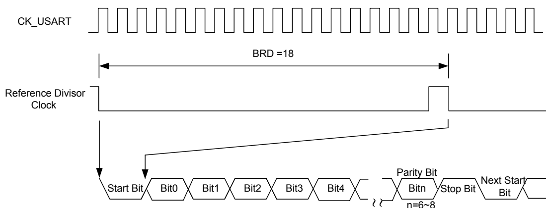
Figure 152. USART Clock CK_USART and Data Frame Timing
