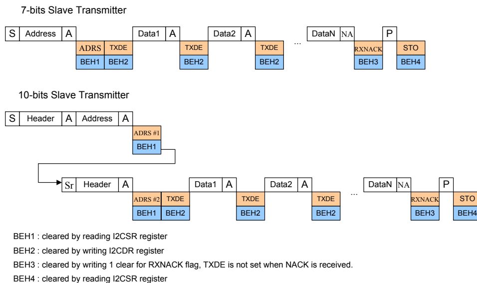
Figure 137. Slave Transmitter Timing Diagram
