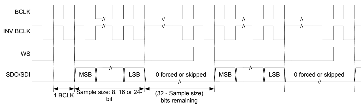
Figure 206. Left-justified Mono Mode Waveforms (32-bit Channel Enabled)
