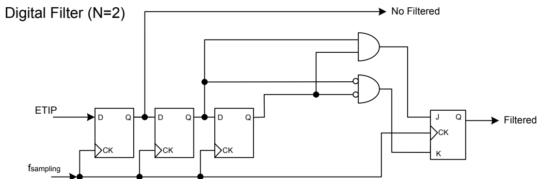
Figure 64. GTn_ETI Pin Digital Filter Diagram with N = 2
