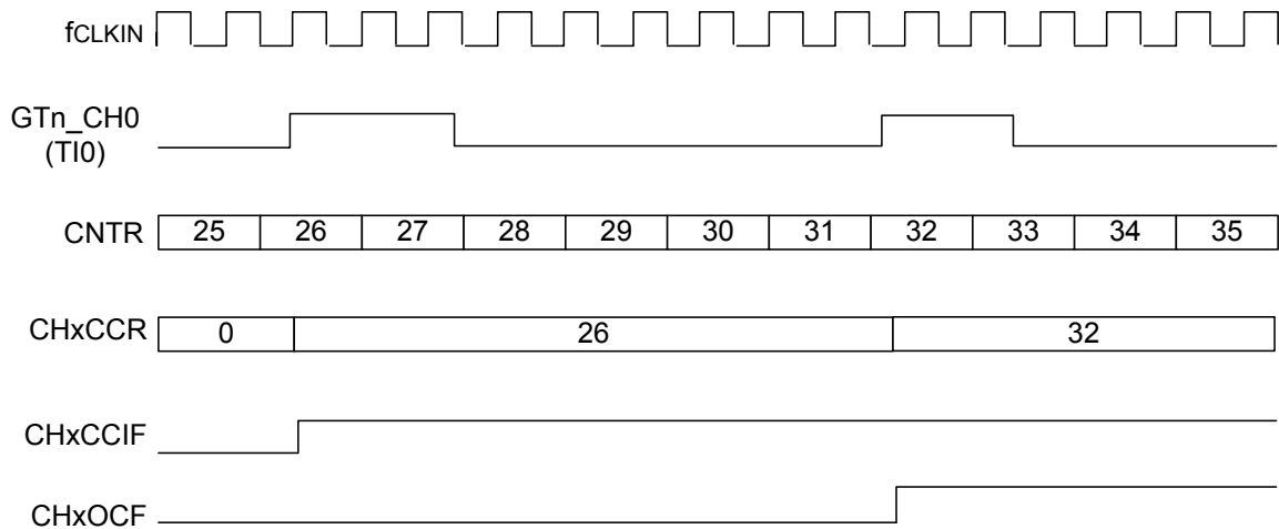
Figure 51. Input Capture Mode
