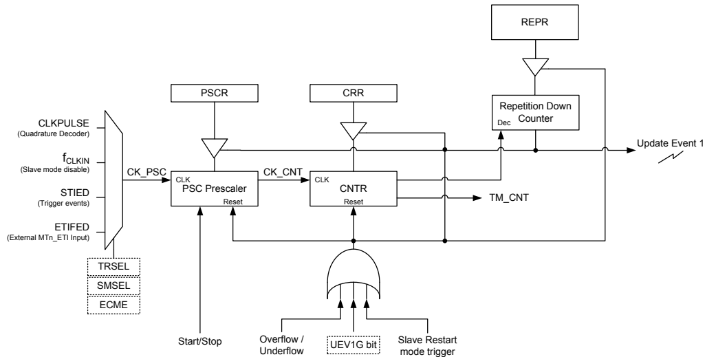
Figure 82. MCTM Clock Selection Source
