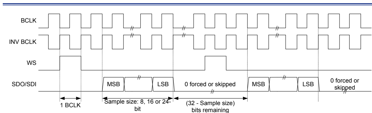
Figure 204. I 2 S-justified Mono Mode Waveforms (32-bit Channel Enabled)
