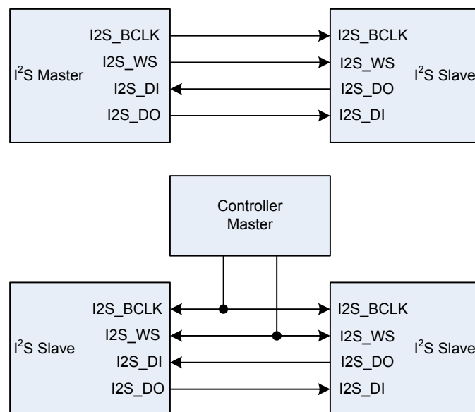
Figure 195. Simple I 2 S Master/Slave Configuration
