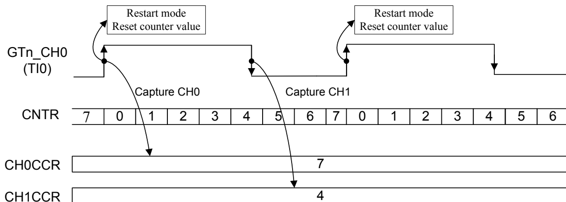
Figure 52. PWM Pulse Width Measurement Example
