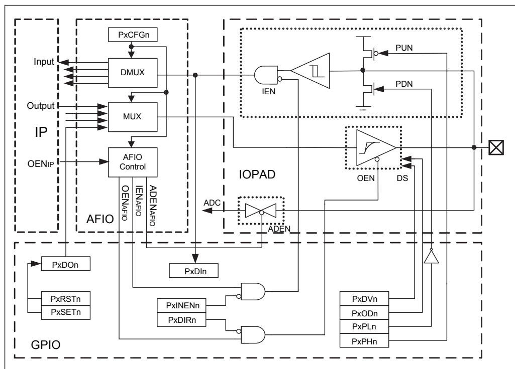
Figure 22. AFIO / GPIO Control Signal
