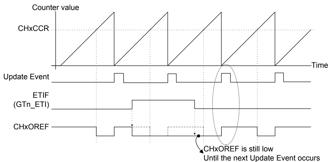
Figure 65. Clearing CHxOREF by ETIF
