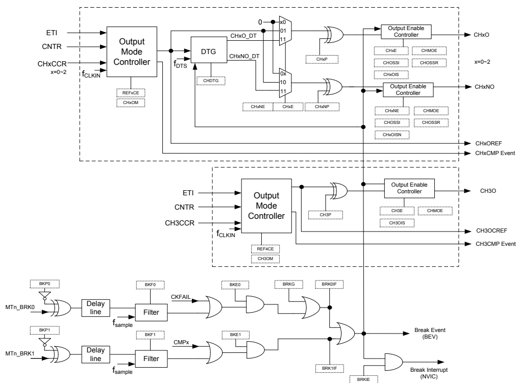
Figure 95. Output Stage Block Diagram
