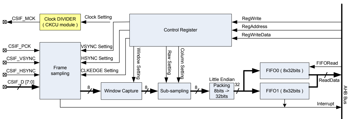
Figure 235. CSIF Block Diagram
