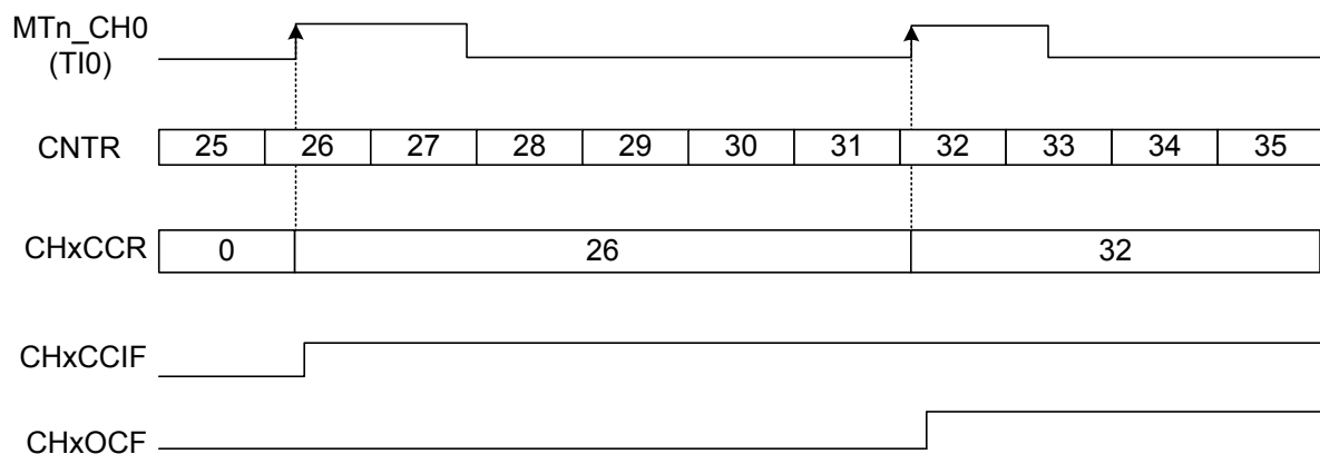
Figure 91. Input Capture Mode
