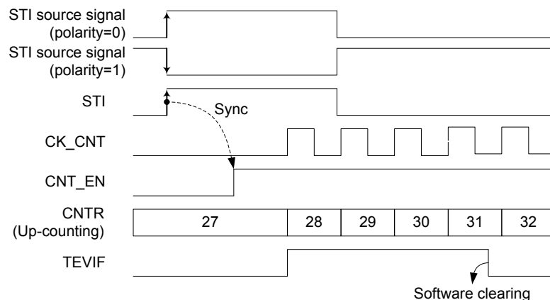
Figure 87. MCTM in Trigger Mode
