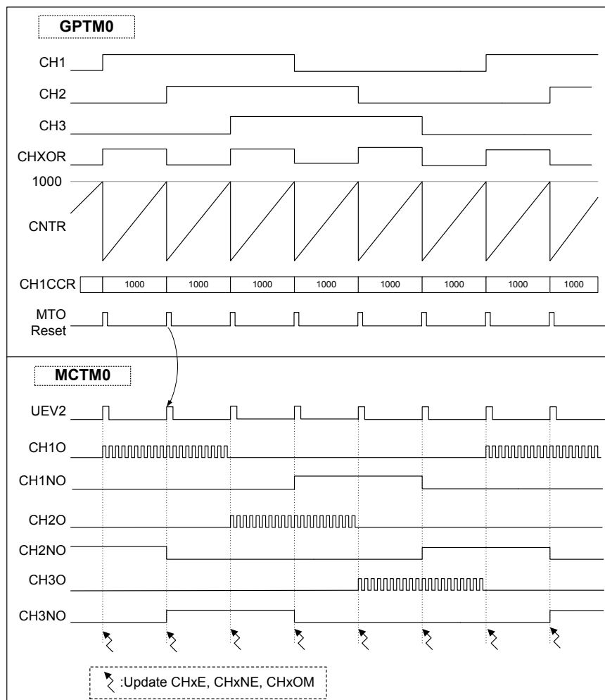
Figure 121. CH1XOR Input as Hall Sensor Interface
