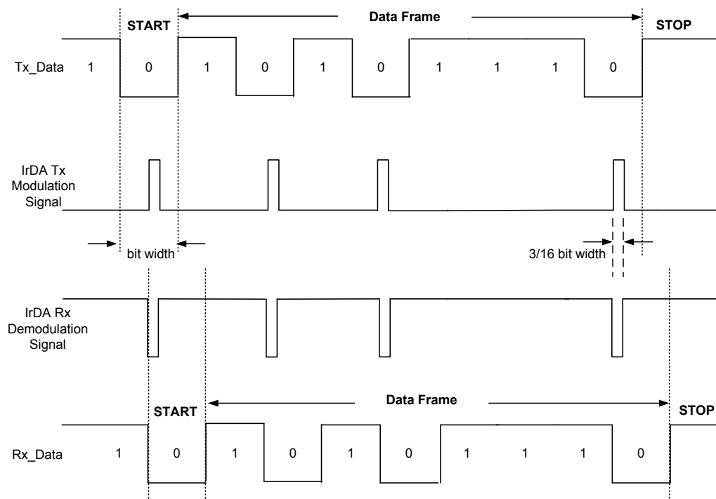
Figure 156. IrDA Modulation and Demodulation
