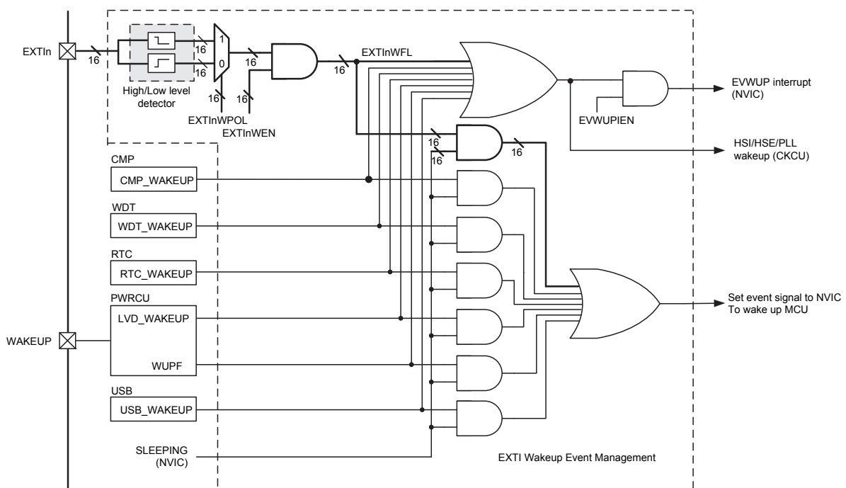
Figure 26. EXTI Wake-up Event Management
