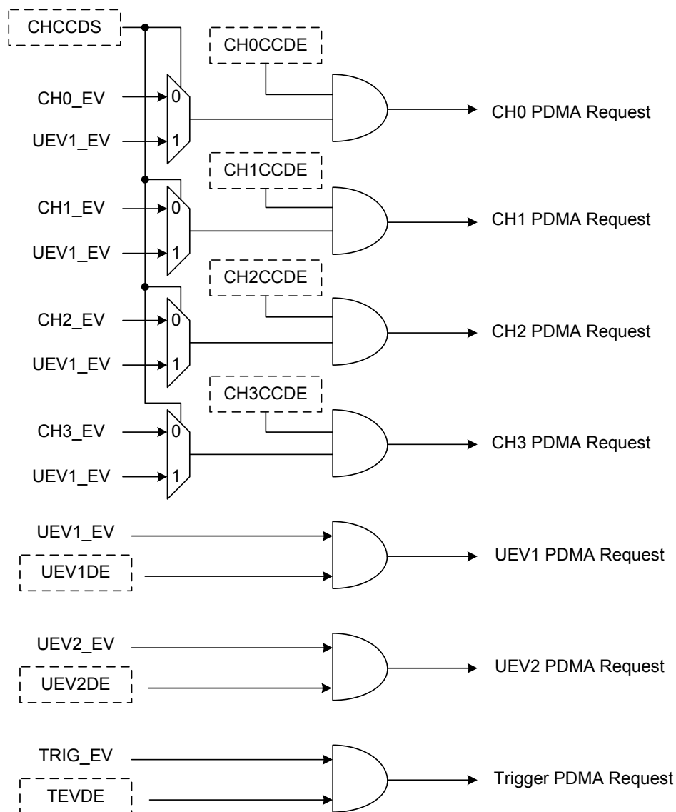
Figure 122. MCTM PDMA Mapping Diagram
