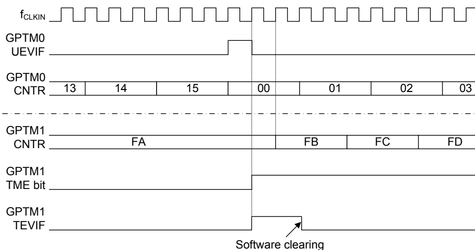
Figure 70. Triggering GPTM1 with GPTM0 Update Event
