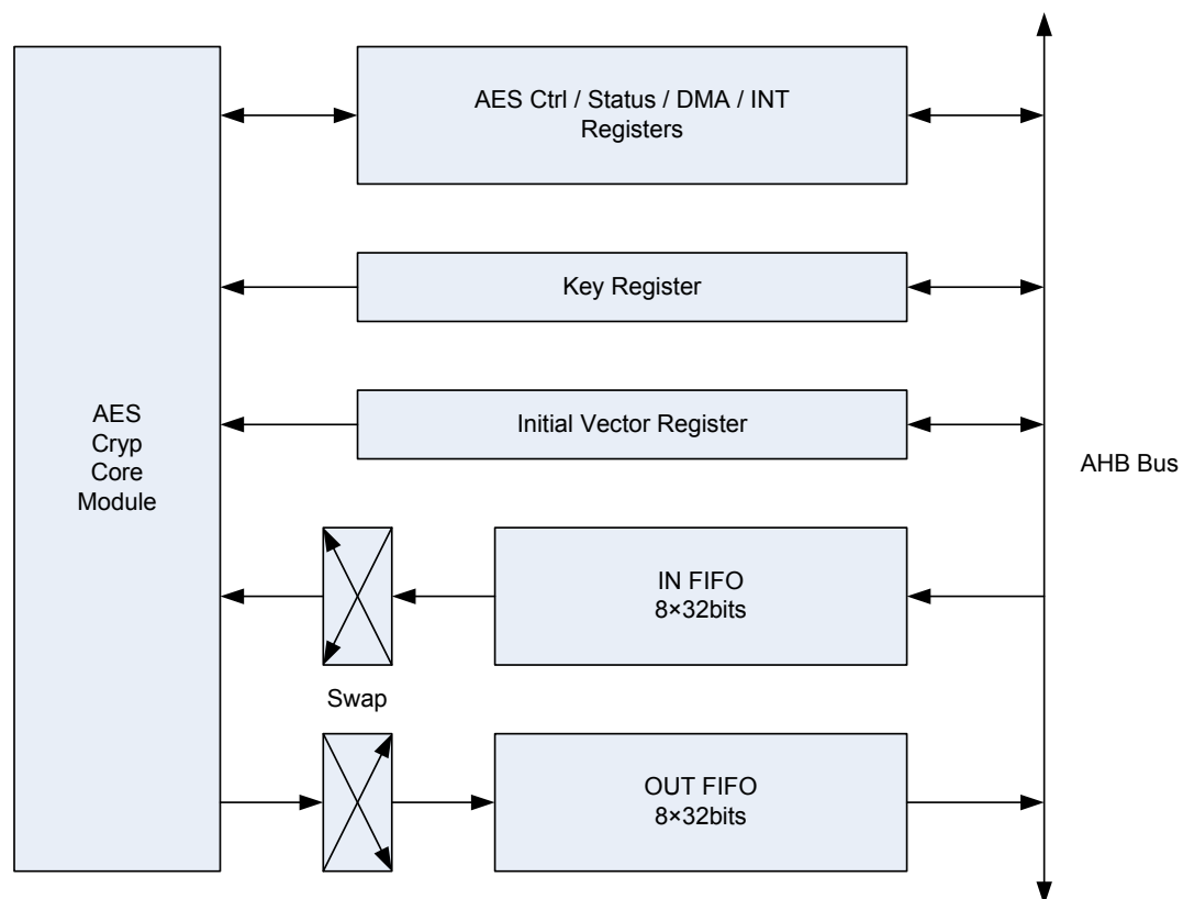
Figure 214. AES Block Diagram
