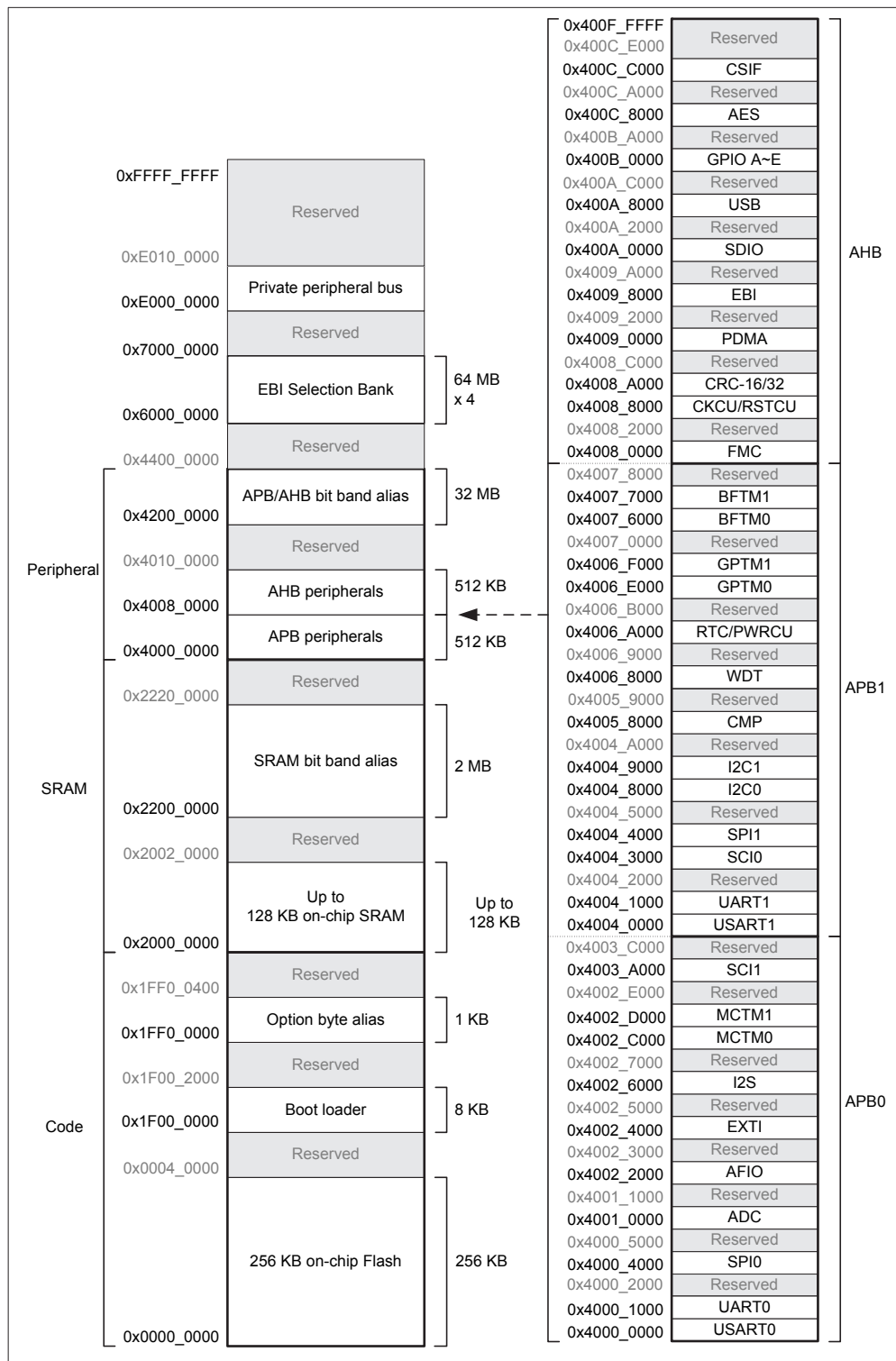
Figure 4. Memory Map
