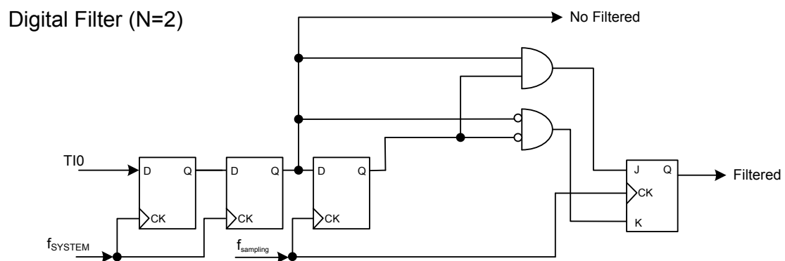
Figure 113. MTn_ETI Pin Digital Filter Diagram with N = 2
