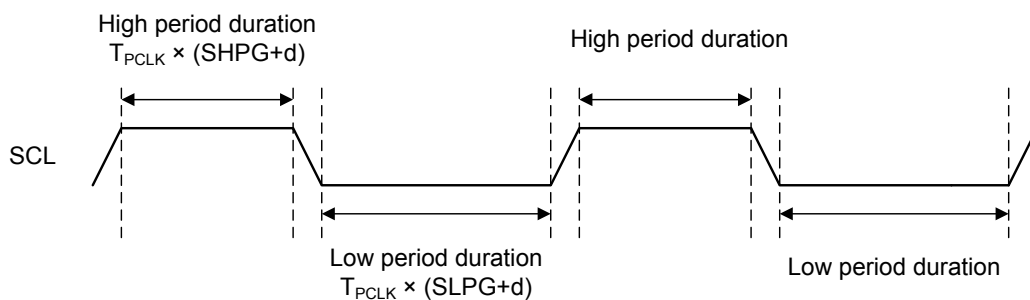
Figure 139. SCL Timing Diagram
