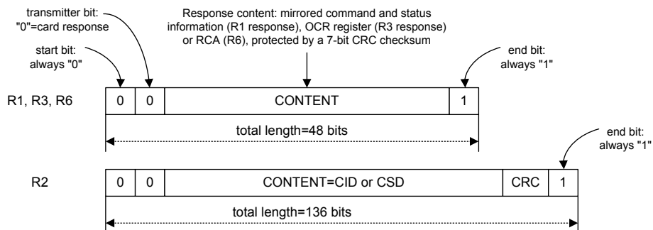
Figure 230. Response Format
