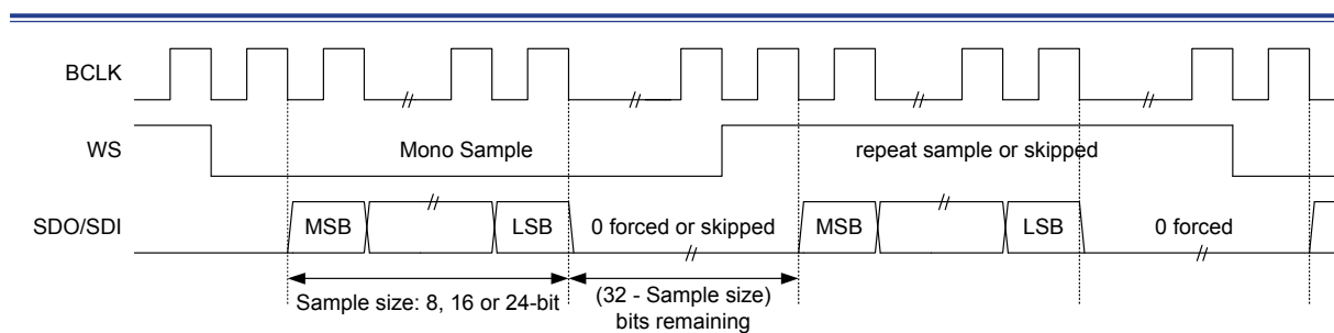
Figure 210. I 2 S-justified Repeat Mode Waveforms (32-bit Channel Enabled)
