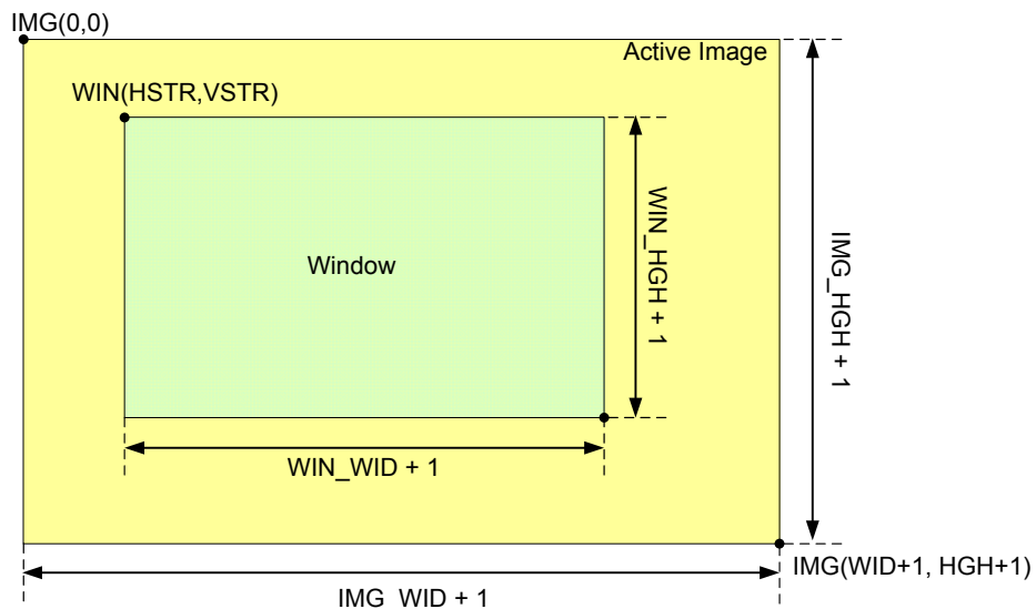
Figure 239. Proper Window Capture
