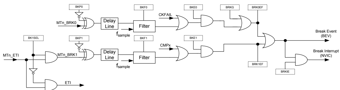
Figure 102. MCTM Break Signal Block Diagram
