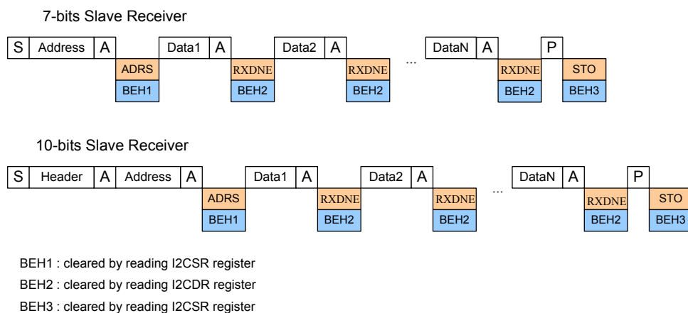
Figure 138. Slave Receiver Timing Diagram
