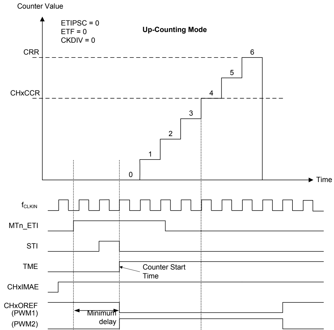
Figure 116. Immediate Active Mode Minimum Delay
