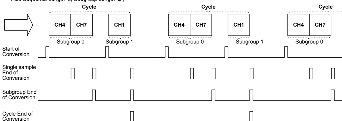
Figure 32. High Priority Group Discontinuous Conversion Mode
