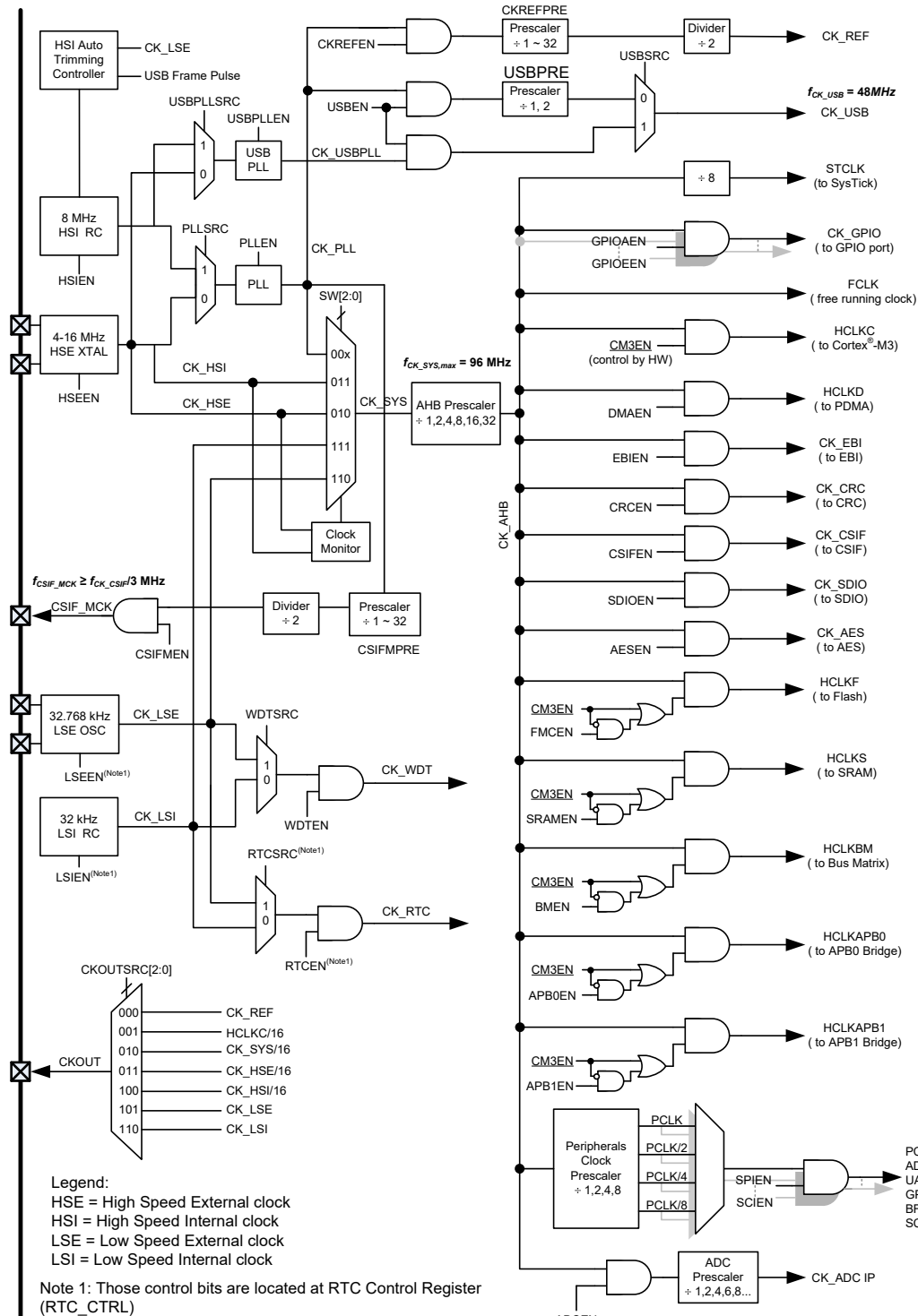
Figure 13. CKCU Block Diagram
