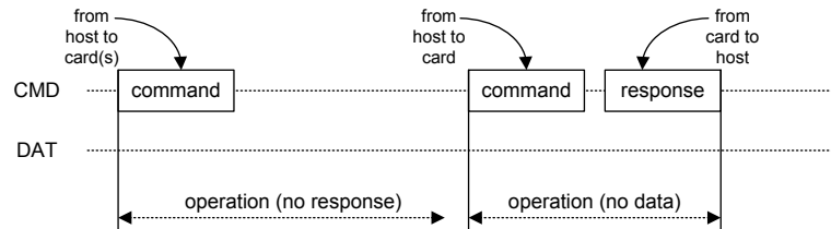
Figure 226. "No Response" and "No Data" Operations
