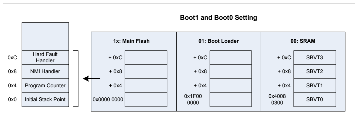
Figure 7. Vector Remapping
