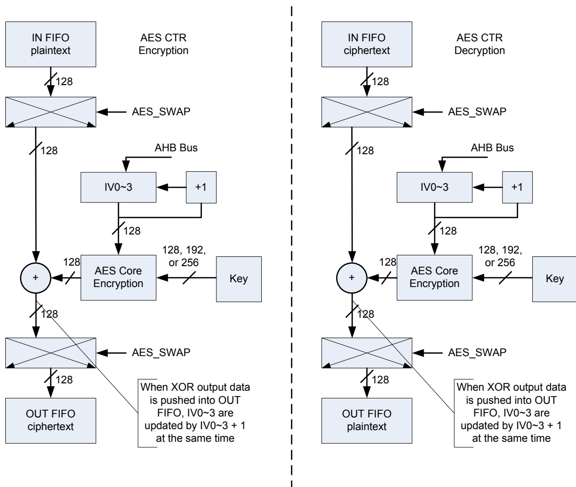
Figure 217. CTR Mode of AES
