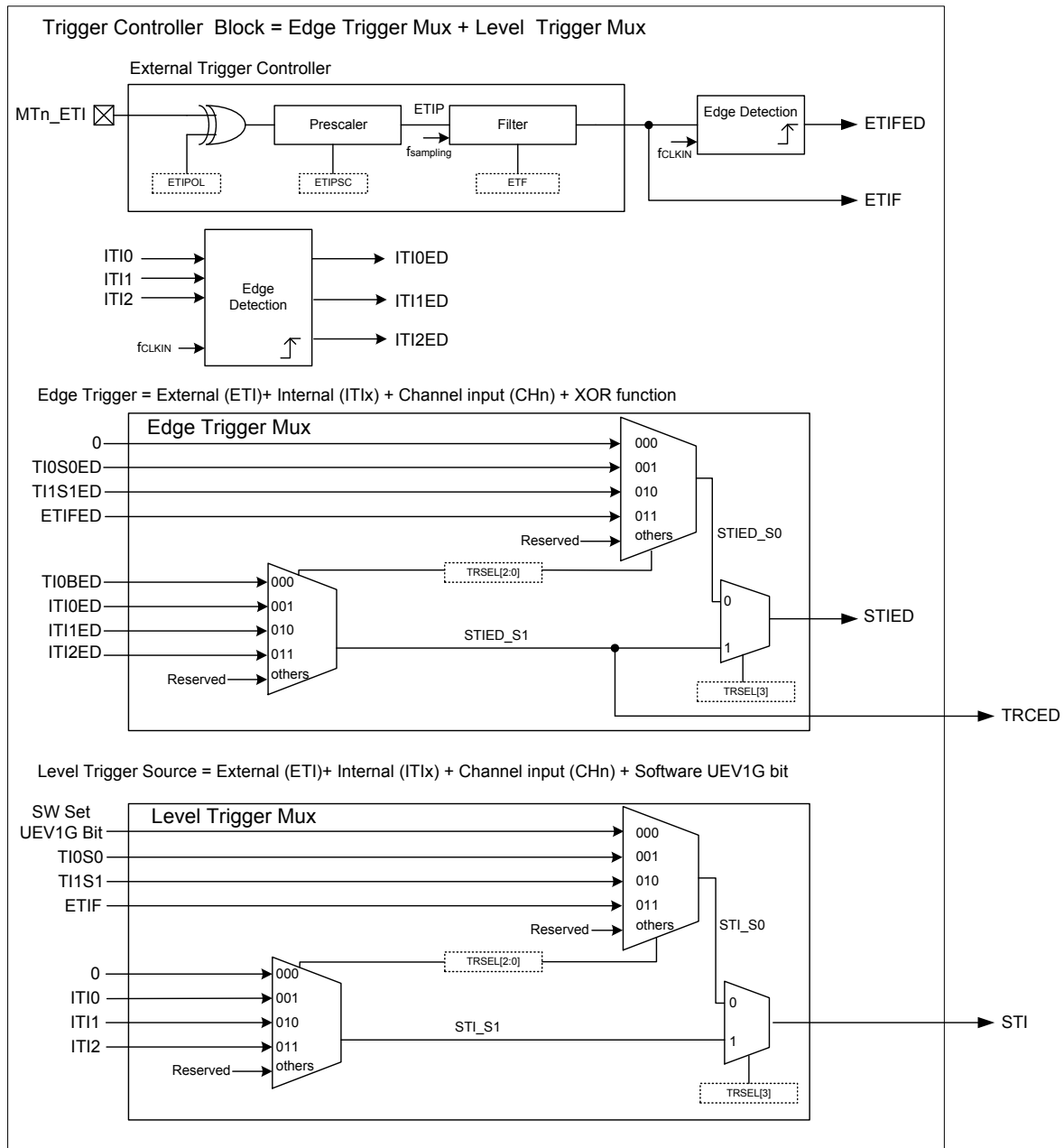
Figure 83. Trigger Control Block
