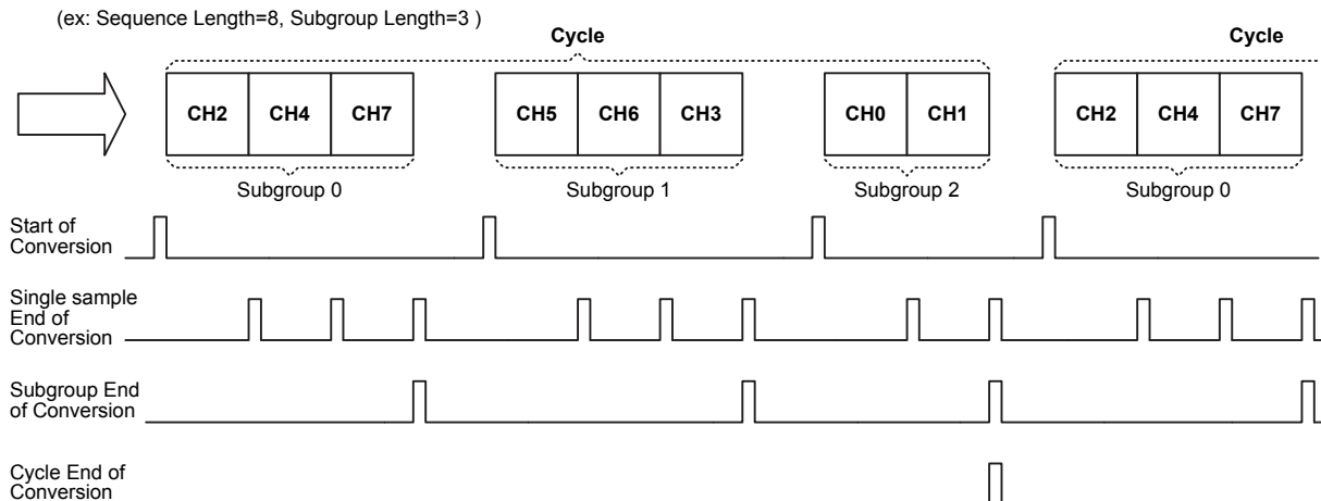
Figure 31. Regular Group Discontinuous Conversion Mode
