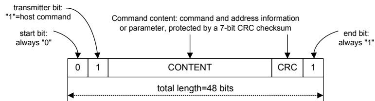
Figure 229. Command Format
