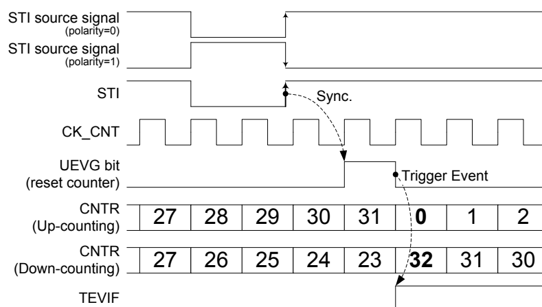
Figure 45. GPTM in Restart Mode
