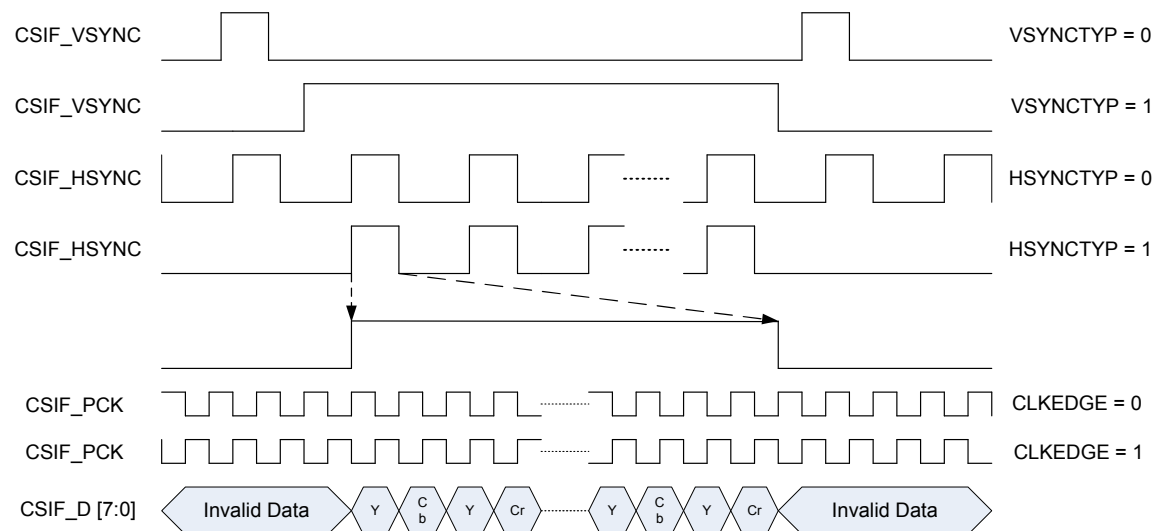
Figure 237. CSIF Frame Timing
