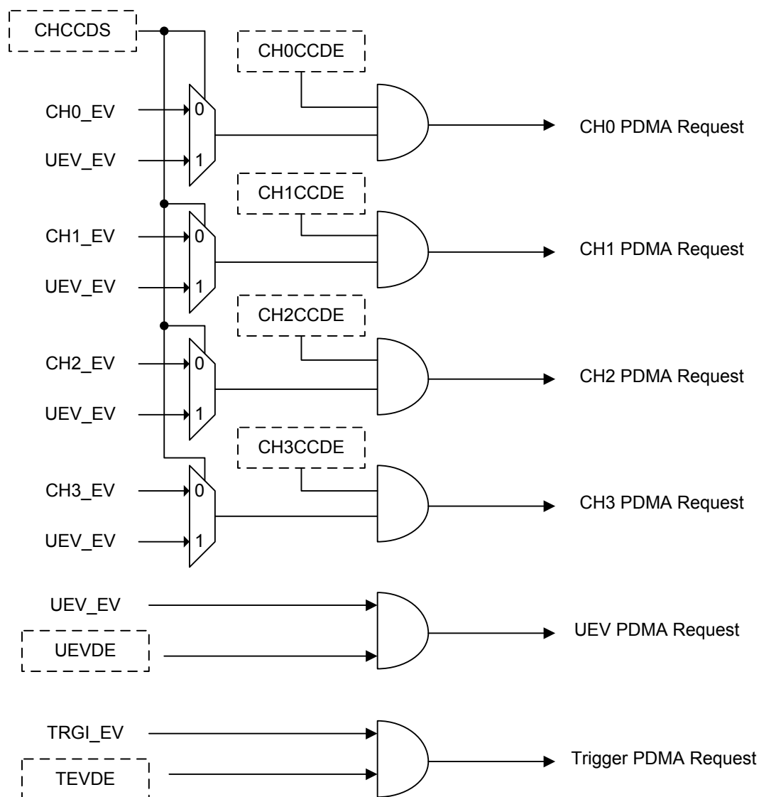
Figure 72. GPTM PDMA Mapping Diagram
