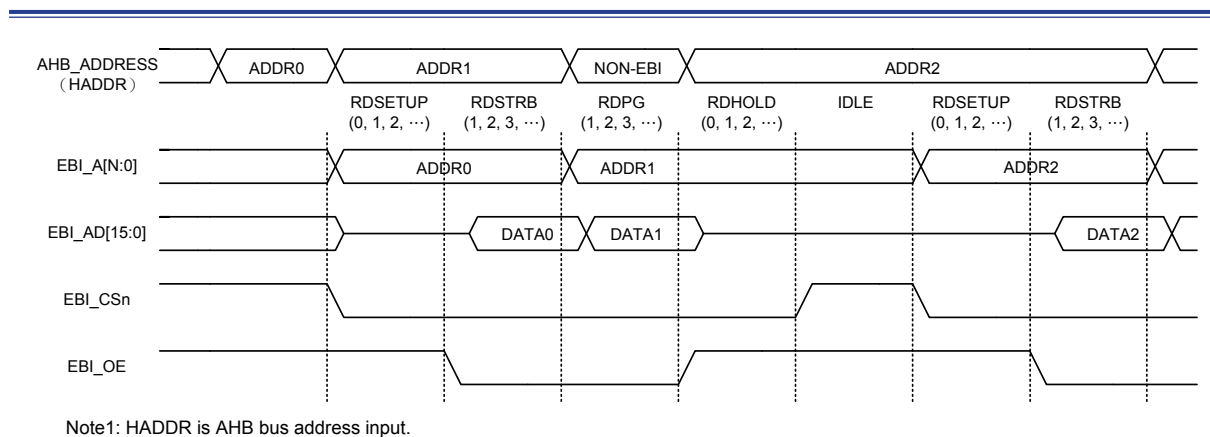
Figure 190. EBI Page Close Example
