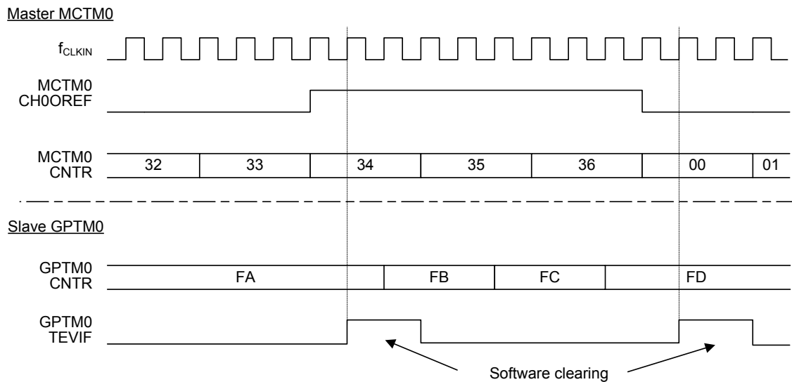
Figure 118. Pausing GPTM0 Using the MCTM0 CH0OREF Signal
