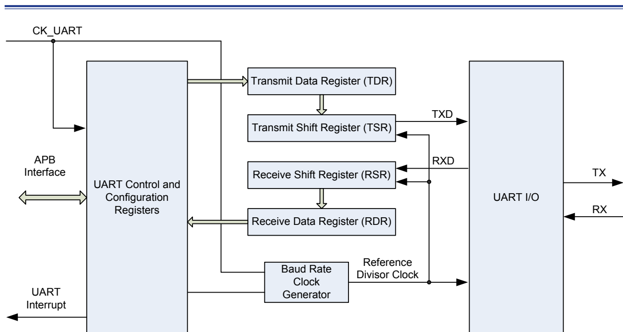
Figure 161. UART Block Diagram
