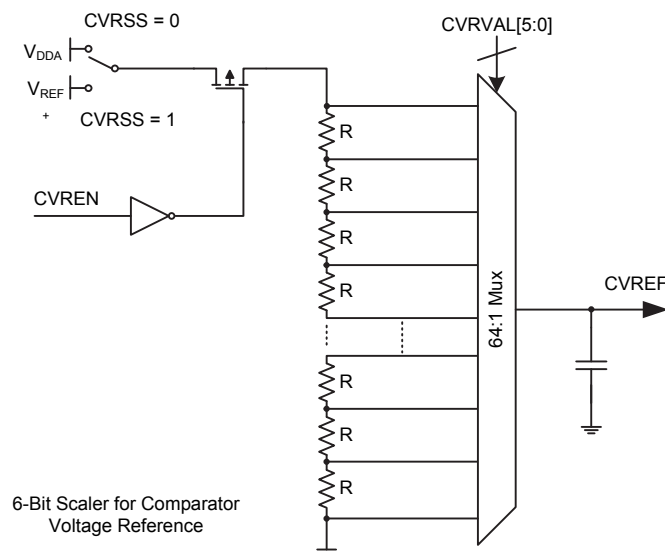
Figure 35. 6-Bit Scaler for Comparator Voltage Reference Block Diagram
