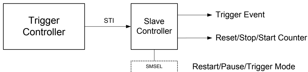
Figure 44. Slave Controller Diagram
