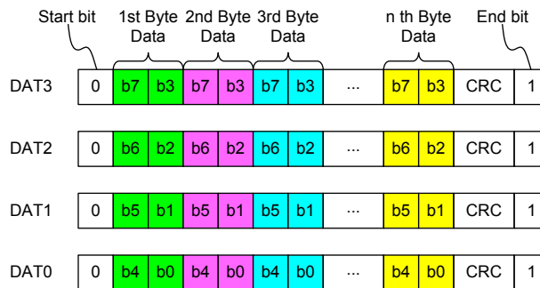
Figure 232. Usual Data Format for Wide Bus – DAT0~DAT3 used
