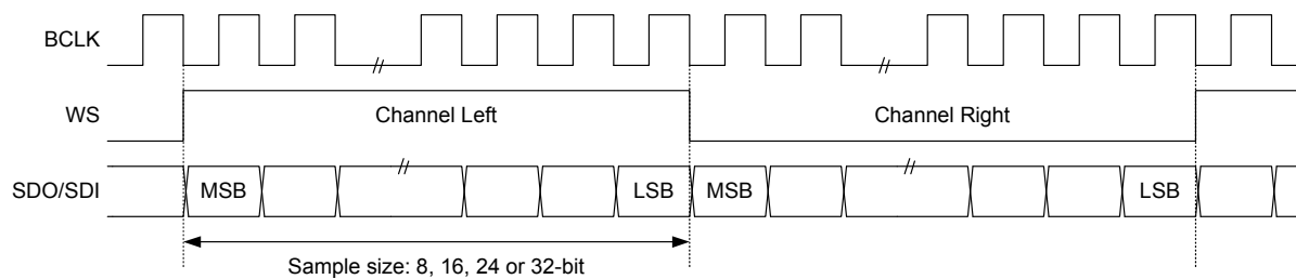
Figure 201. Right-justified Stereo Mode Waveforms
