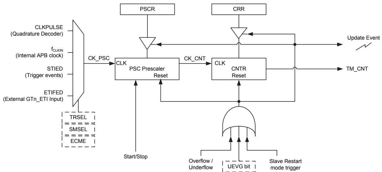
Figure 42. GPTM Clock Selection Source
