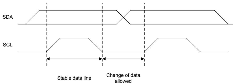
Figure 128. Data Validity
