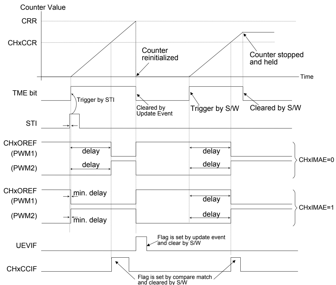
Figure 66. Single Pulse Mode
