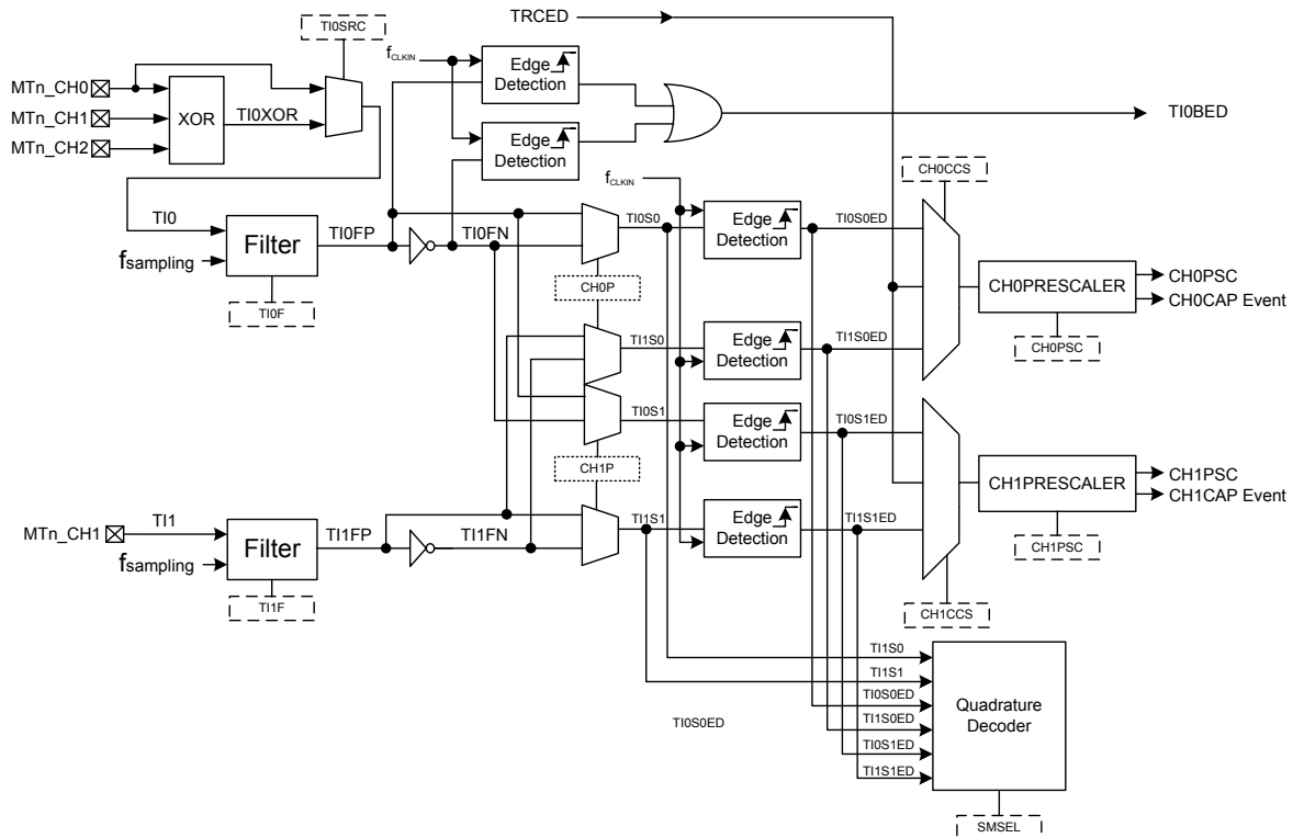
Figure 111. Input Stage and Quadrature Decoder Block Diagram
