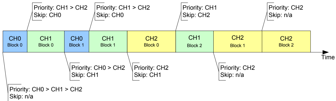
Figure 175. PDMA Channel Arbitration and Scheduling Example
