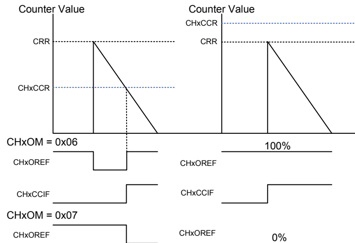
Figure 99. PWM Mode Channel Output Reference Signal and Counter in Down-counting Mode
