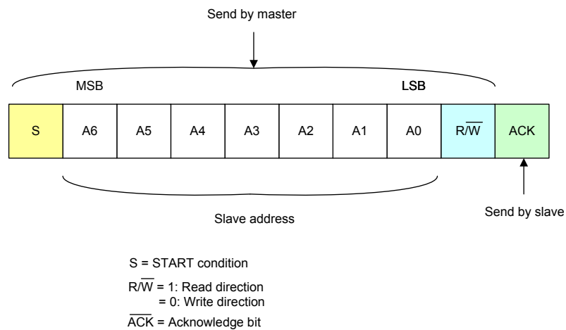
Figure 129. 7-bit Addressing Mode
