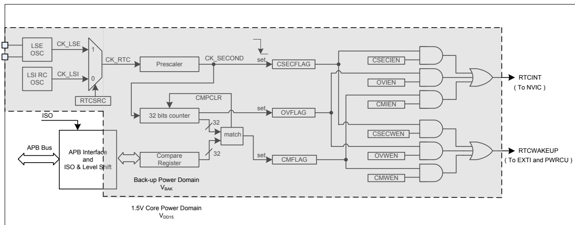
Figure 123. RTC Block Diagram
