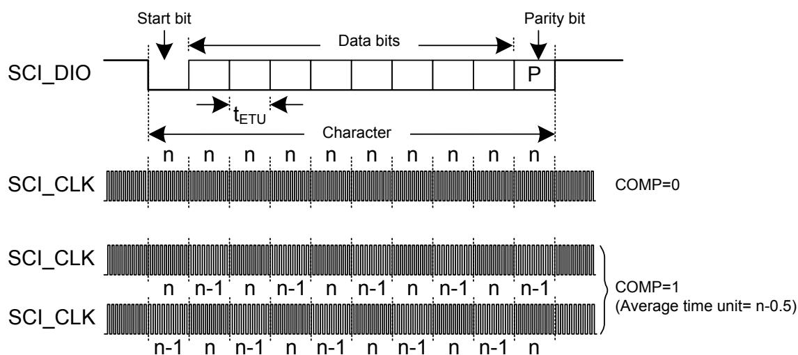
Figure 165. Character Frame and Compensation Mode
