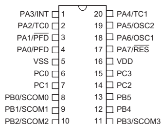
HT48R066 20 DIP-A/SOP-A/SSOP-A
