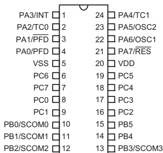
HT48R066 24 SKDIP-A/SOP-A/SSOP-A
