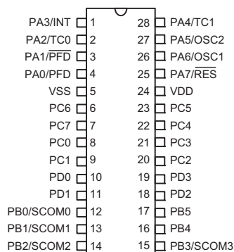
HT48R066 28 SKDIP-A/SOP-A/SSOP-A
