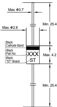
Glass Case DO-41 Dimensions in mm
