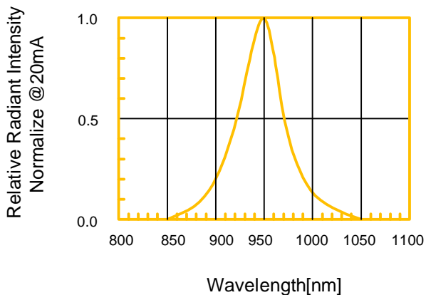
Fig.2 Relative Radiant Intensity vs. wavelength
