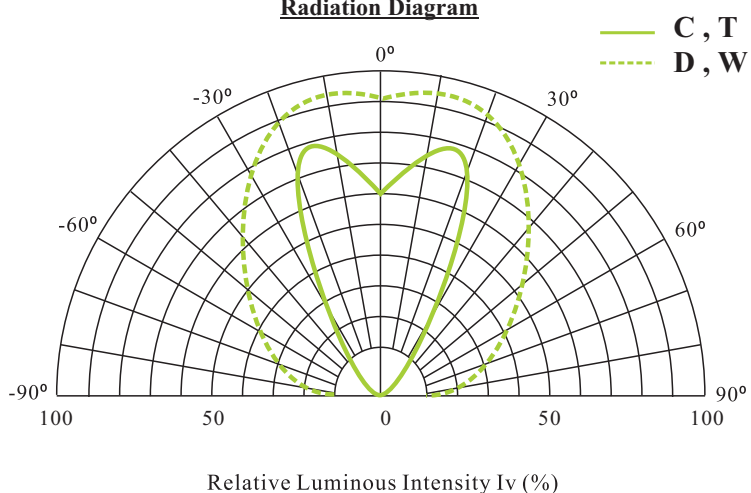
Radiation Diagram
