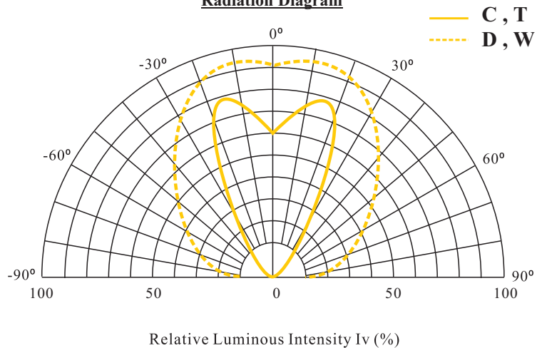
Radiation Diagram
