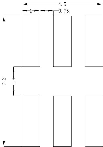
For reflow soldering 建议焊盘尺寸
