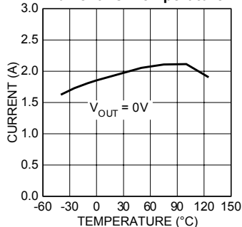
MIC29150-3.3 Short Circuit Current vs. Temperature
