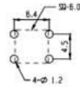
PCB LAYOUT
